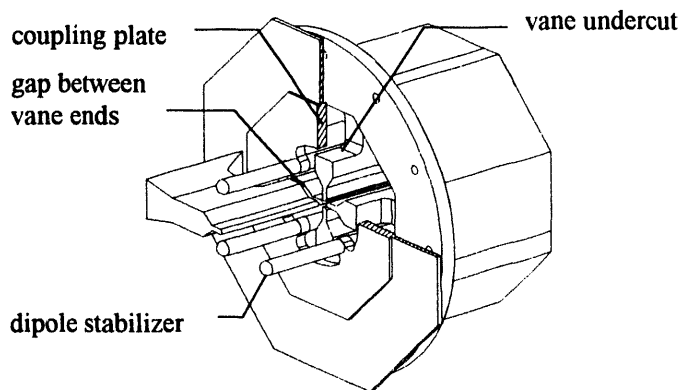
Figure 1 Cutaway drawing of the coupling plate between segments of the RFQ.
