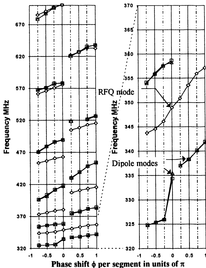
Figure 2 Dispersion curve of modes in resonant coupled RFQ. Note, chart on right has expanded scale. The diamonds indicate quadrupole modes while the squares and triangles indicate dipole modes.
