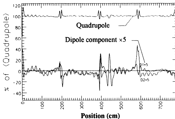
Figure 3 Bead-perturbation measurement of the 8-m-long coupled RFQ. The dipole components of the fields are shown multiplied by a factor of 5.
