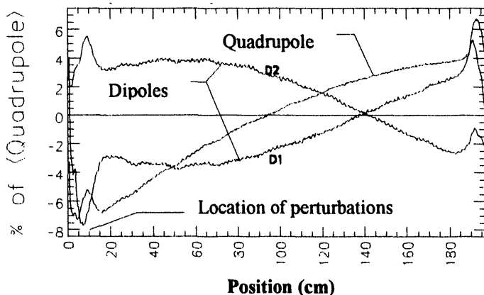
Figure 5 Difference between two bead-perturbation measurements in a 2-m long RFQ showing the change in the fields caused by two 90 kHz perturbations, one each in quadrants 2 and 3.
