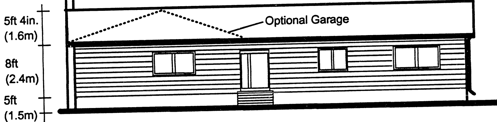
Fig 2. Floor plan and elevation of 1-story ranch house.
