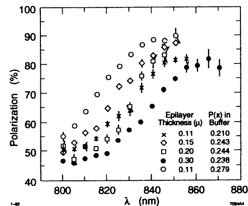
Fig. 5. Polarization can be enhanced by varying the thickness of the surface epilayer and the phosphorus concentration of the sublayer. Shown here are measurements made in GaAs materials with these parameters varied. E143 has been operating with a 0.1\mu and 28% phosphorus concentration, giving an average polarization of 85%.
