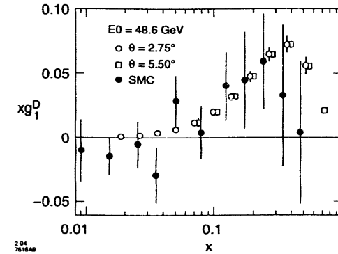
Fig. 9. The expected statistical errors on xg_1^d(x) from the 50 GeV experiment E155 proposal is compared to existing SMC data (ref. 8).
