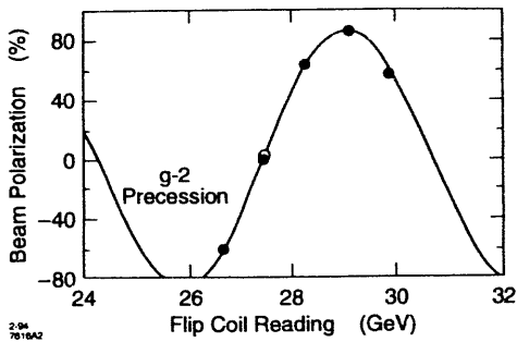
Fig. 2. Calibration of the energy of the beam line in E143 was possible using the precession of spin. The longitudinal component is measured with a Møller polarimeter in the End Station A. The data are shown plotted versus the flipcoil measurement of energy in the reference magnet, and the curve shows the expected g-2 precession. The accuracy of the energy calibration is approximately \pm 0.1\% by this method.
