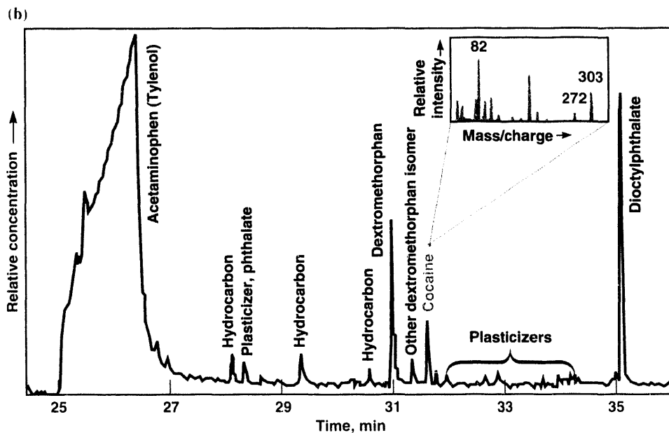
Figure 1. (a) Our portable gas chromatograph/mass spectrometer (GC/MS) can be used to analyze any liquid, solid, or gas chemical sample in the field. Results from a typical GC/MS analysis (b) show the separation of compounds in the sample. Shown here is a sample of confiscated cocaine, which had been adulterated with Tylenol and other compounds. Identification of the various compounds is achieved through analysis of the ion fragmentation patterns of some 2000 individual mass spectra. The inset graph is one such mass spectral fragmentation pattern, which reveals enough structural information to identify the compound as cocaine.
