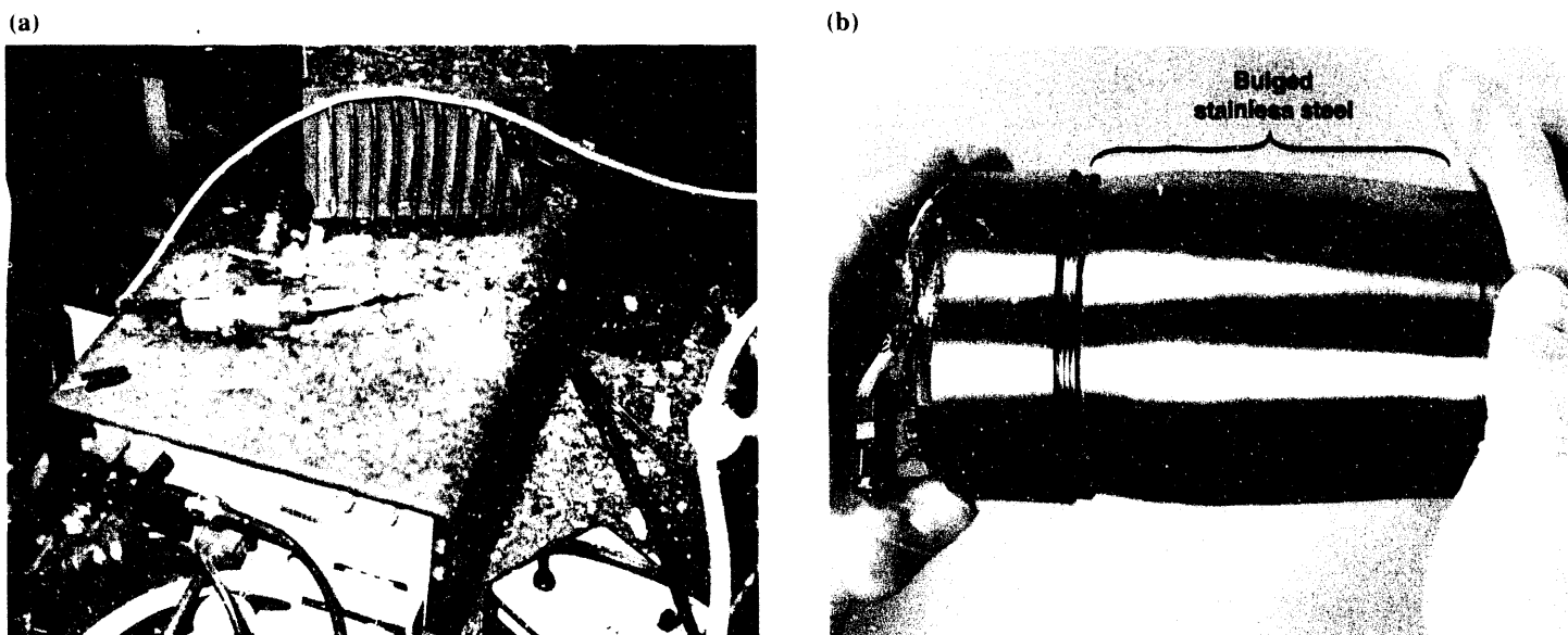
Figure 5. In 1992, an explosion occurred during a "cold-fusion" experiment at a research laboratory in California. About 65 LLNL scientists were called upon to analyze the debris (a) to shed light on potential causes of the explosion. The distended cold-fusion cell after the explosion is shown in (b). Our most unanticipated result was that machine-shop lubricating oil could have been a potential contributor to the incident. 1
