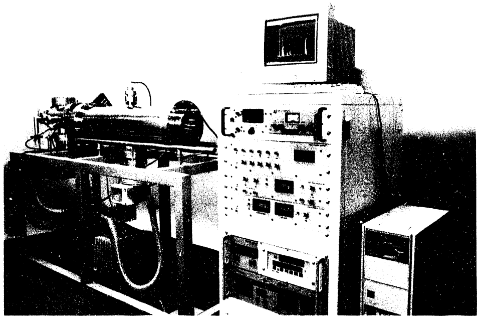
Figure 3. Our laboratory-size ion-storage trap/time-of-flight (IT/TOF) instrument. We are currently designing a smaller transportable instrument.
