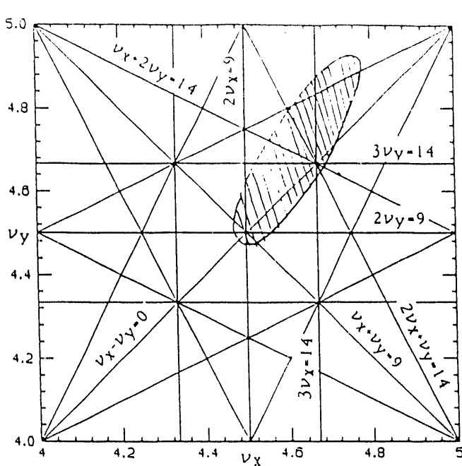
Fig. 1 Tune diagram of the AGS Booster.
