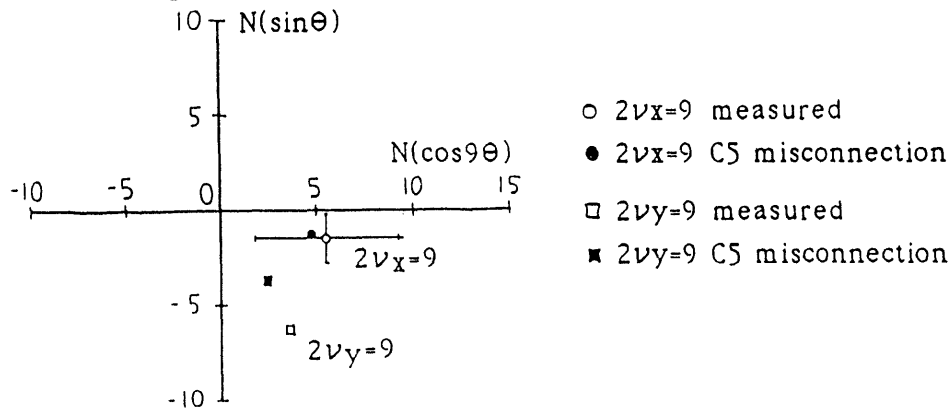
Fig. 5 Eddy-current terms of normal quadrupole imperfection.
