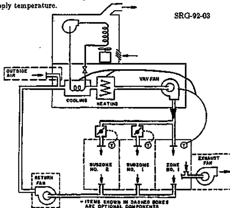
Figure 3.5: Packaged variable temperature, variable volume system (PVVT).
