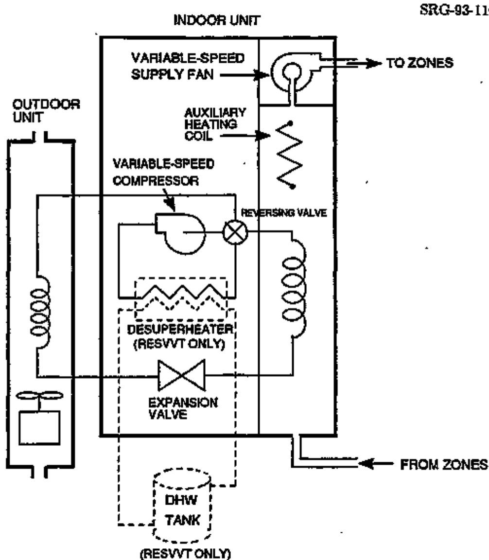
Figure 3.8: System configuration for a variable speed electric heat pump.
