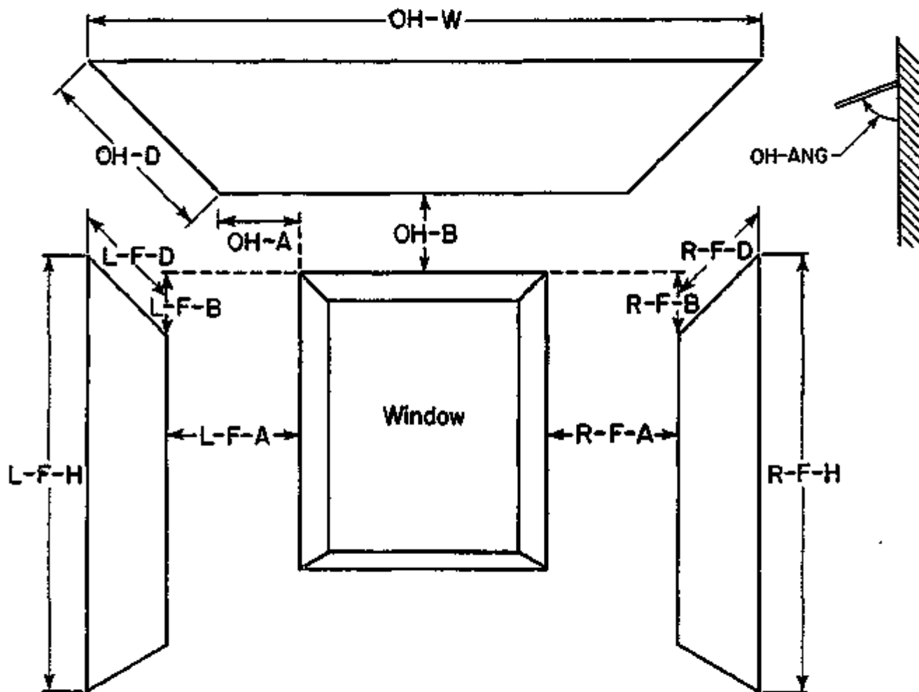
Figure 2.17 Positioning of overhang and fins with respect to a window. The values in this figure are all positive. If the value for L-F-B is input as negative, then the left fin will originate at a point above the top edge of the window, and similarly for R-F-B .
