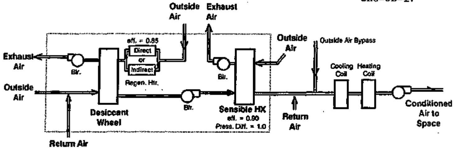
Figure 3.20: Mode 2 — Solid desiccant unit with dehumidifier and heat exchanger, without regeneration preheat, shown integrated with a sensible cooling system.
