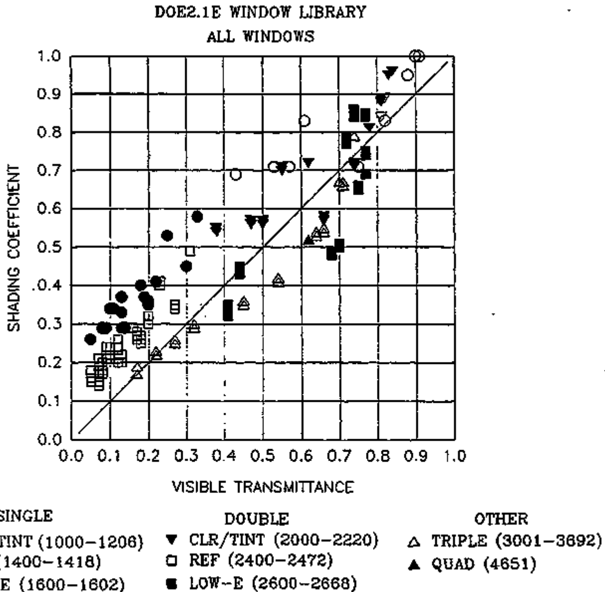
Figure 2.21: Center-of-glass shading coefficient (ASHRAE summer conditions) vs. visible transmittance for all glazings in the Window Library except the electrochromic glazings. The values shown correspond to SC and T_{vis} , respectively, in the Index to the Window Library, Table 2.12. CLR/TINT is clear or tinted glass. REF is glass with a reflective coating. LOW-E is glass with a low-emissivity coating. SINGLE, DOUBLE, TRIPLE and QUAD refer to the number of panes. Numbers in parentheses give the G-T-C range from Table 2.12.
