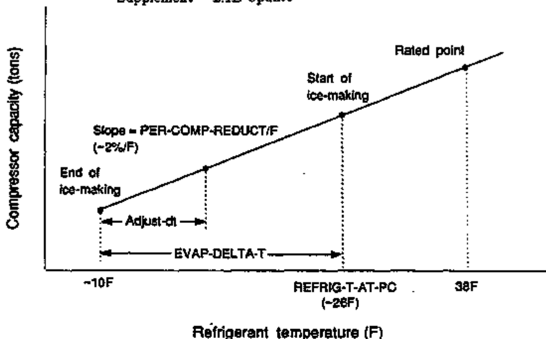
Figure 4.1: Compressor capacity vs. refrigerant temperature for ice making.
