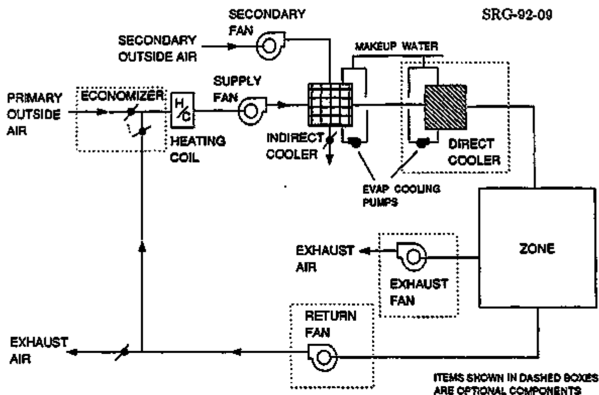
Figure 3.11: Stand-alone evaporative cooler system (SYSTEM-TYPE = EVAP-COOL).
