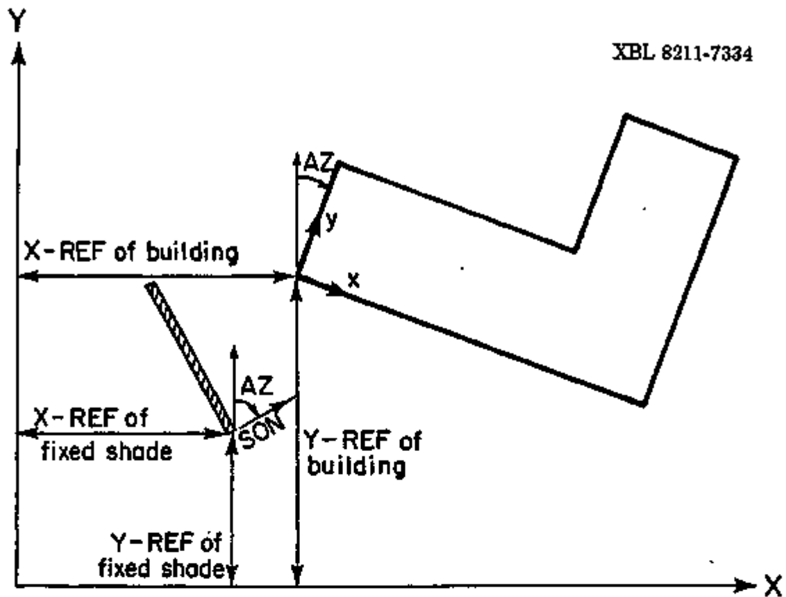
Figure 2.15 Reference Coordinate System. X-REF and Y-REF are the coordinates of the lower left-hand corner of a fixed shade.
