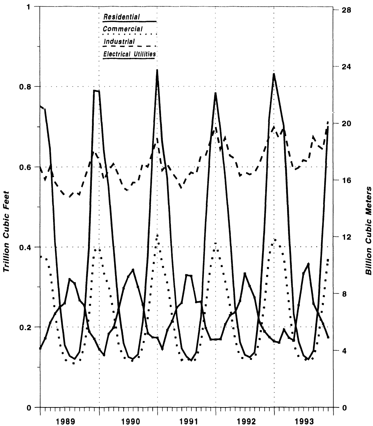
Figure 16. Natural Gas Deliveries to Consumers in the United States, 1989 - 1993
