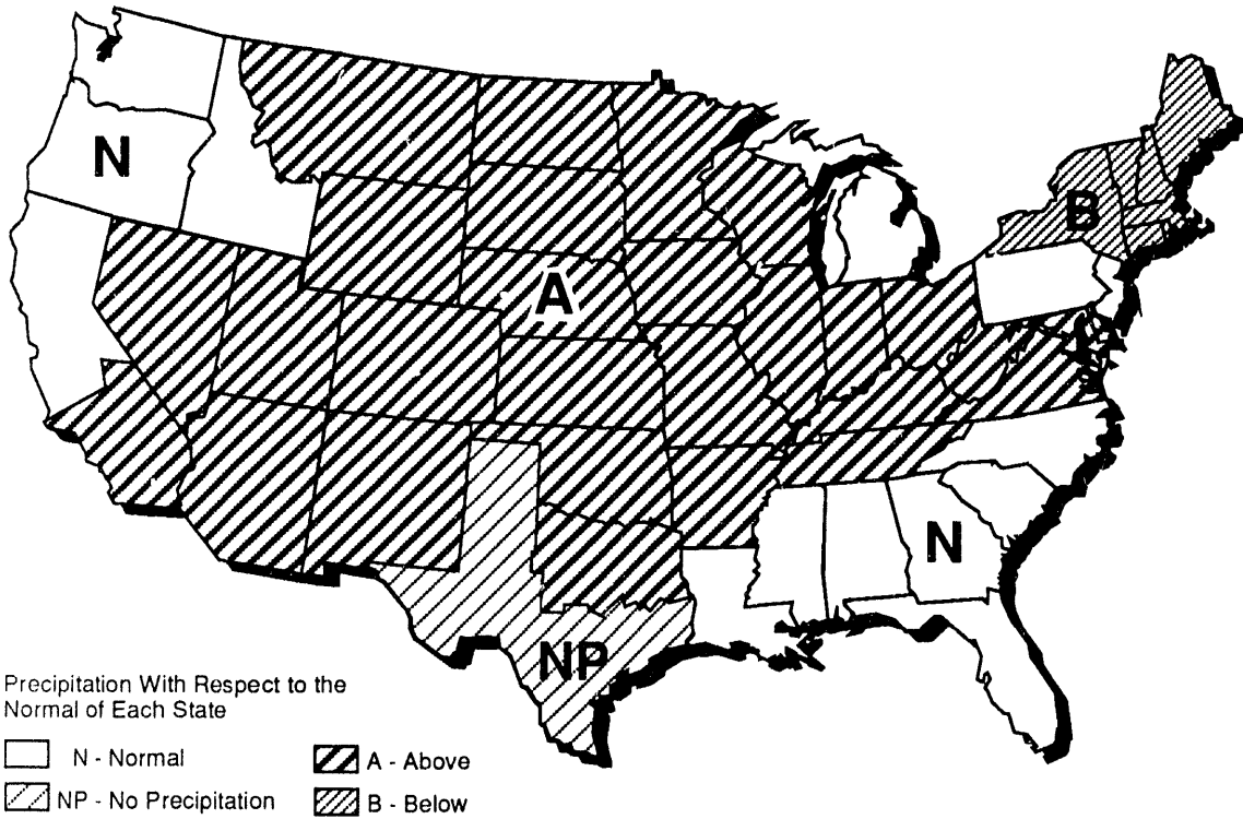
Figure 35. 6 - 10 Day Precipitation Outlook or March 22 Through March 26, 1994
