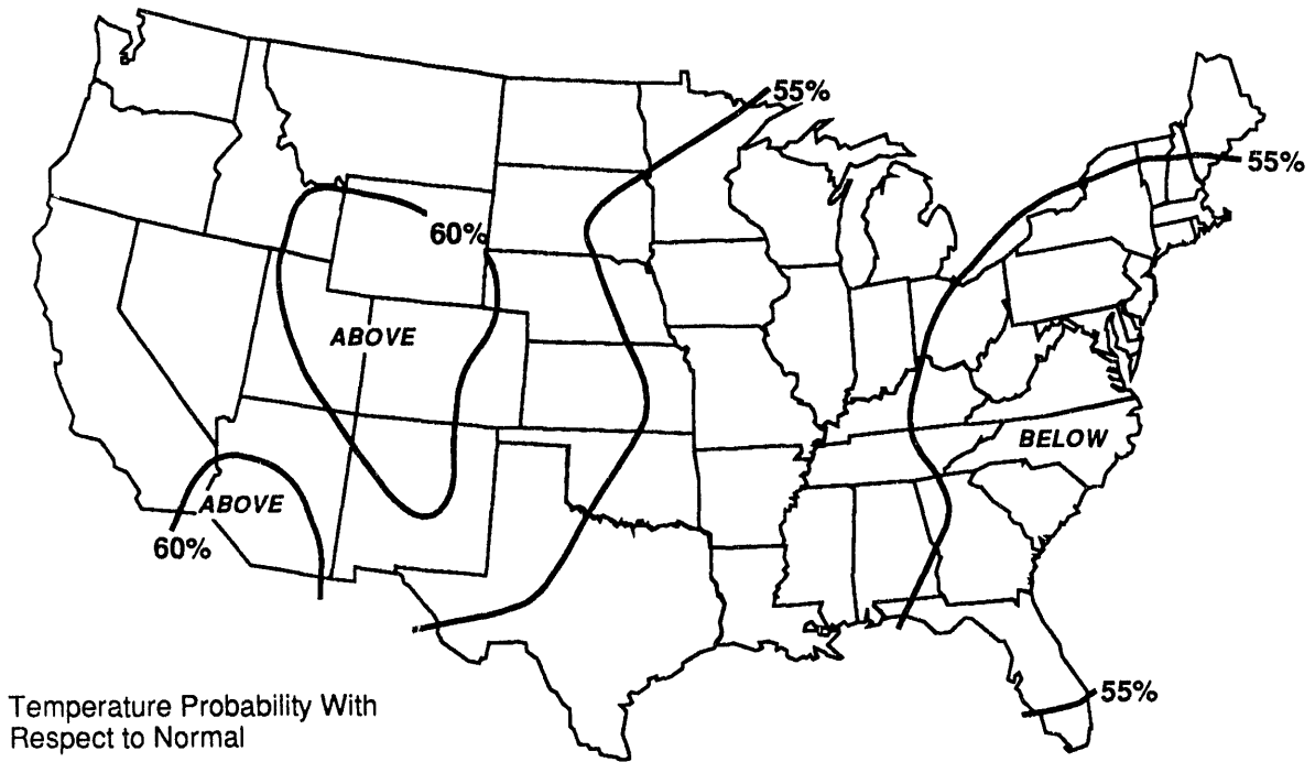
Figure 36. 30 Day Temperature Outlook for March 1994
