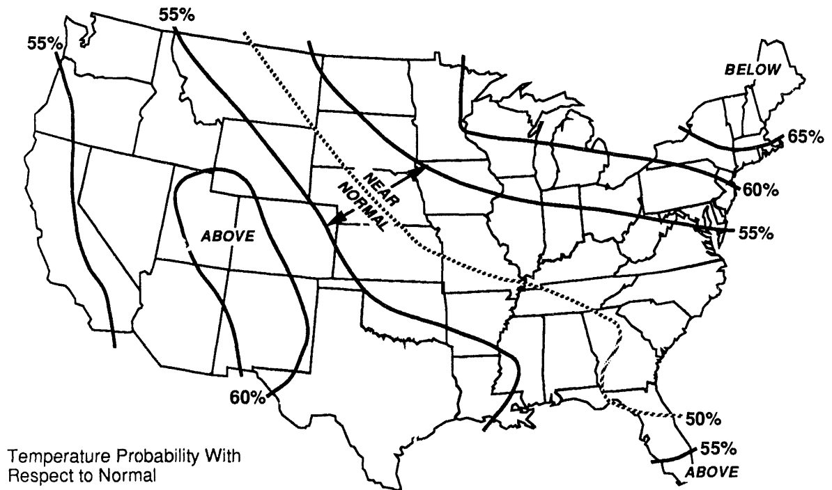
Figure 37. 90 Day Temperature Outlook for March 1994 Through May 1994
