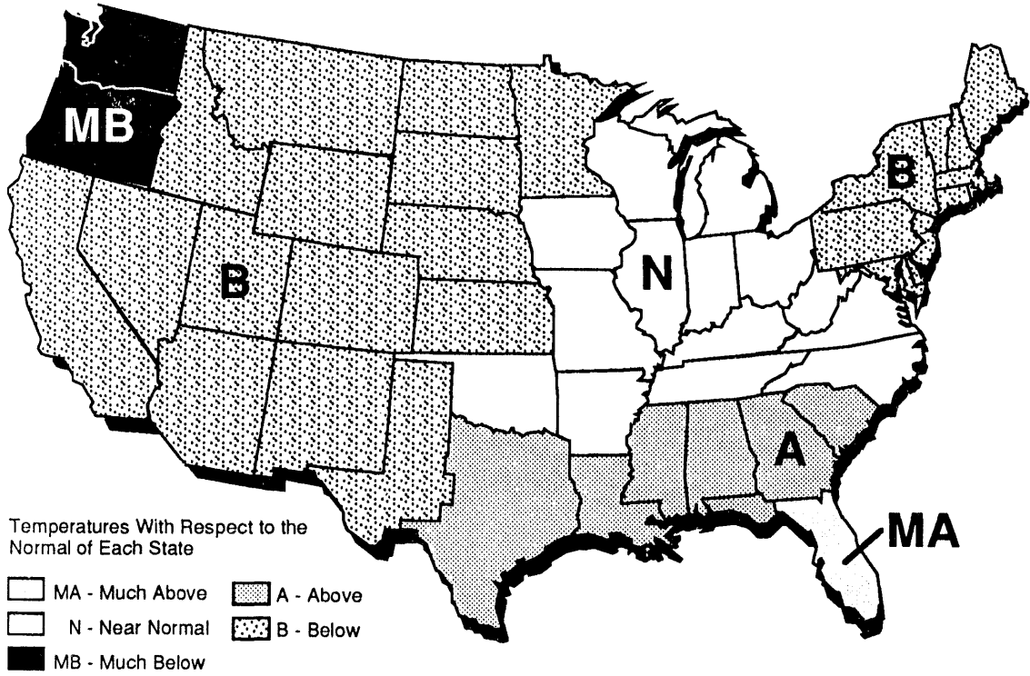
Figure 34. 6 - 10 Day Temperature Outlook for March 22 Through March 26, 1994
