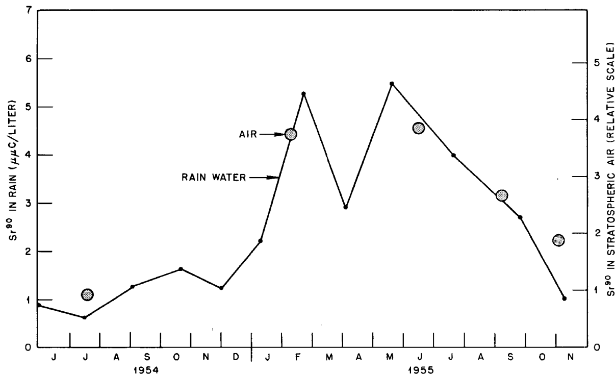
Fig. 4—Correlation between \text{Sr}^{90} concentrations in rain water and in the lower stratosphere.
