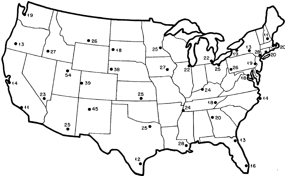
Fig. 5—Cumulative \text{Sr}^{90} deposition in United States as of June 1957, gummied film measurements.
