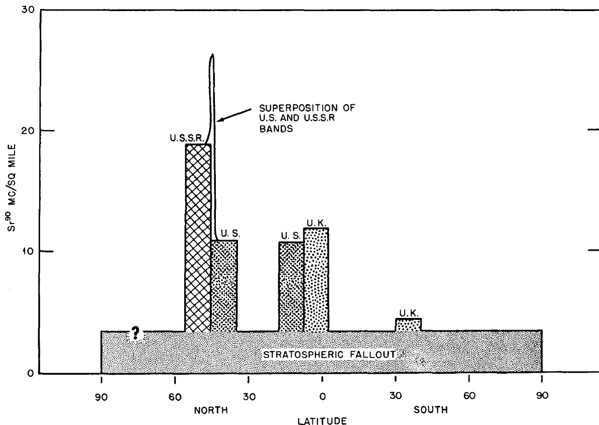
Fig. 3—Theoretical latitudinal fallout profile, December 1957.
