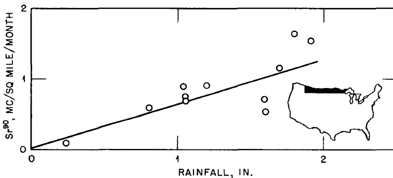
Fig. 3b—Regression of Sr^{90} in rain water on the amount of rainfall collected March through July 1956 at International Falls, Glasgow, Helena, Boise, and Spokane.
