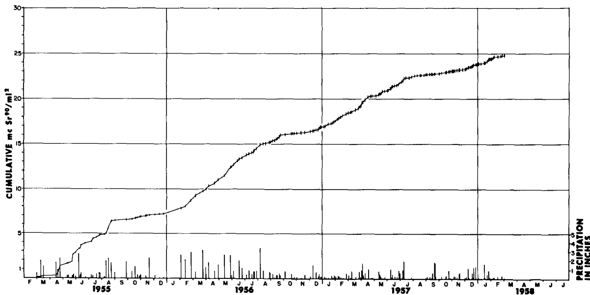
Fig. 2—Sr 90 in Pittsburgh fallout. (Galvanized tub collections.)
