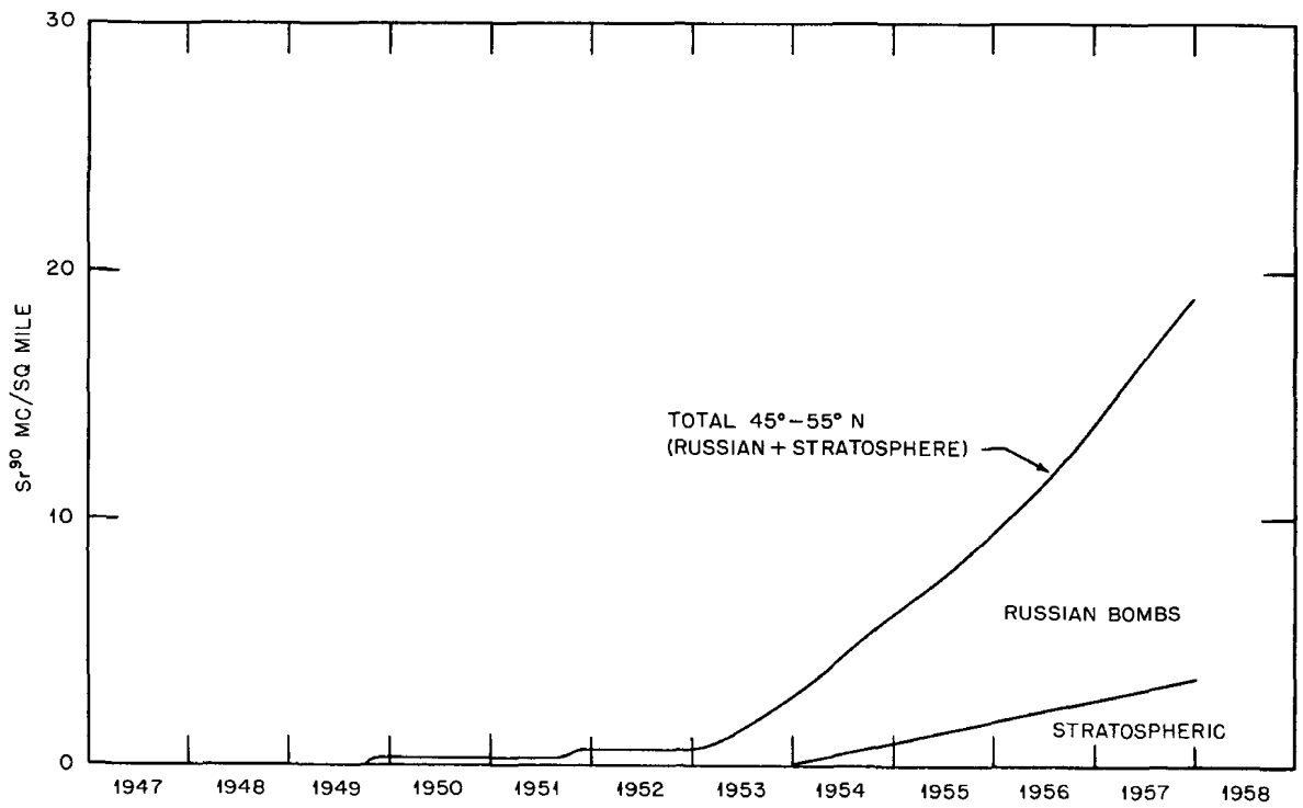
Fig. 8—Predicted Sr 90 fallout curves; total fallout 45°N-55°N.
