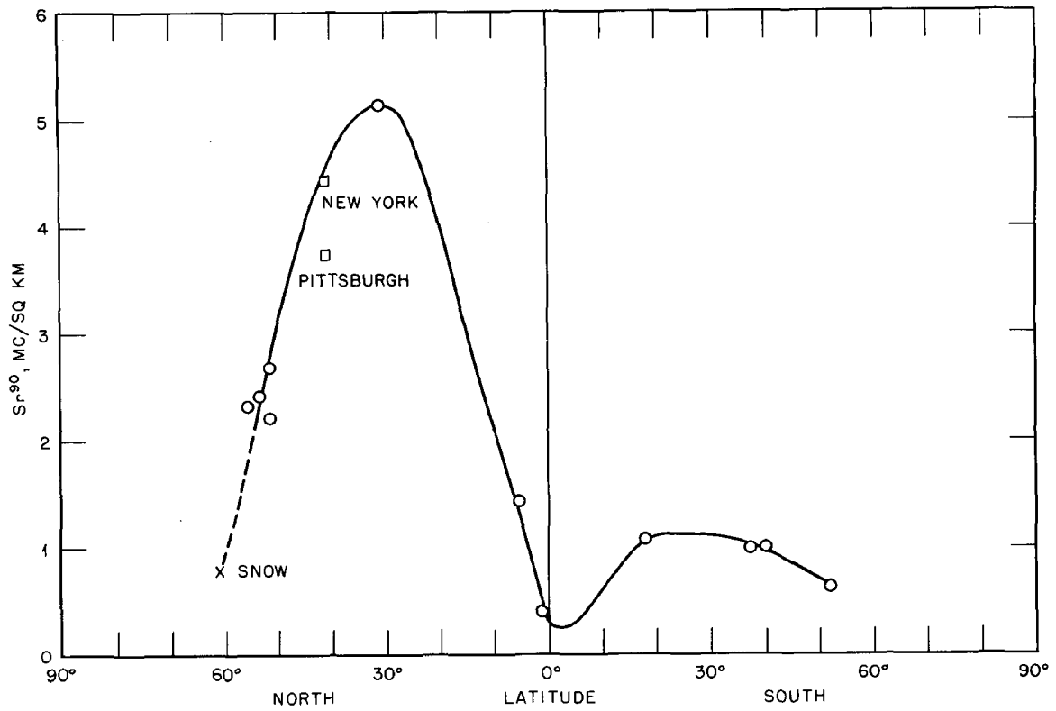
Fig. 10— Total deposition of Sr 90 in 1956 at various latitudes.
