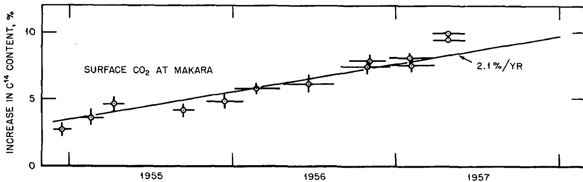
Fig. 10—Bomb \text{C}^{14} effect.
