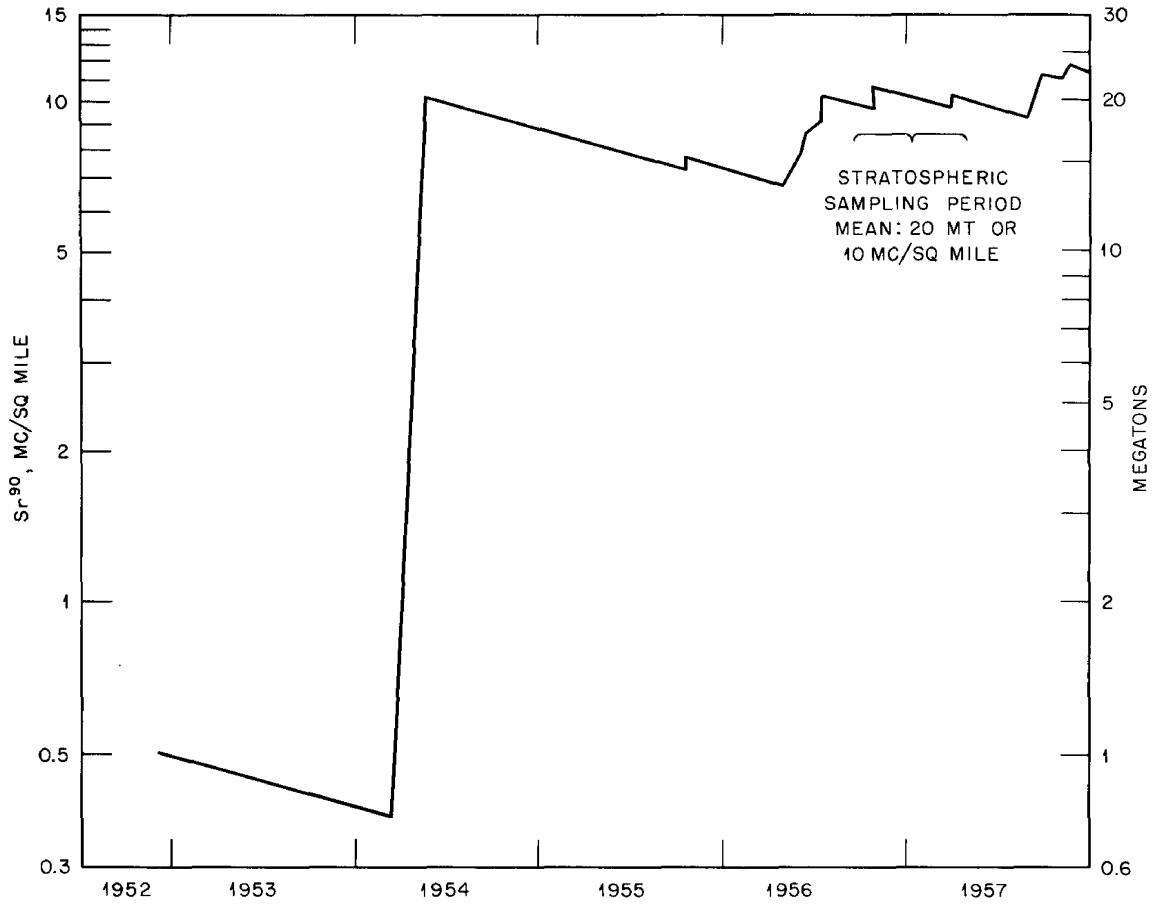
Fig. 7—Stratospheric inventory.
