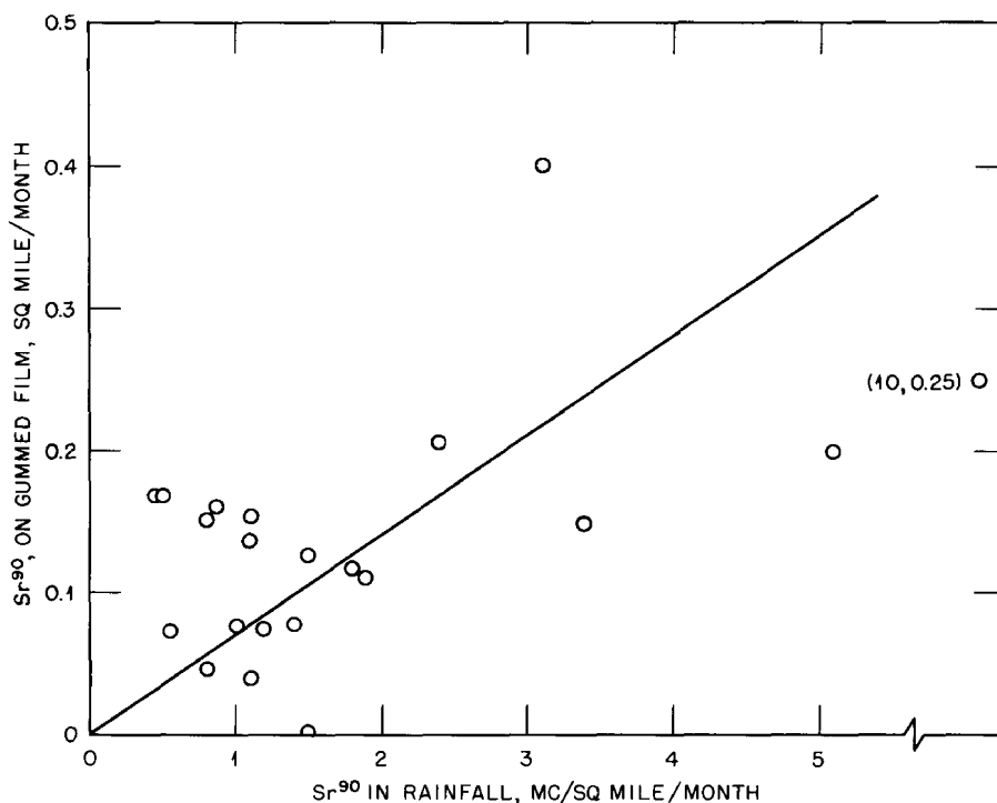
Fig. 5—Regression of Sr 90 in gummied film on Sr 90 in rain water from 20 stations in May 1956.
