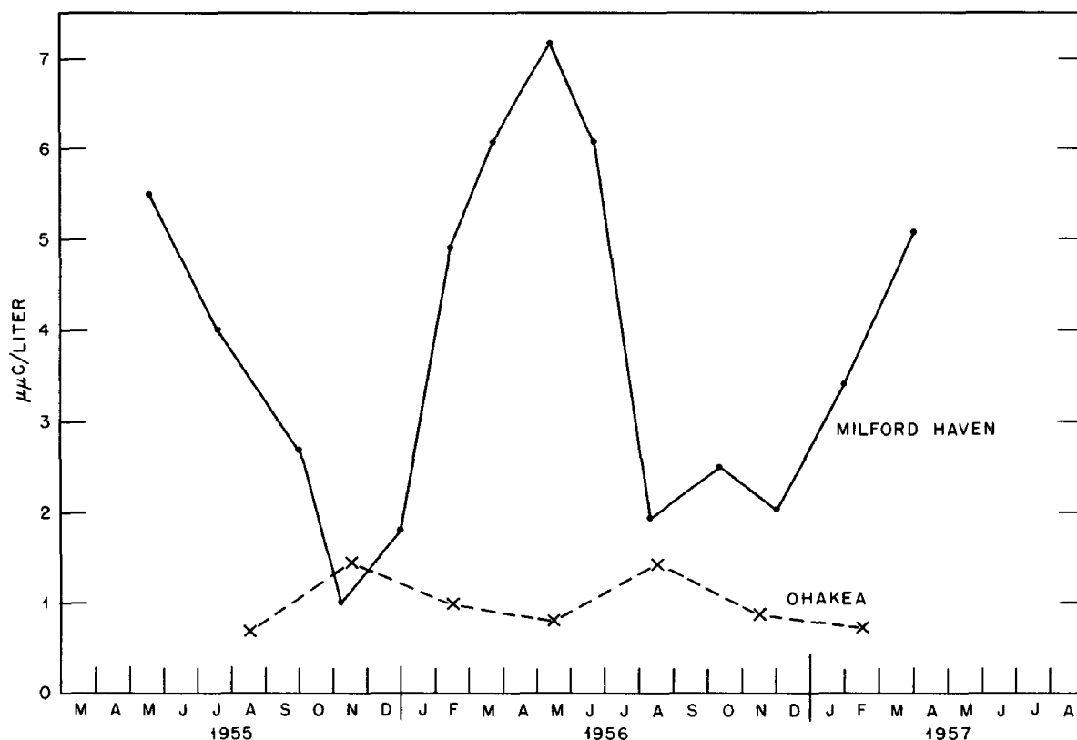
Fig. 6—Seasonal variation of \text{Sr}^{90} content of rain water at Milford Haven and Ohakea.
