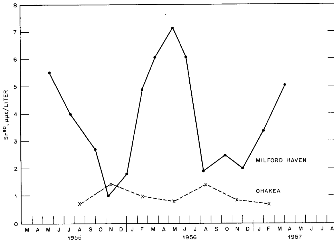
Fig. 12—Seasonal variation of Sr 90 content in rain water at Milford Haven, England, and Ohakea.
