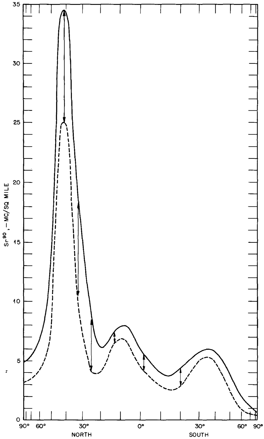
Fig. 3—Adjusted soil data: -----, 1956 soil data; —, data adjusted to December 1957. Vertical arrows show pot data used for adjustment.
