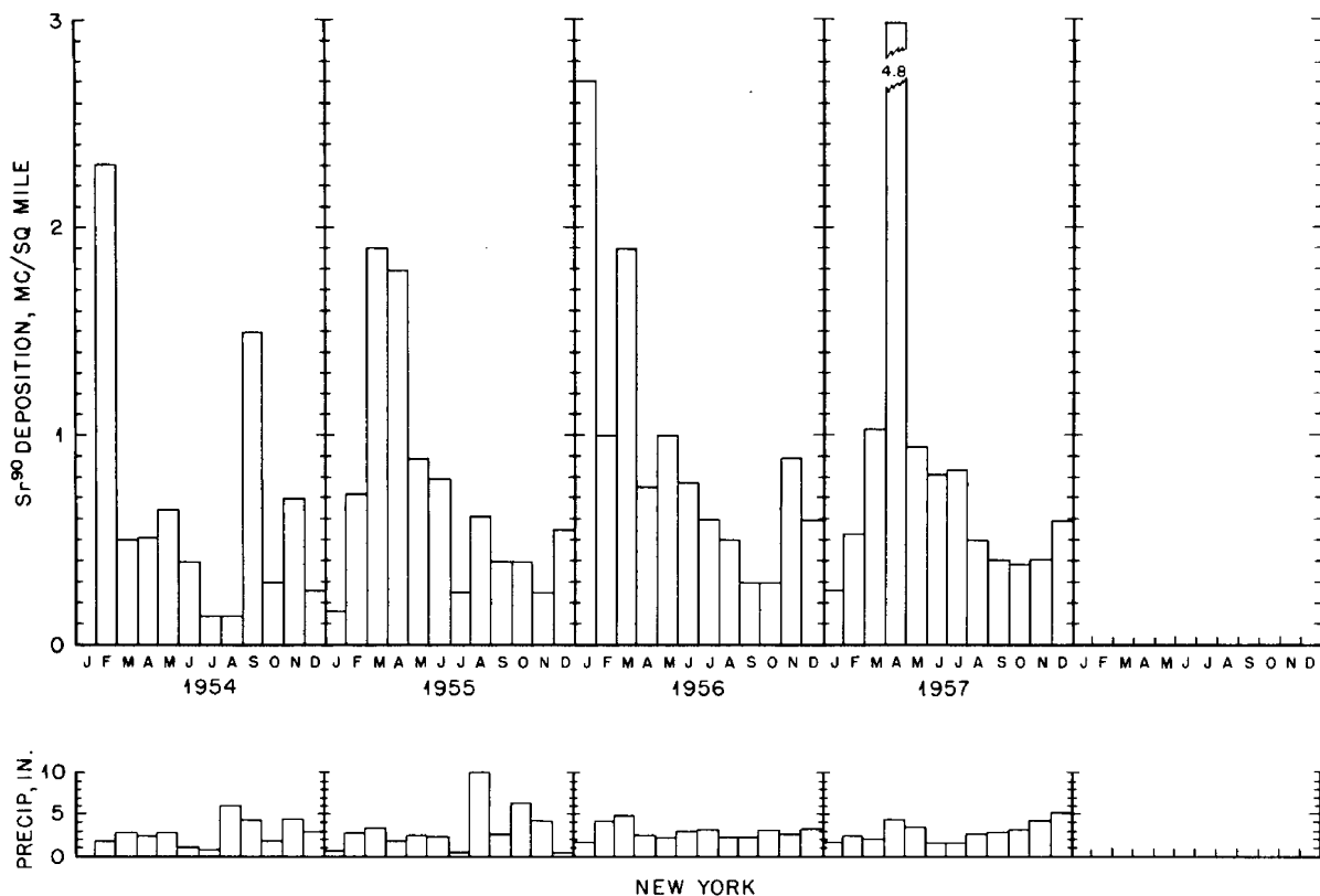
Fig. 5 — Sr 90 deposition, New York, 1954-1957.
