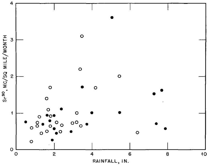
Fig. 2d—Regression of Sr 90 in rain water on the amount of rainfall in June 1956.
