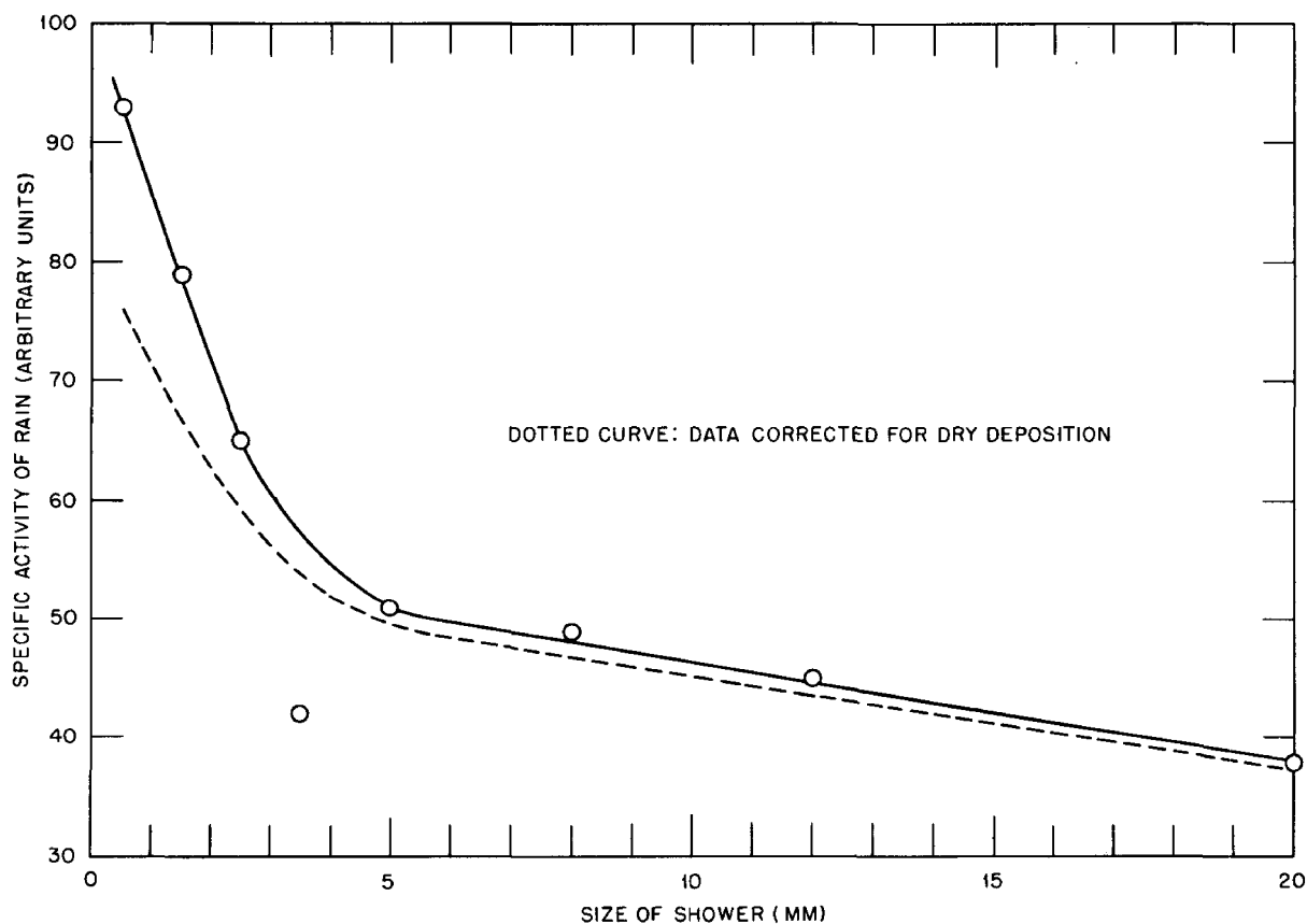
Fig. 1—Variation of specific activity of rain water with size of shower.
