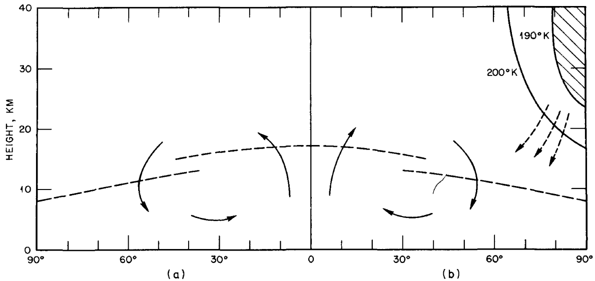
Fig. 7— Atmospheric circulation model (after Dobson and Brewer). a. Summer. b. Winter.
