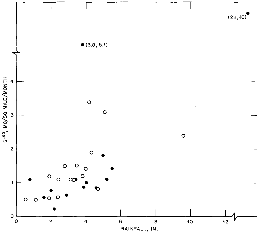
Fig. 2c—Regression of Sr^{90} in rain water on the amount of rainfall in May 1956.
