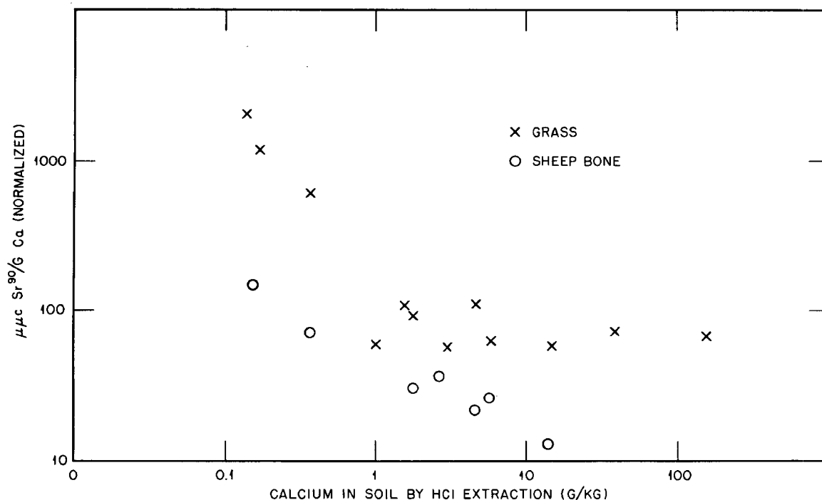
Fig. 5—Correlation of Sr 90 in grass and sheep bone with soil calcium (normalised to 5000 μμc/m 2 in soil).
