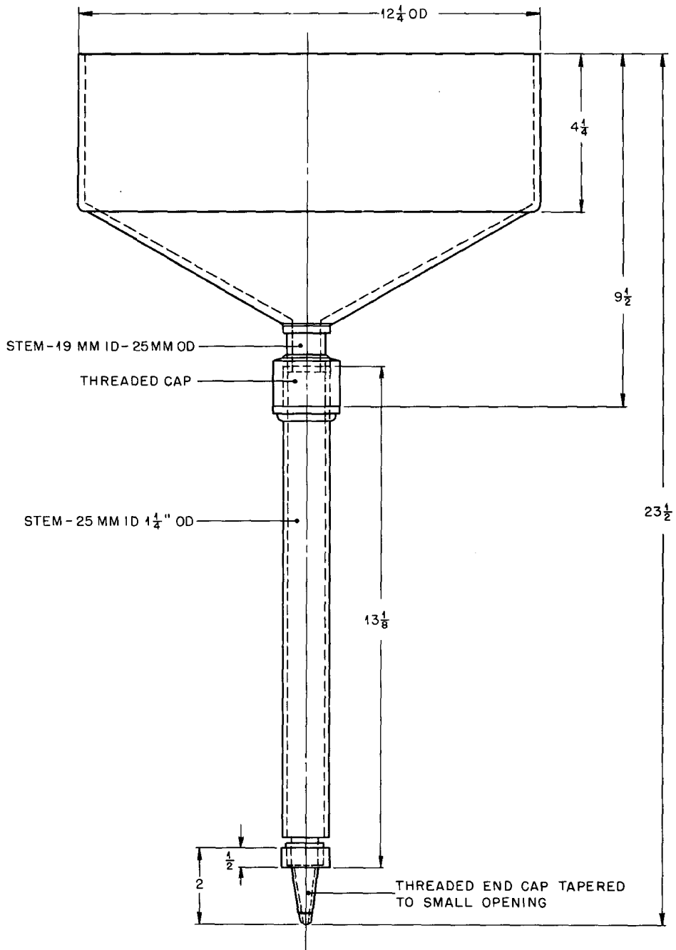
Fig. 1 — Ion-exchange fallout collector.
