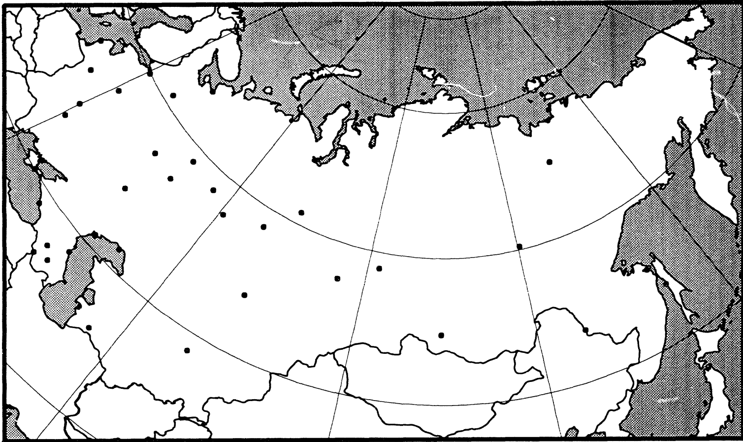
Figure 2. Observing network in 1885. Weather stations are denoted by large black dots. With only 36 posts collecting data, coverage of the country was extremely poor. Most stations were located in major population centers west of the Ural mountains and at ports along the Black and Caspian seas. In contrast, vast tracts of Siberia were virtually unrepresented. Coverage over the eastern half of the country remained sparse through the late 19th and early 20th centuries.
