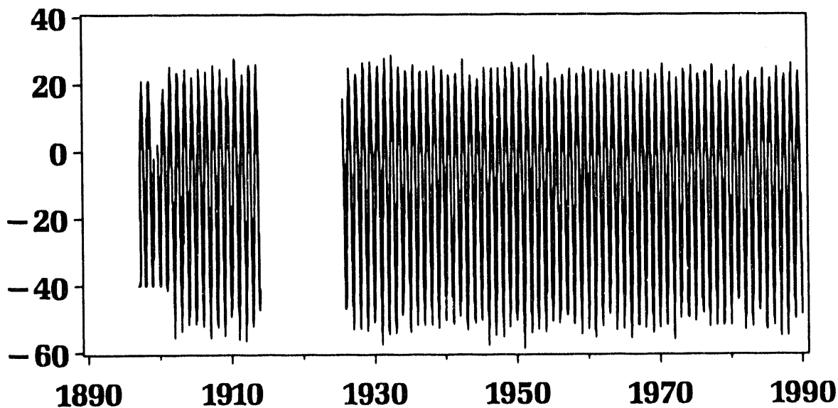
Figure 6. Mean temperature record at Ust'-Maja. Through a visual inspection of the time series, it was noted that no values of less than -40^{\circ}\text{C} were recorded at the site prior to 1902. Visual quality assurance checks such as this identified 25 time series with extensive data quality problems.
