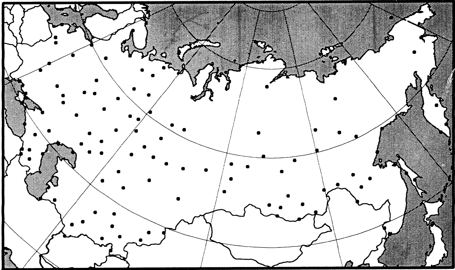
Figure 3. Observing network in 1935. Weather stations are denoted by large black dots. With 117 posts collecting data, most of the country was well-sampled. However, because of their relative underpopulation, some areas north of the Arctic Circle and east of the Ural mountains still lacked adequate coverage. Many of these gaps were filled the next year, when 65 additional posts were opened.
