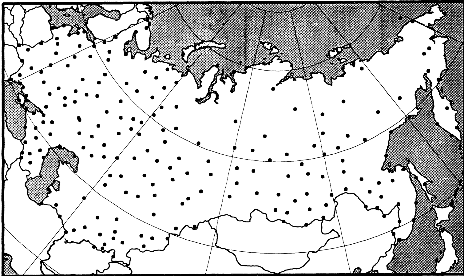
Figure 4. Observing network in 1985. Weather stations are denoted by large black dots. With 222 posts collecting data, virtually all of the country, with the exception of a few areas north of the Arctic Circle and east of the Ural mountains, was well-sampled. From a practical standpoint, the data set can probably be used to study long-term climate variations over the USSR as a whole for the period 1936–89.
