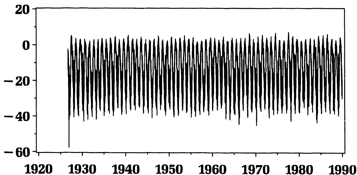
Figure 5. Minimum temperature record at Ostrov Vrangelja. Through a visual inspection of the plotted time series, the presence of several anomalously low temperature values early in the record was noted. In general, visual quality assurance checks identified suspect observations in a number of time series.
