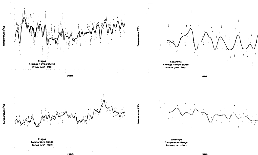
FIG. 6. Time series of the variations of the annual diurnal temperature range and the annual mean temperature from two long-term stations: Sodankyla, Finland, which has been designated as a climate reference station, and the Prague Klementinum-Observatory, Czechoslovakia. Smooth curve same as in Fig. 3.
