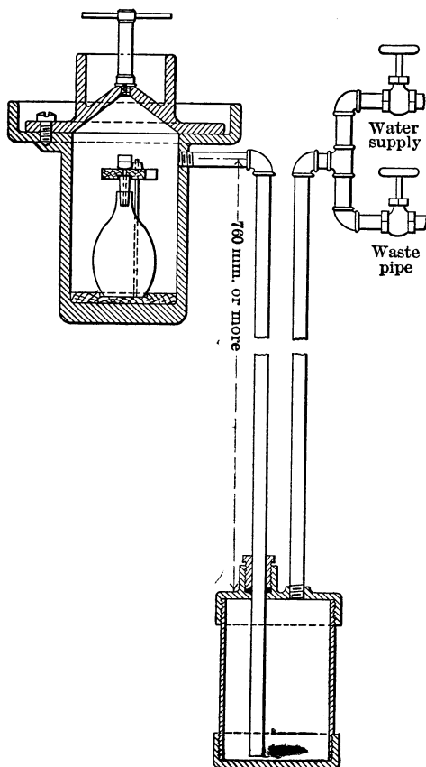
FIGURE 5.—Densimeter.
