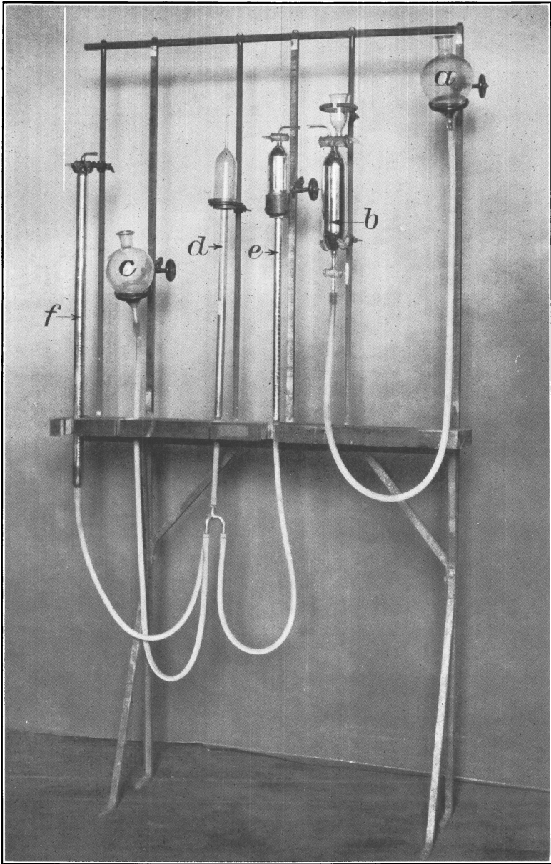
NITROMETER.
