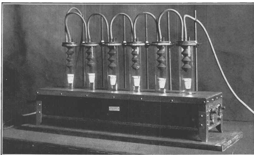
A. APPARATUS FOR ETHER EXTRACTION. WILEY EXTRACTOR.
