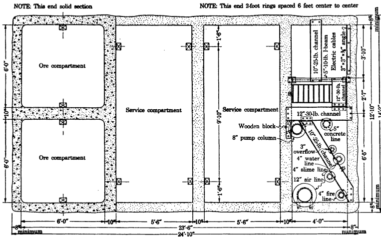
FIGURE 1.—Cross section of United Verde No. 7 shaft
