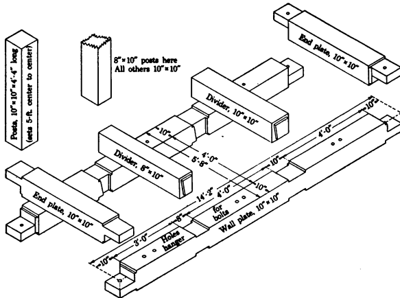
FIGURE 29.—Shaft set, Magma mine. (All daps, 1 inch; corners fastened with wooden dowel pins)
