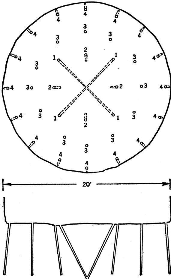
FIGURE 16.—Round used in Randfontein shaft. (Numbers on holes indicate firing order)
