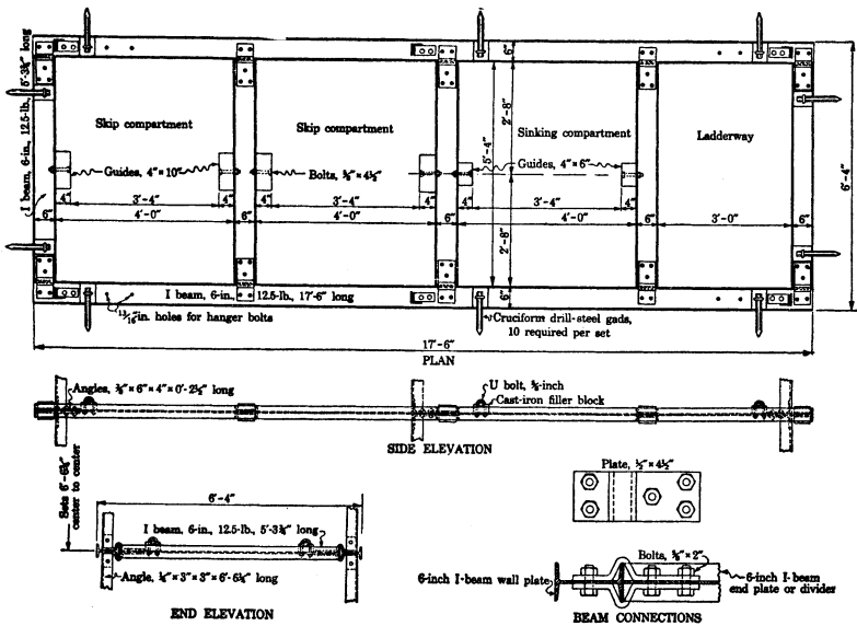
FIGURE 36.—Steel shaft set, Interior shaft, Santa Marghrita mine, Cia. Real del Monte y Pachuca
