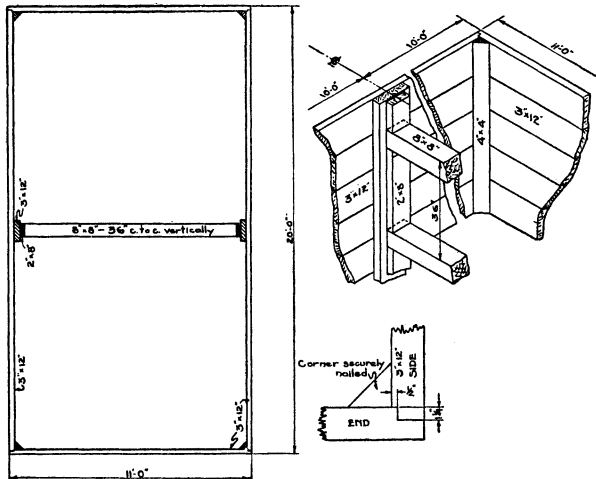
FIGURE 33.—Shaft timbering, Rock Springs mines Nos. 4 and 5, Union Pacific Coal Co., Wyoming
