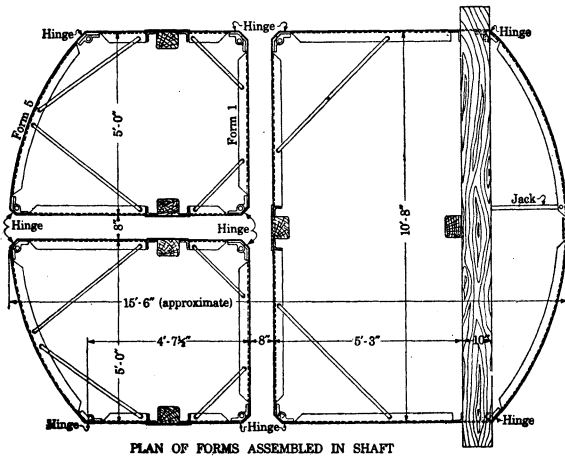
FIGURE 39.—Steel forms with rounded ends for concreting Campbell shaft
