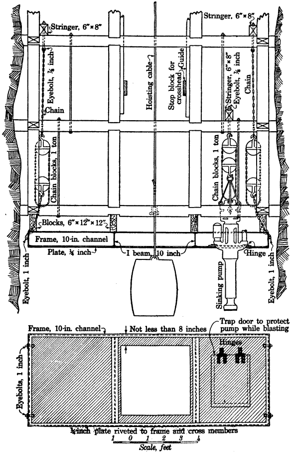
FIGURE 28.—Suspended bulkhead used for shaft sinking by Walter Fitch, Jr., Co.
