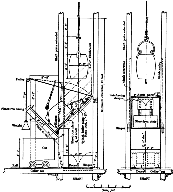
FIGURE 18.—Arrangement for dumping buckets at surface, used by the Walter Fitch, jr., Co., Eureka, Utah
