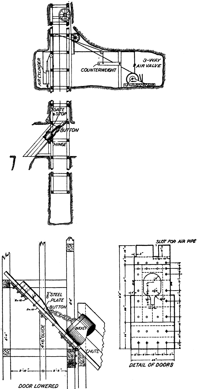
FIGURE 19.—Arrangement for dumping buckets at Engels mine, California
