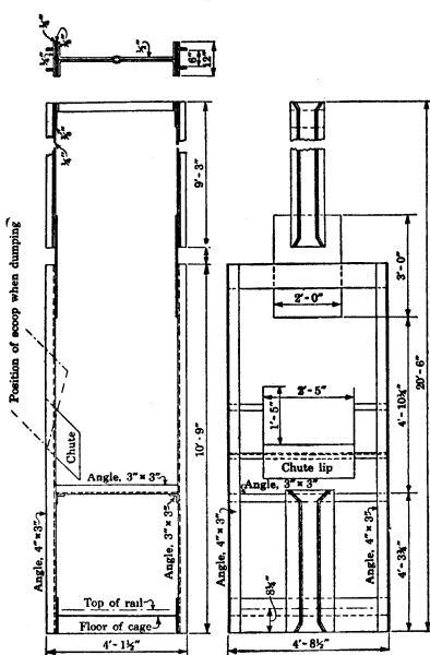
FIGURE 23.—Details of cage used in sinking Guadalupe shaft. (All joints and connections are riveted; standard safety dogs are used)
