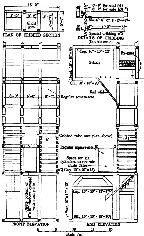
FIGURE 6.—Method of timbering shaft, Utah Copper Co.
