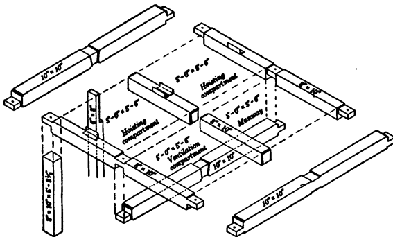
FIGURE 30.—Sets at South shaft, Teck-Hughes mine
