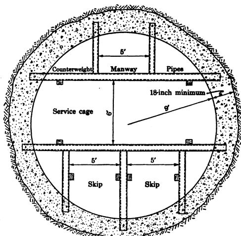
FIGURE 2.—Cross section of circular shaft
