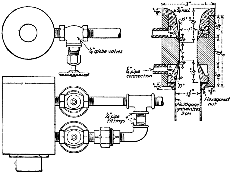
FIGURE 5.—Compressed-air injector used by Moctezuma Copper Co. for ventilating raises through diamond-drill holes
