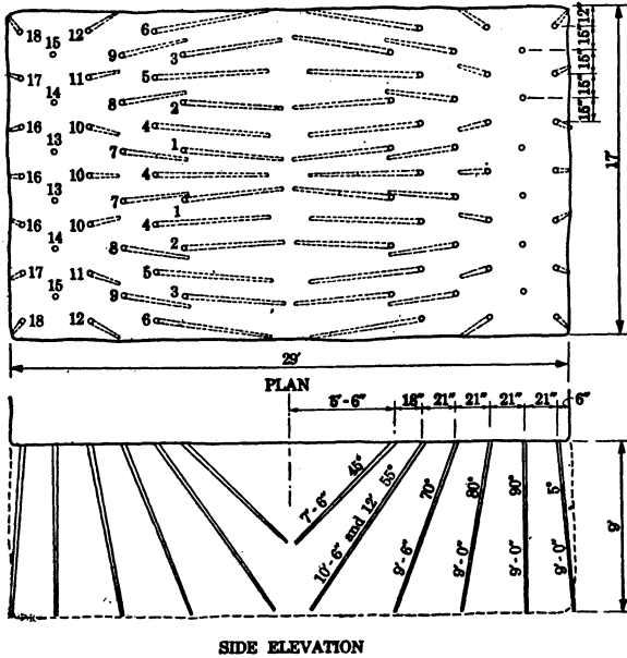
FIGURE 12.—Round used in Frood No. 3 shaft. (Numbers on holes indicate firing order)
