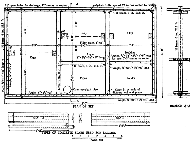
FIGURE 35.—Steel shaft set
