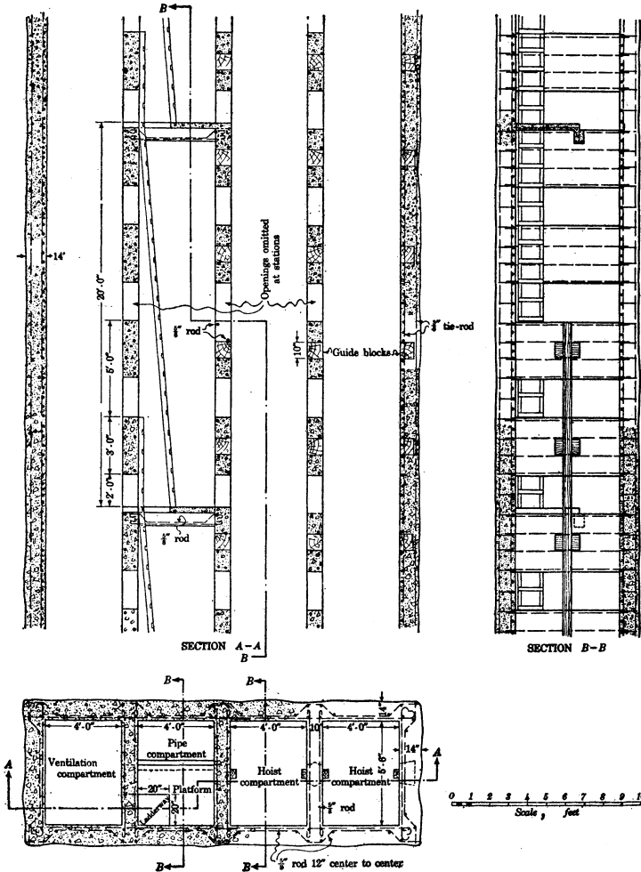
FIGURE 40.—General shaft plans and standard reinforcement, Magma Copper Co.
