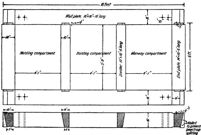
FIGURE 32.—Sets at Argonaut inclined shaft
