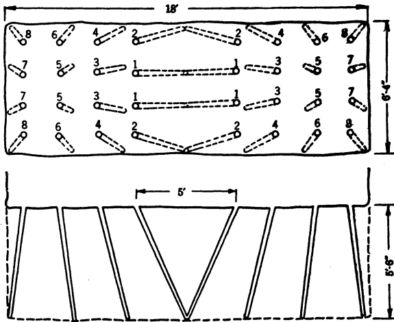
FIGURE 8.—Shaft round used at United Verde mine in medium ground. (Numbers indicate firing order)
