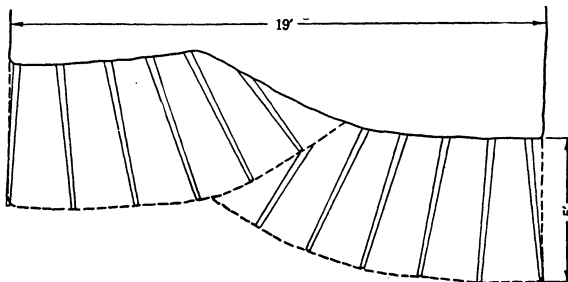
ELEVATION SHOWING TWO SUCCESSIVE ROUNDS FIGURE 13.—Round used in McPherson shaft, Tennessee Copper Co.
