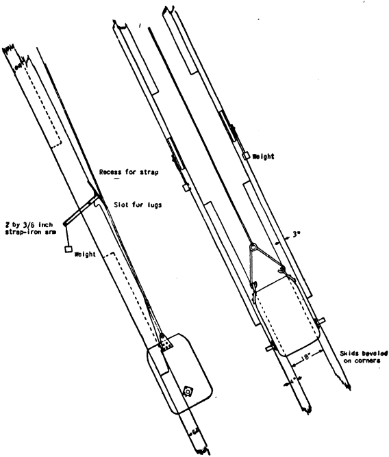
FIGURE 20.—Arrangement for dumping bucket in inclined shaft
