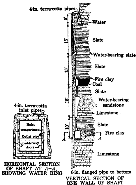
FIGURE 42.—Water rings in concreted coal-mine shaft
