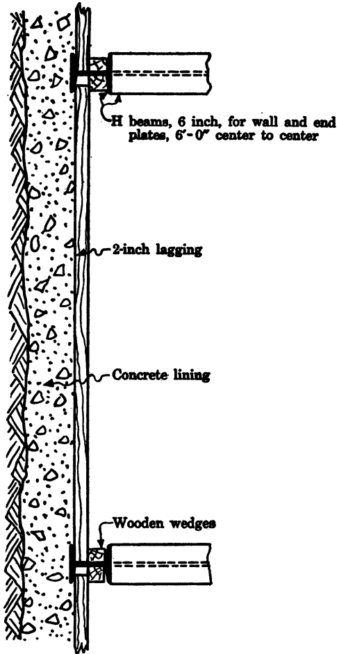
FIGURE 44.—Combination of concrete and steel sets for shaft lining
