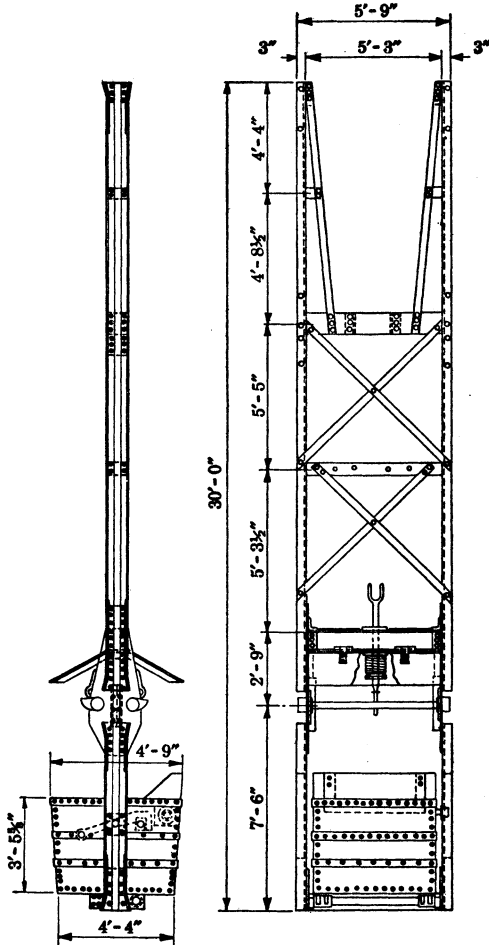
FIGURE 21.—Sinking skip used at Frood No. 3 shaft
