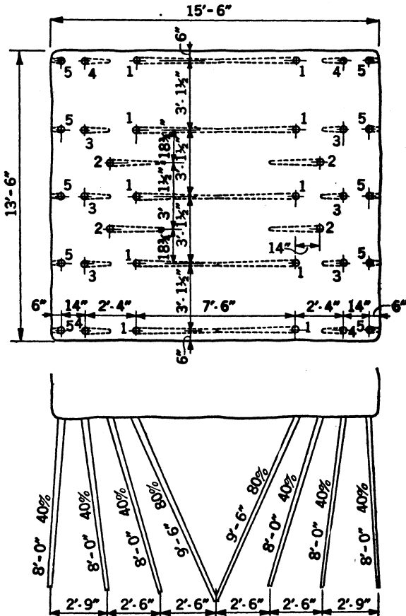
FIGURE 11.—Shaft round in easy-breaking ground at Morenci. (Numbers on holes indicate firing order)
