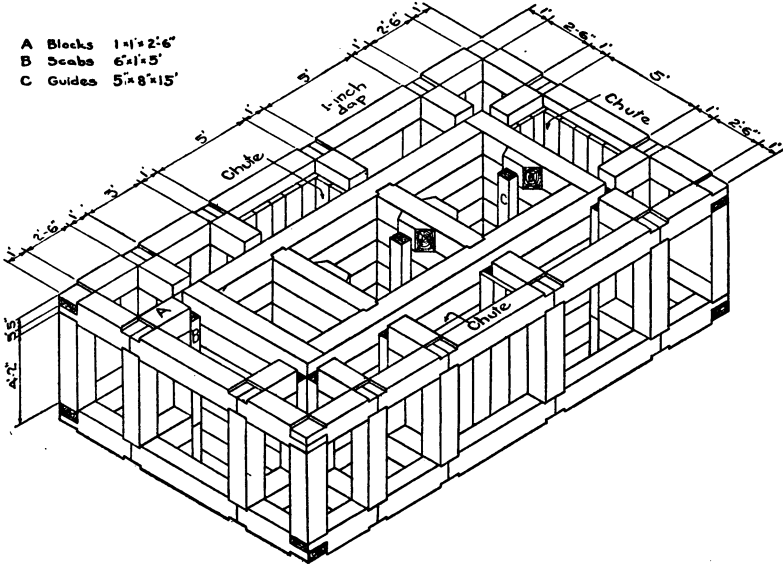
FIGURE 34.—Jacket set around cribbed shaft, Butte & Superior mine
