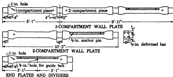
FIGURE 46.—Precast cribbing used at Zaruma, Ecuador
