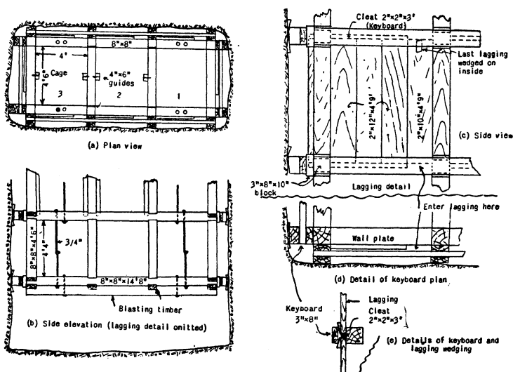
FIGURE 27.—Arrangement of timbering and keyboard lagging, Eighty-Five mines
