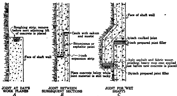
FIGURE 43.—Closure joints in concrete shaft
