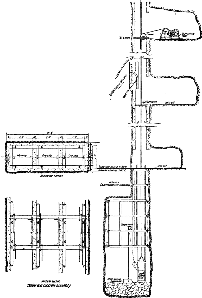
FIGURE 26.—Arrangement for sinking shafts at United Verde mine
