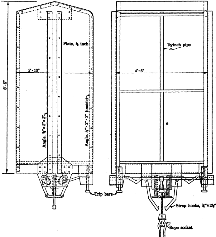
FIGURE 3.—Safety crosshead used in sinking Eureka shaft
