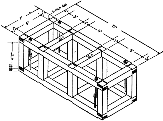
FIGURE 31.—Standard shaft set, Black Rock mine, Butte & Superior Mining Co.
