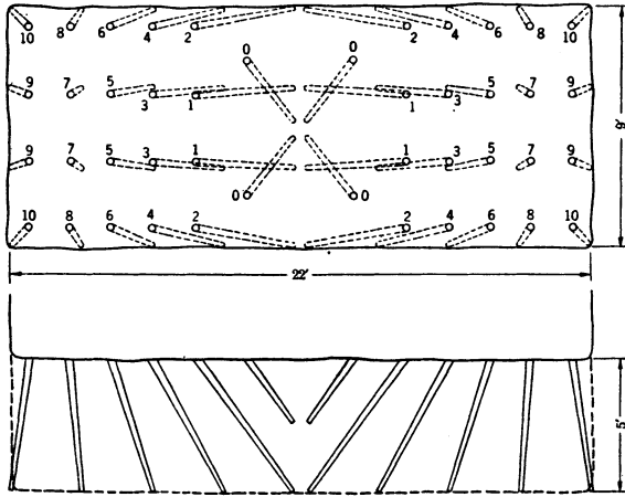
FIGURE 9.—Shaft round, Hecla mine. (Numbers on holes indicate firing order)
