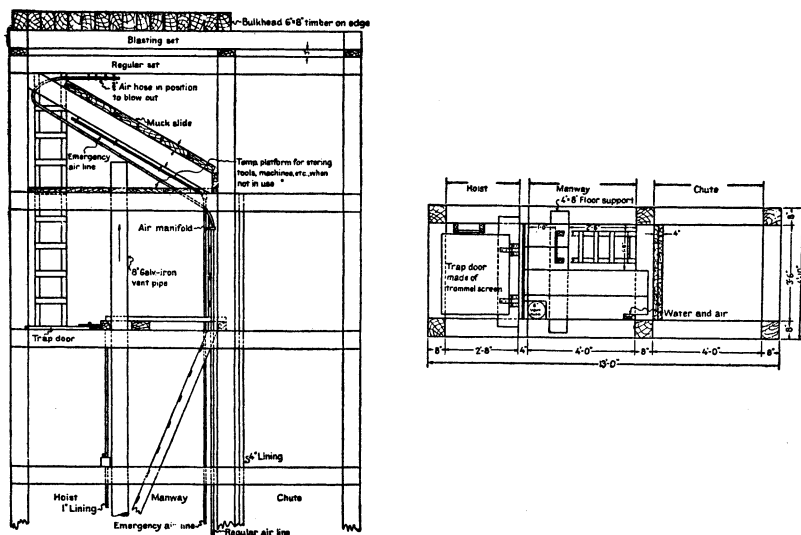
FIGURE 4.—Pilot raise, No. 6 shaft, Morenci, Ariz.
