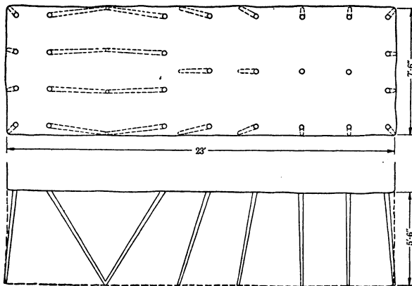
FIGURE 10.—Round used in Guadalupe shaft, Moctezuma Copper Co.
