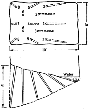
FIGURE 14.—Round for wet shaft of small cross section. (Numbers on holes indicate firing order)
