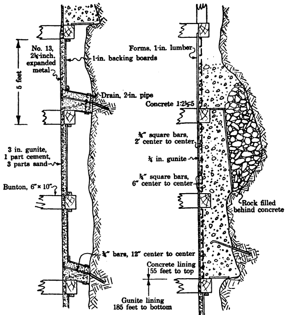
FIGURE 37.—Combination concrete and gunite shaft lining
