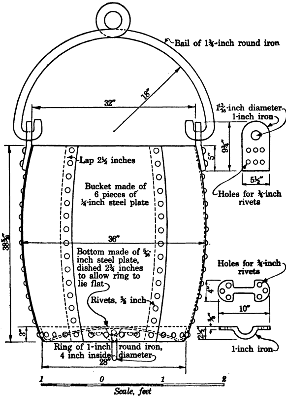
FIGURE 17.—Nineteen-cubic-foot sinking bucket
