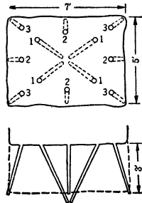
FIGURE 15.—Round for shaft of small cross section. (Numbers on holes indicate firing order)
