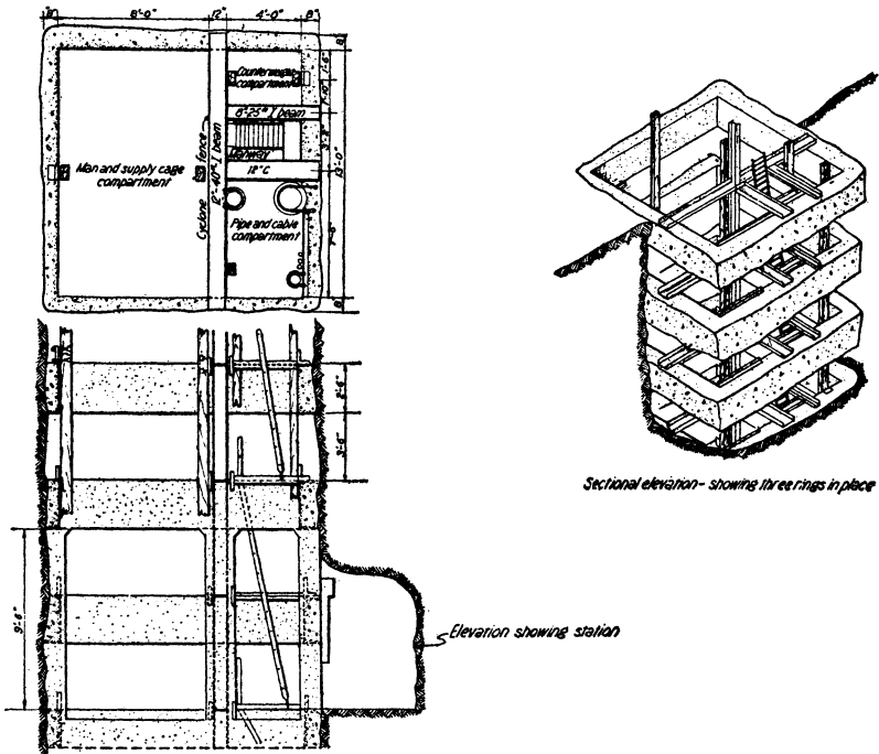
FIGURE 45.—Ring method of concreting shafts, United Verde Copper Co.
