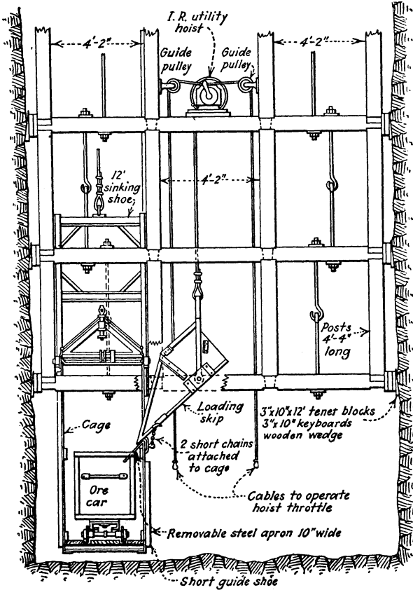
FIGURE 22.—Arrangement for using auxiliary skip at Park Konold mine, Utah
