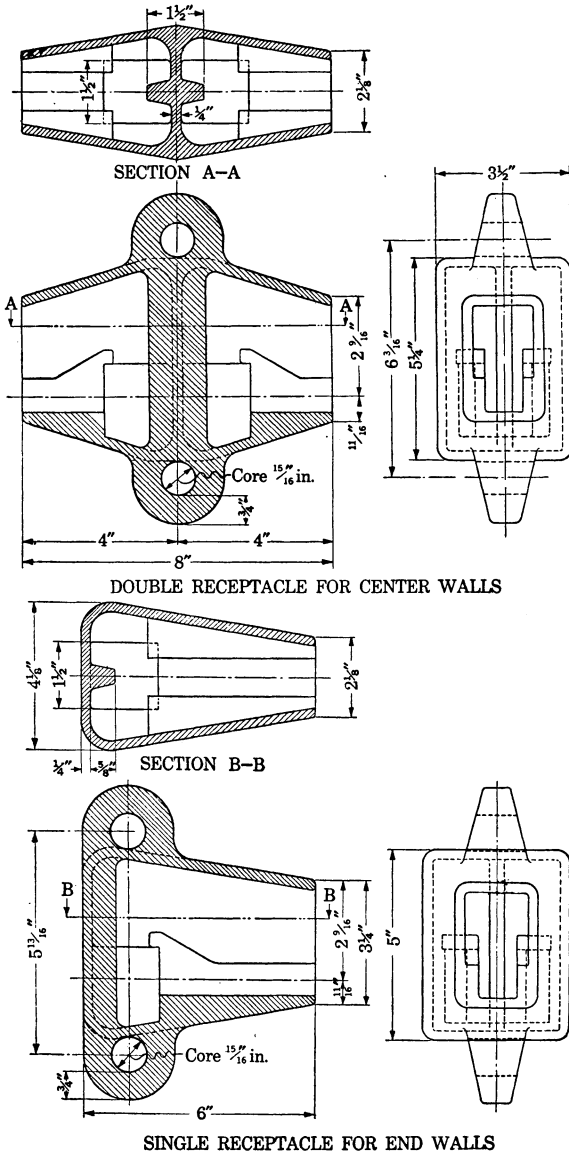
FIGURE 47.—Bolt sockets for attaching guides, Campbell shaft
