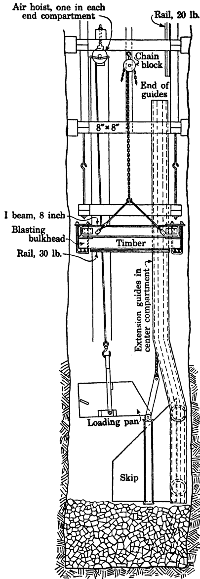
FIGURE 24.—Arrangement for dumping auxiliary pan into skip, North Star mine
