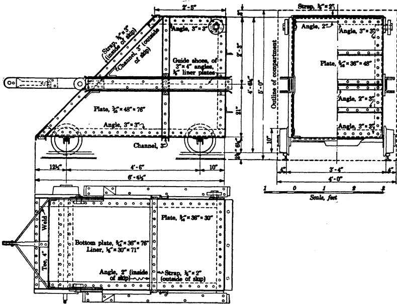
FIGURE 25.—Skip for sinking combination vertical and inclined shaft
