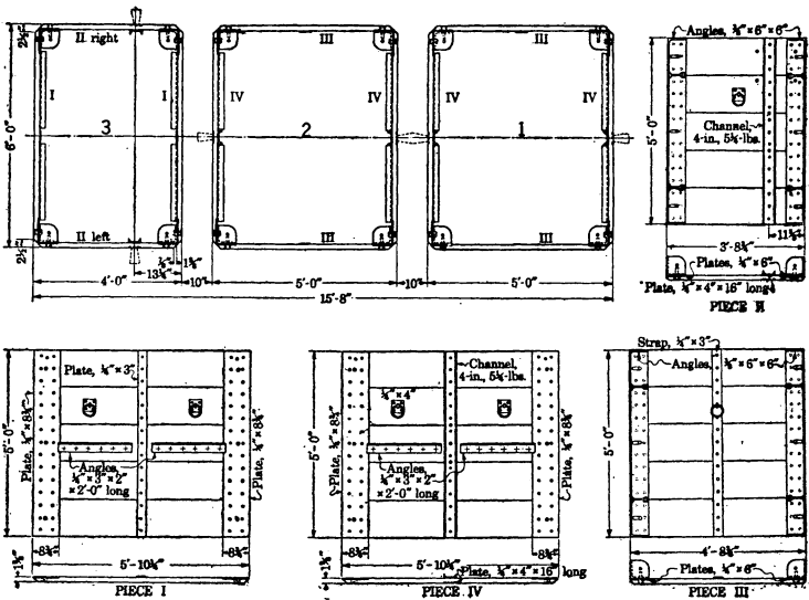
FIGURE 38.—Wooden forms for concreting shaft, used at Calumet and Arizona mine
