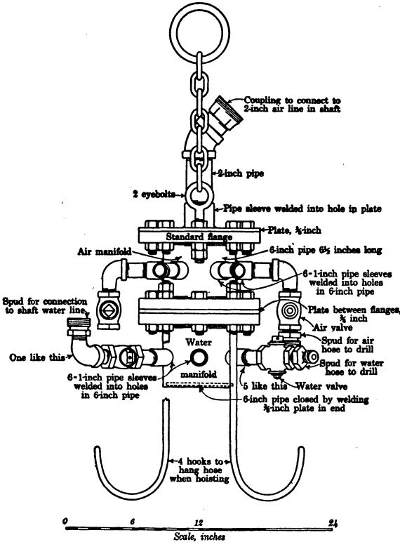
FIGURE 7.—Manifold for drills used at Magma mine
