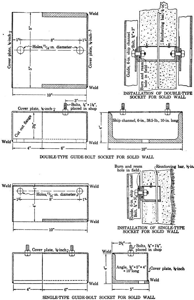
FIGURE 48.—Bolt sockets for attaching guides, skip compartment, No. 7 shaft, United Verde mine
