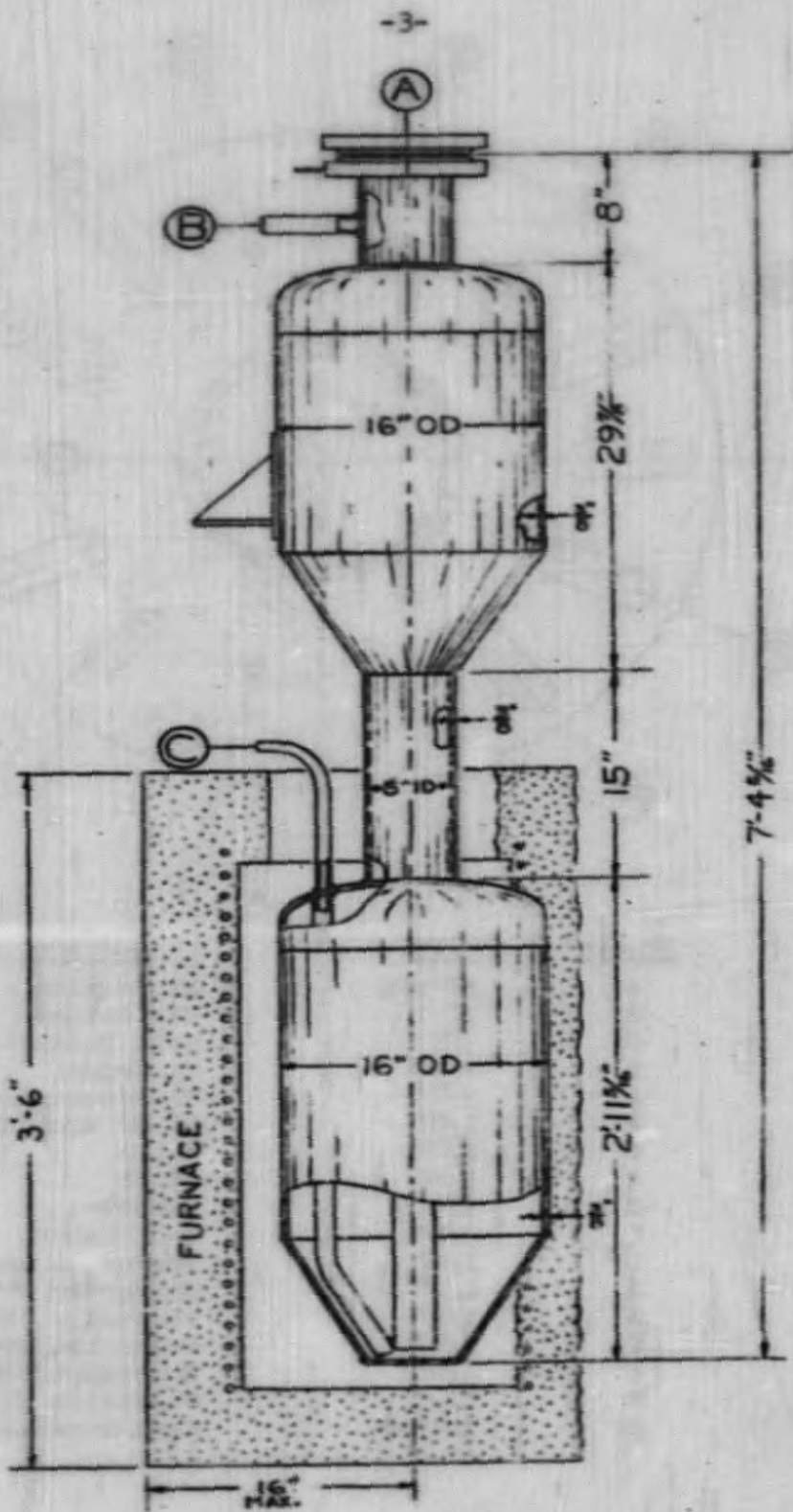
FIG. 1 FLUORINATOR FV-100 MARK III
