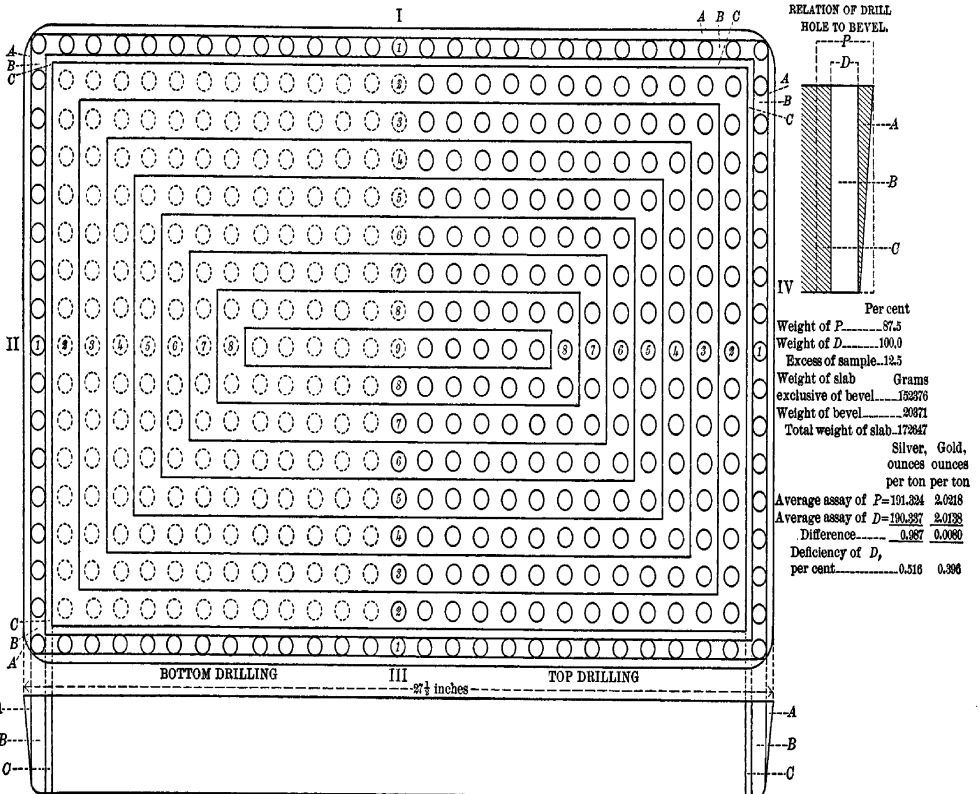
RESULTS OF SAMPLING CONVERTER COPPER SLAB, SHOWING EXTENT OF WEIGHT AND ASSAY ERRORS INCIDENT TO SAMPLING BEVEL ZONE BY DRILLING.
