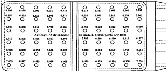
ASSAYS OF SLAB A
