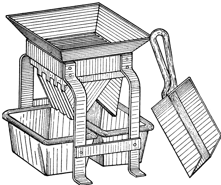
FIGURE 30.—Jones sampler.
