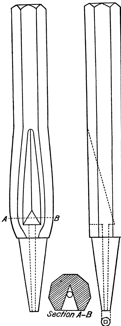
FIGURE 31.—Punch for sampling lead bullion or other soft alloys.
