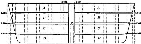
ASSAYS OF SAW CUTS
