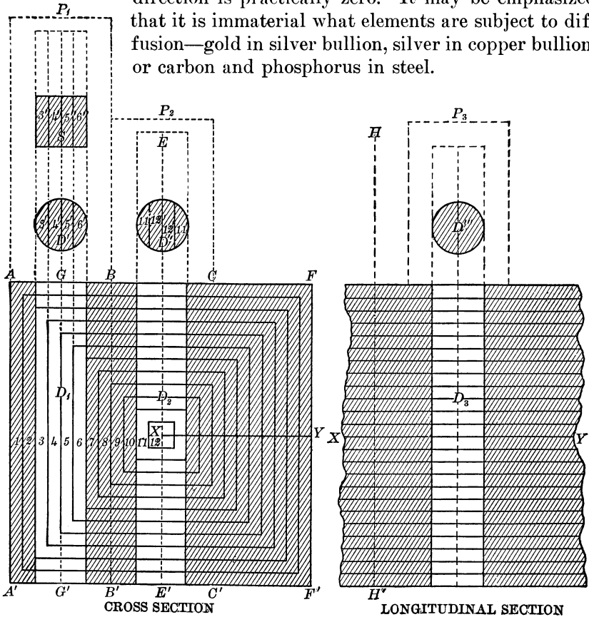
FIGURE 12.—Sections of hypothetical bullion bar. At left, cross section; at right, longitudinal section.
