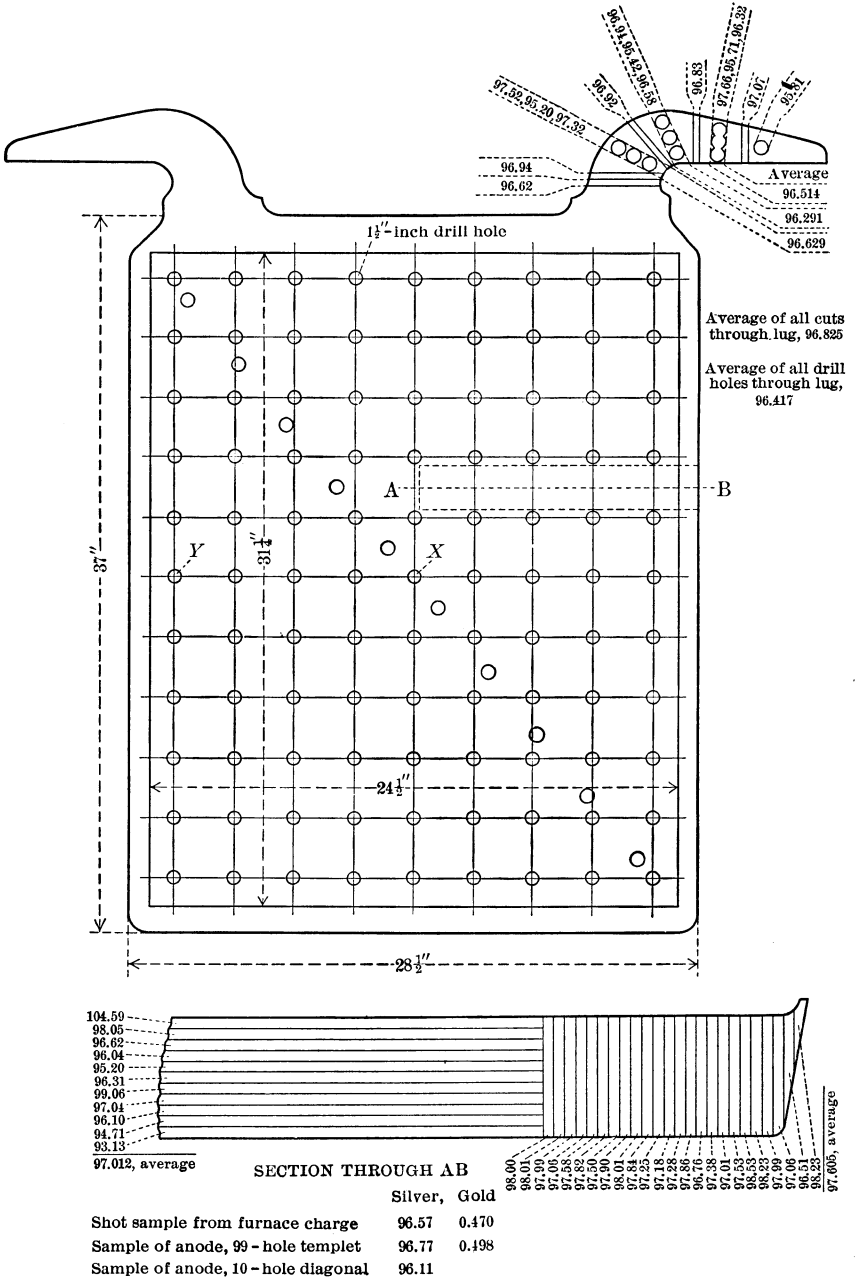
FIGURE 26.—Silver distribution in furnace-refined copper bullion anode. Silver given in ounces per ton.
