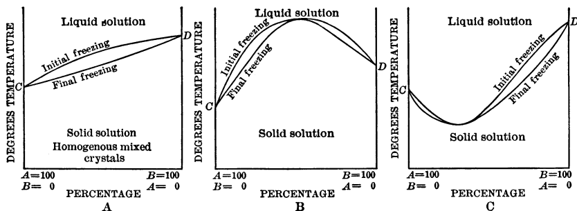
FIGURE 1.—Freezing-point diagrams of binary alloys in which the two substances are miscible in all proportions. A and B , pure substances; C , freezing point of pure substance A ; D , freezing point of pure substance B .
