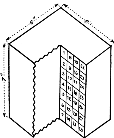
FIGURE 5.—Size of cube used in experiments with copper-silver alloys, showing where 28 samples were taken.
