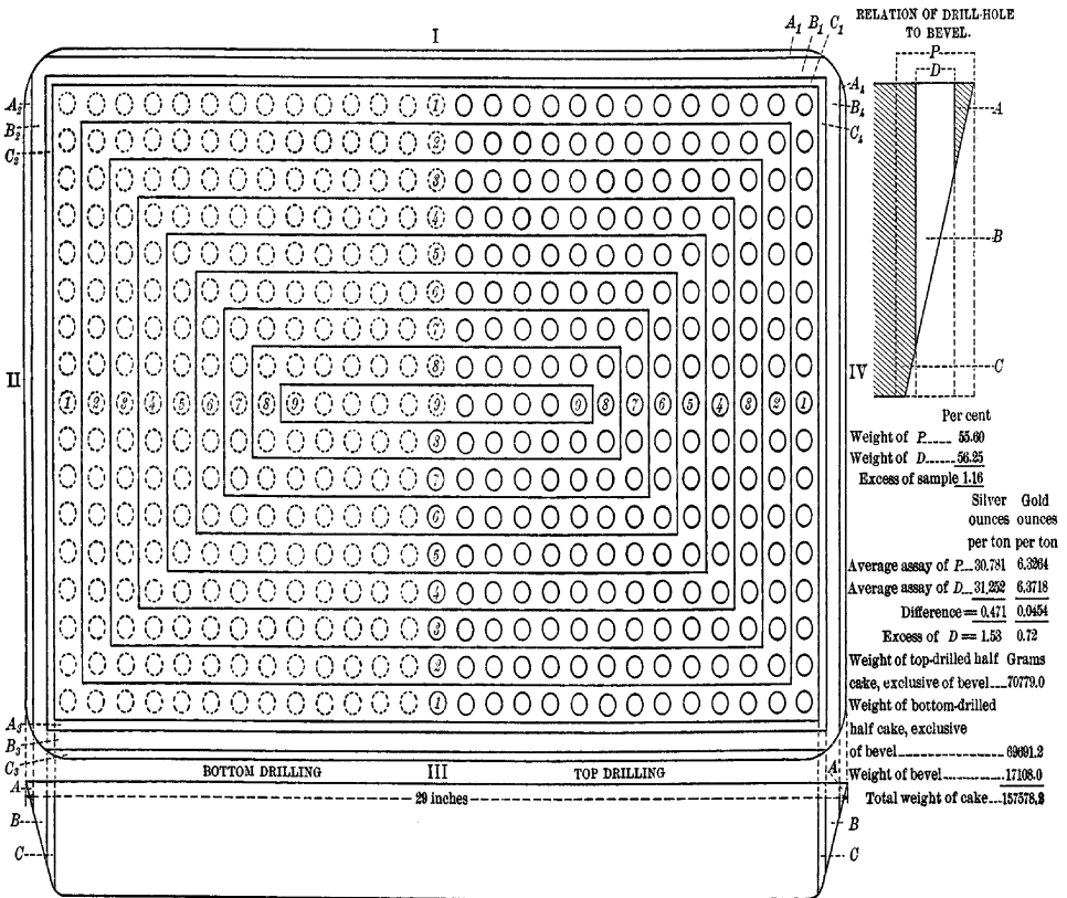
RESULTS OF SAMPLING CONVERTER COPPER SLAB, SHOWING EXTENT OF WEIGHT AND ASSAY ERRORS INCIDENT TO SAMPLING BEVEL ZONE BY CUTTING.
