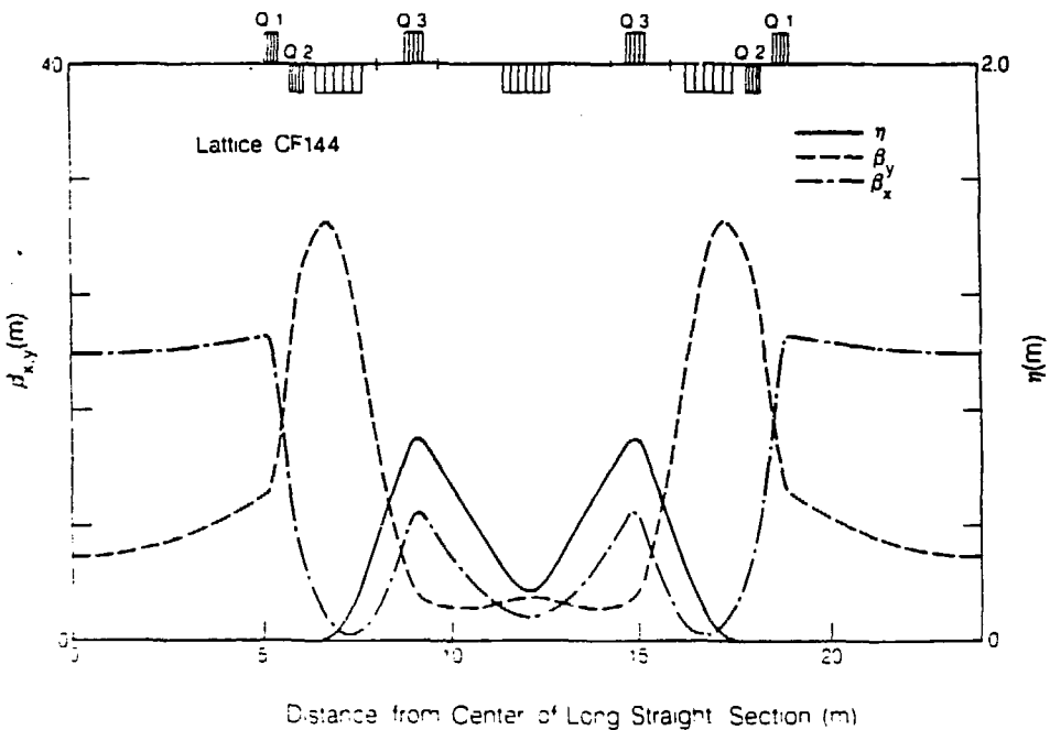
Fig. 4 Lattice structure and functions in one period of lattice CF144. The pattern repeats six times around the ring.
