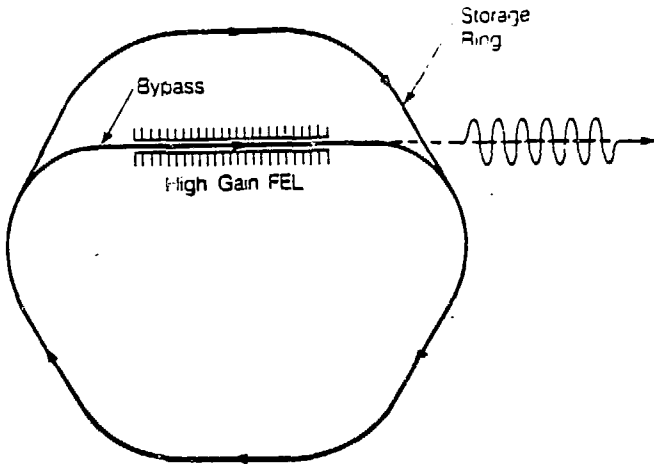
Fig. 1 Schematic drawing of a storage ring with a bypass containing a high gain FEL.
