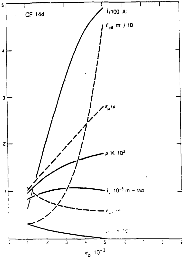
Fig. 2 Dependence of the peak current, \bar{I} , equilibrium emittance, \bar{\epsilon}_x , and some FEL parameters ( \rho , l_e ) on the momentum spread, \sigma_p . Degradation of performance ( \rho_{eff} , l_{eff} ) with increasing momentum spread is apparent. A Lorentzian momentum distribution was assumed in the calculation of the degradation [see Eqn. (2.17)].
