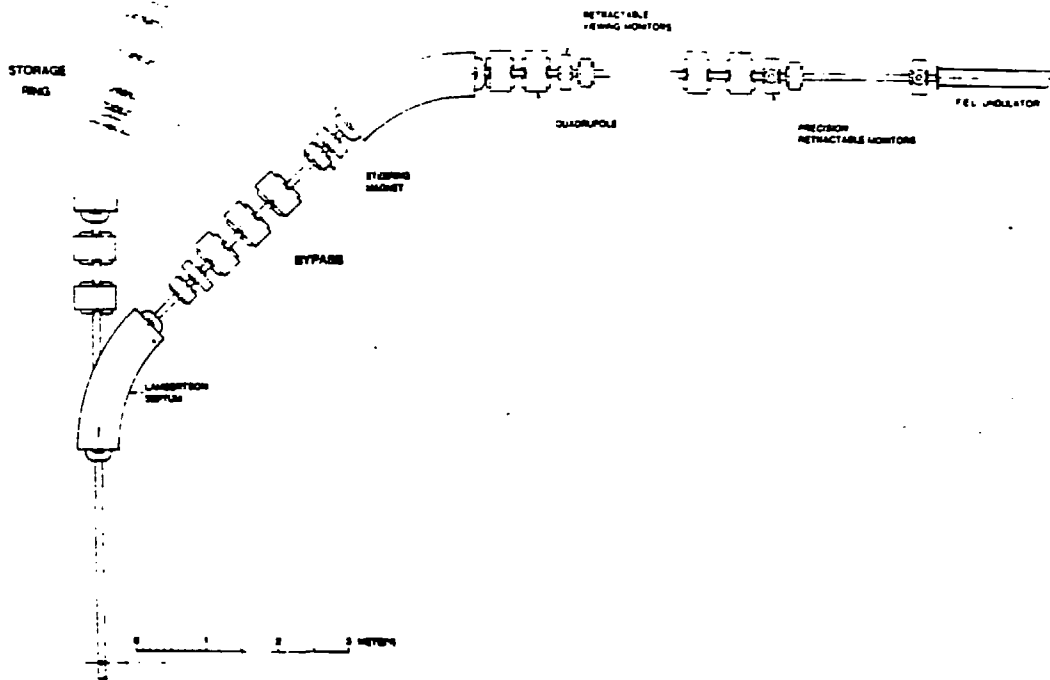
Fig. 5 Layout of the transfer line to the FEL undulator.
