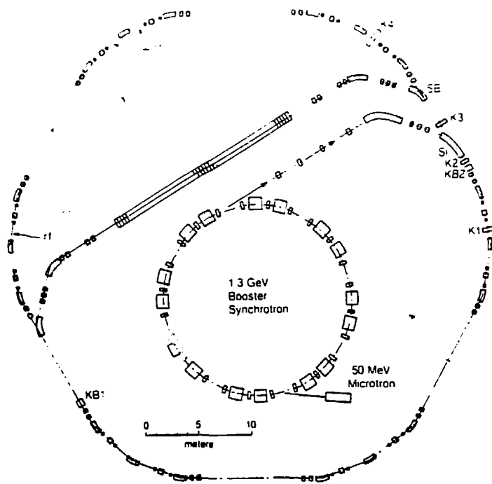
Fig. 3 Schematic layout of ring CF144 and bypass.
