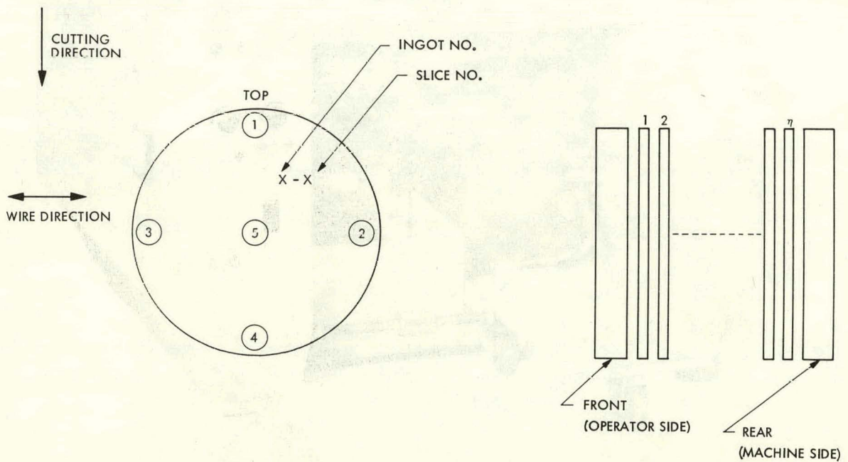
Figure 3. Location of thickness measurement on a wafer
