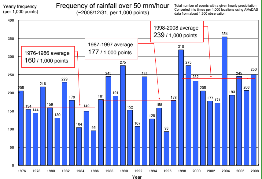
Annual number of events with \geq 50 mm hourly precipitation taken at AMeDAS observation stations (converted into number of events per 1,000 stations) Source: JMA, 2009
