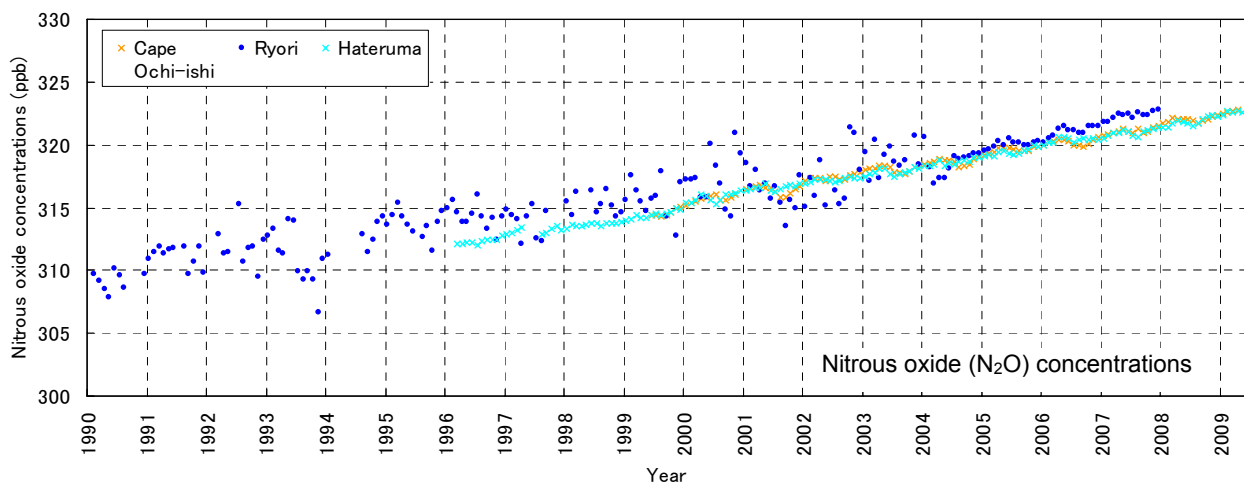
Fig. 2.4.4 Observed GHG concentrations in Japan
