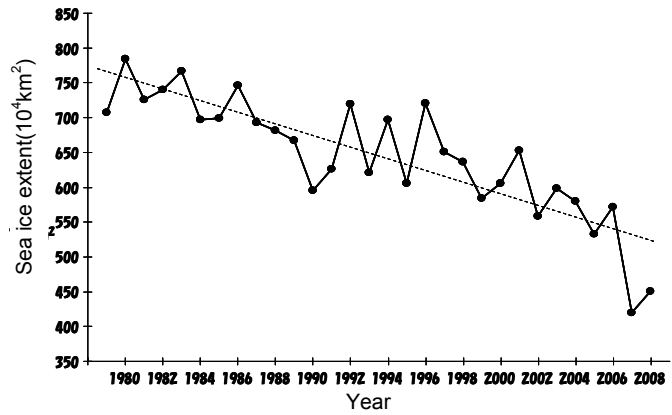
Annual minimum extent of Arctic sea ice from 1979 to 2008 (The dotted line shows a linear trend.)
