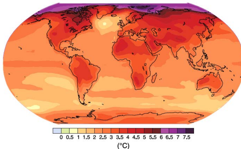
Fig. 3.2.4 Projected surface temperature changes for the late 21 st century (2090-2099)
