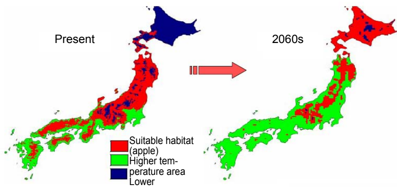
Fig. 4.1.10 Shift in areas suitable for growing apples Results are for a temperature rise of about 3°C by the 2060s, relation to the temperature in 1980. Source: Sugiura & Yokozawa, 2004
