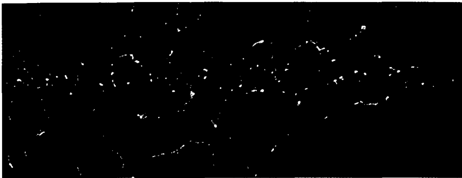
Figure 5. This historical photograph, published in 1923, shows the tracks made by electrons that have been hit by a narrow beam of x-rays. The x-rays pass through very moist air striking electrons in their path. These electrons speed off leaving a trail of electrically charged particles. Each
