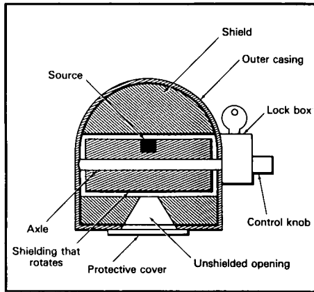
Figure 4. Diagram of a beam-type camera shown in safe (closed) position.
