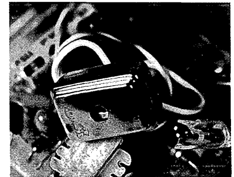
Figure 15. A neon bulb used for voltage regulation in this audible-alarm dosimeter has broken because it was dropped.
