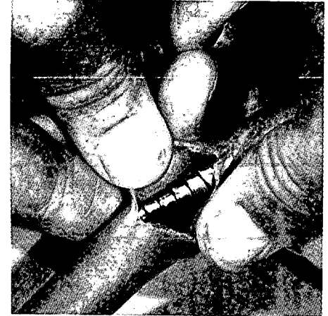
Figure 10. This guide tube has been crushed. A source can get stuck here. The guide tube must be repaired or replaced.
