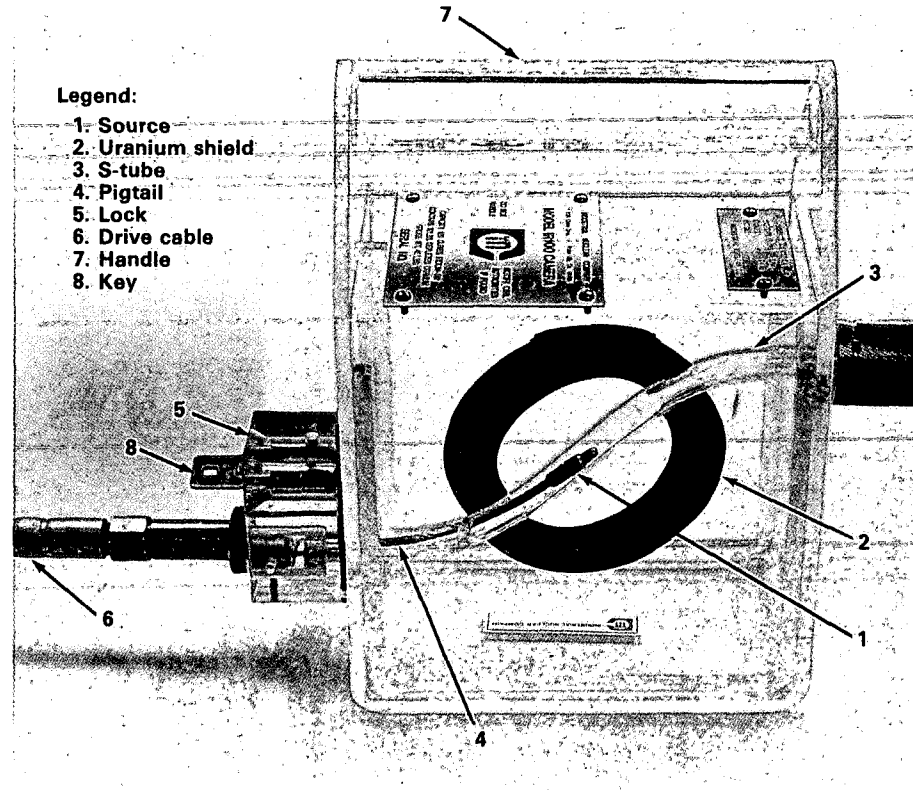
Figure 1. Demonstration model of a portable crank-out camera for iridium-192.
