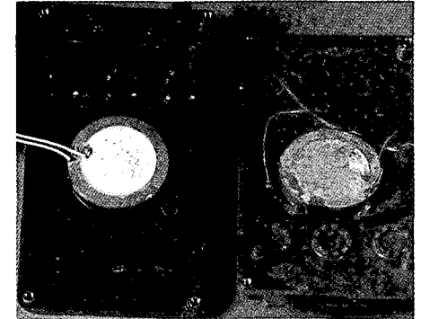
Figure 14. The audible-alarm dosimeter on the right has a ceramic speaker that was broken when dropped. The audible-alarm dosimeter on the left shows the speaker intact.
