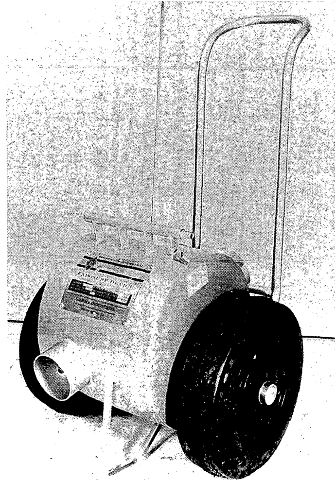
Figure 3. A mobile camera for 200 curies of cobalt-60. This camera weighs 475 pounds.
