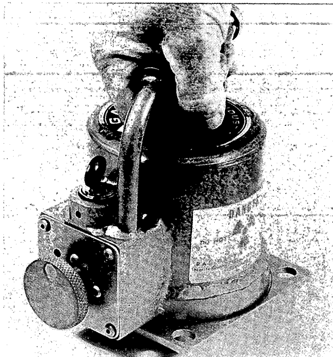
Figure 5. A beam-type camera for iridium-192. It operates using the knob in front or a drive cable that attaches to the handle.
