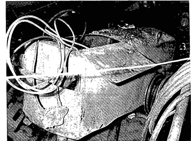
Figure 7. A fire in a factory destroyed this cobalt-60 camera. The tires burned off and the crank melted, but the shielding was undamaged. There was no radiation hazard.
