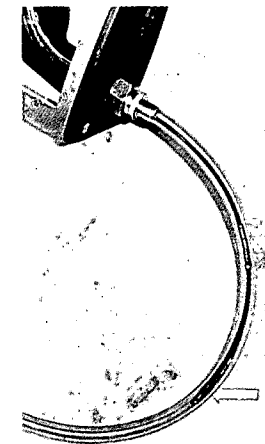
Figure 1. A dummy camera with transparent sides and guide tube is used here to show the position of an incompletely retracted source. The arrow shows the location of a source near the entrance to the S-tube. While disconnecting the guide tube, you can experience a particularly severe overexposure to your hands because they will be so close to the source.
