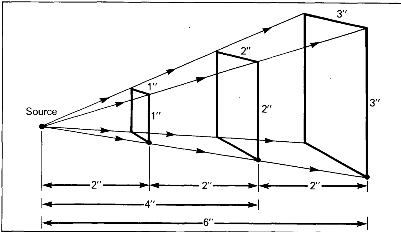
Figure 5. Inverse square law concept.
