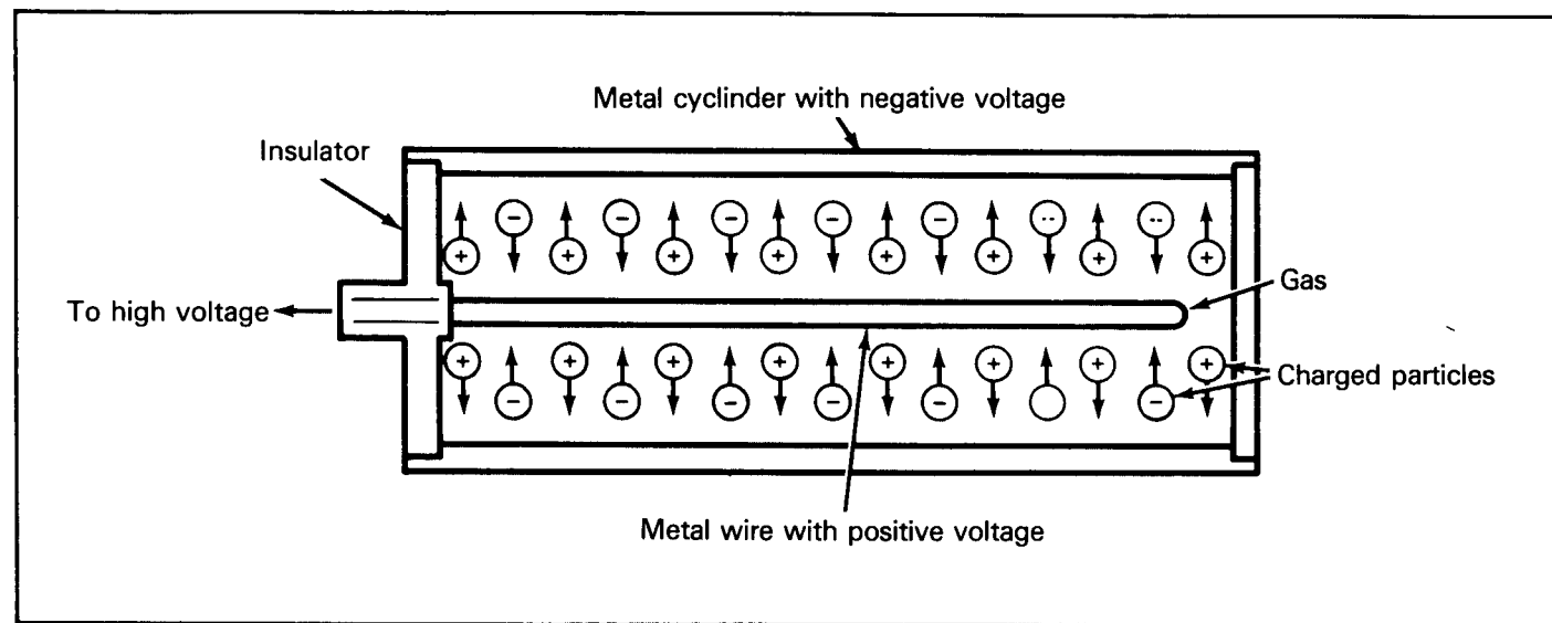
Figure 1. Cross section of a gas-filled radiation detector. Figure 5 in Chapter 2 showed charged particles produced by radiation in gas. The charged particles will be attracted to materials with an opposite charge. Movement of charged particles is an electric current. The electrical circuit of the instrument measures the current. The amount of current is read on the dial of the survey meter.
