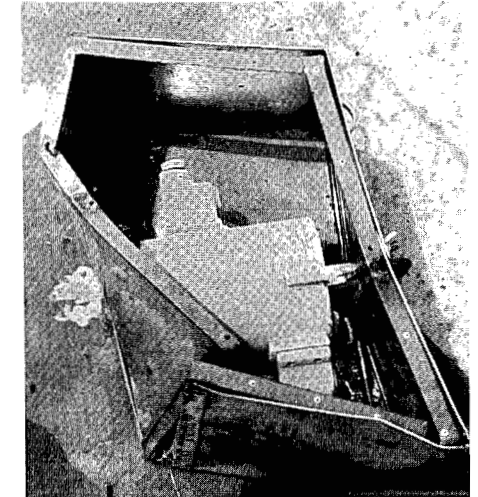
Figure 5. Camera in overpack after the impact. The source remained fully shielded.
