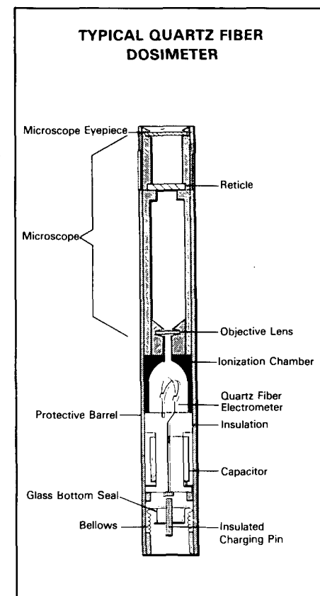
Figure 9. Cross section of a self-reading pocket dosimeter.
