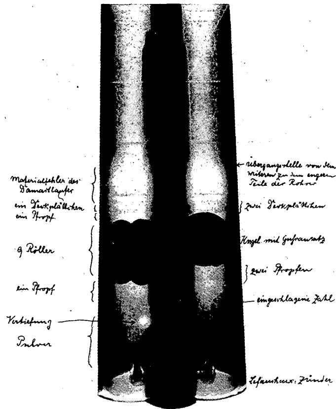
Figure 3. This radiograph of Roentgen’s shotgun is the earliest industrial radiograph (1896). This radiograph shows erosion in the barrels. Exposure time was 12 minutes.
