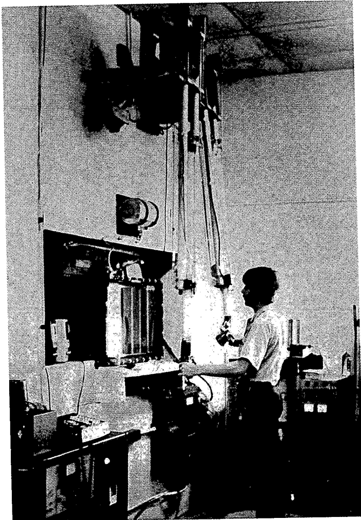
Figure 14. Several feet of heavy concrete shielding and glass containing lead are used to shield enclosures where radiography sources are manufactured. The operator uses master-slave manipulators to weld together the steel capsule containing the radioactive material.
