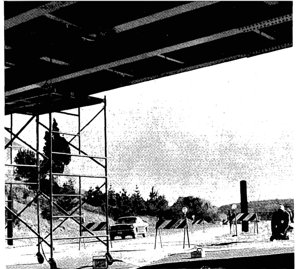
Figure 16. Radiography on a highway overpass.
