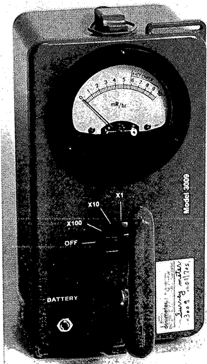
Figure 2. G-M survey meter with 3 ranges: 0-10 mR/hr, 0-100 mR/hr, and 0-1000 mR/hr.
