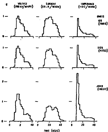
Fig. 6. Online waveforms from 157,000 shot run.
