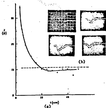
Fig. 2. a. Impedance waveform 17,000 shot run. b. Voltage (left, 160 kV/div.) and current (right, 8 kA/div.), 20 ns/div.
