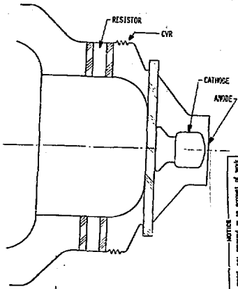
Fig. 1. Diagram of the RTF-I diode.
