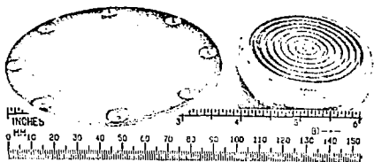
Fig. 5. Anode (left) and cathode for 157,000 shot run.
