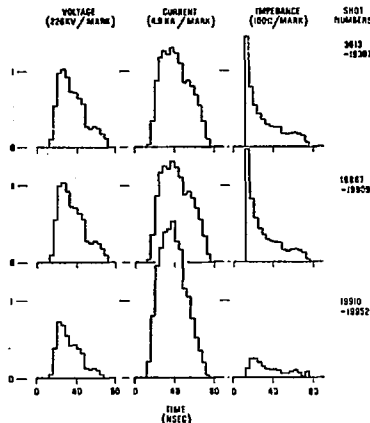
Fig. 4. Computer waveforms from 20,000 shot run.
