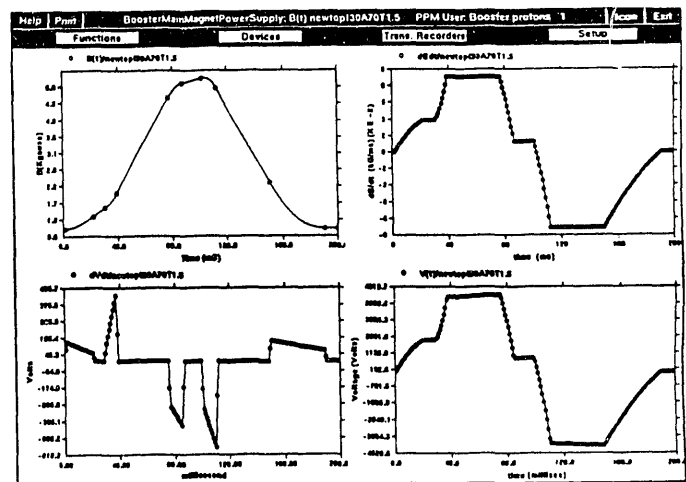
Figure 2 - MMPS program view of several B(t) related functions allows the User to verify they are as required for the cycle.
