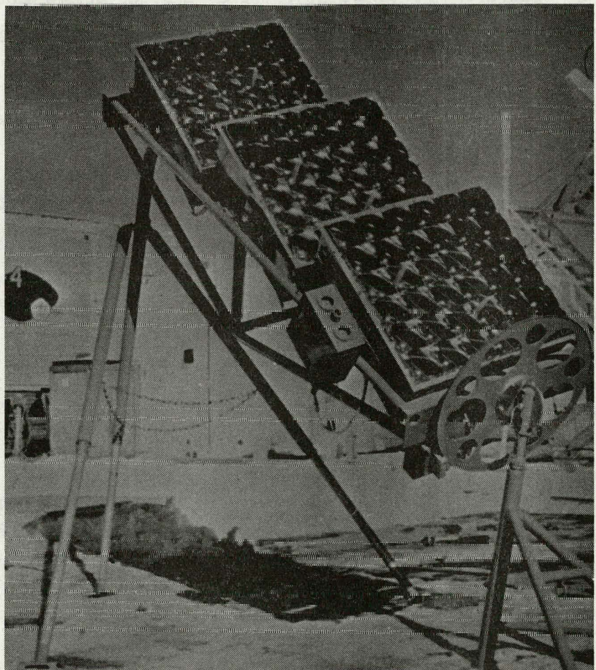
Fig. 32. Close up of the GaAs cells in the Varian, 1 kW system.
