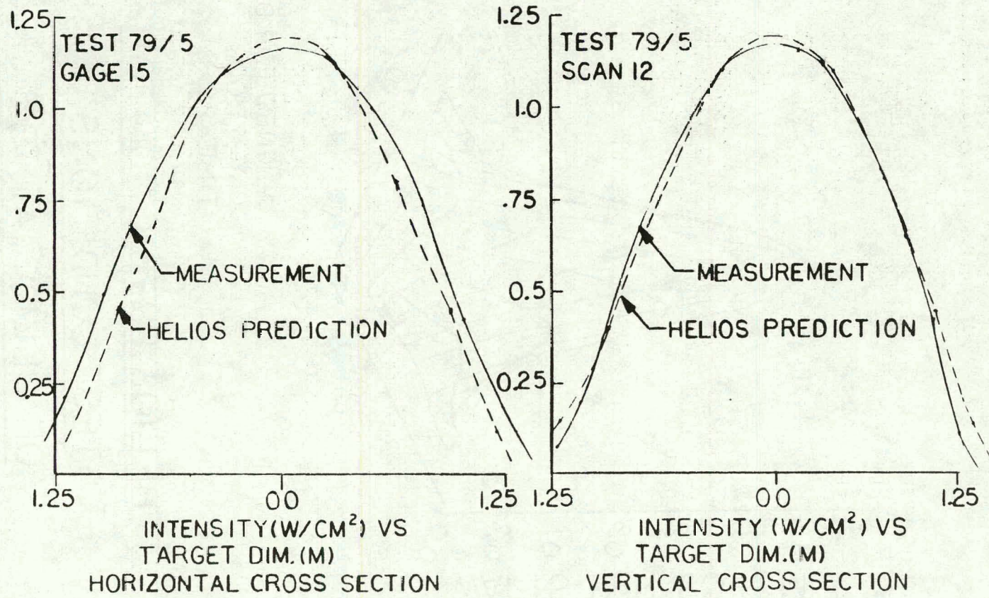
MEASURED VS. PREDICTED BEAM SHAPE
