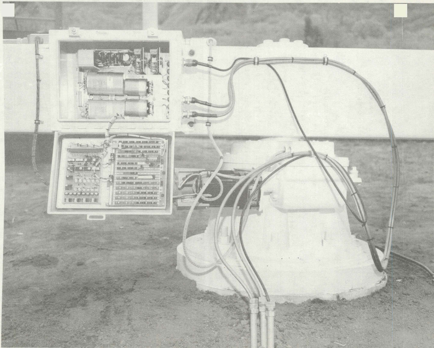
HELIOSTAT CONTROL ELECTRONICS UNIT
