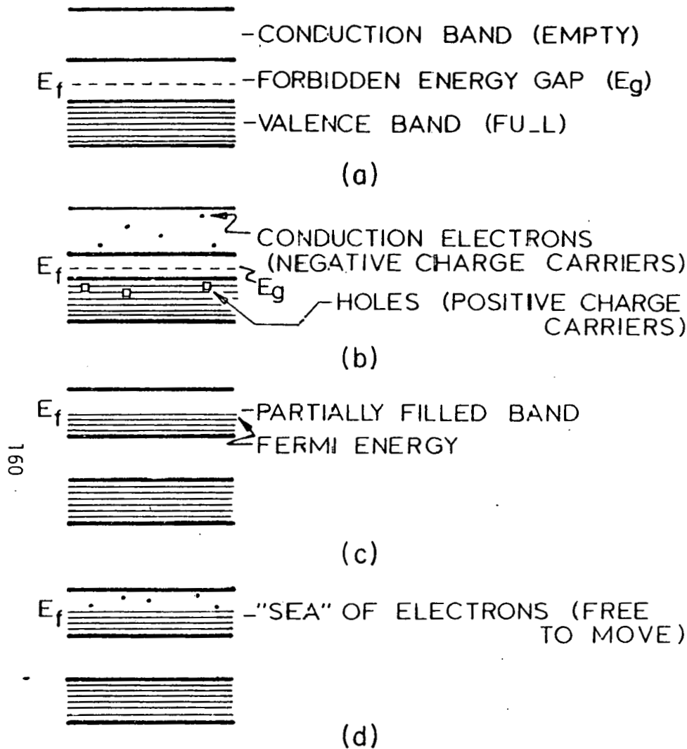
Fig. 1. One-dimensional energy band diagrams for different types of materials. (a) Intrinsic insulator or semiconductor at 0^\circ\text{K} ; (b) intrinsic semiconductor at T > 0^\circ\text{K} ; (c) metal or good conductor at 0^\circ\text{K} ; (d) conductor at T > 0^\circ\text{K} .
