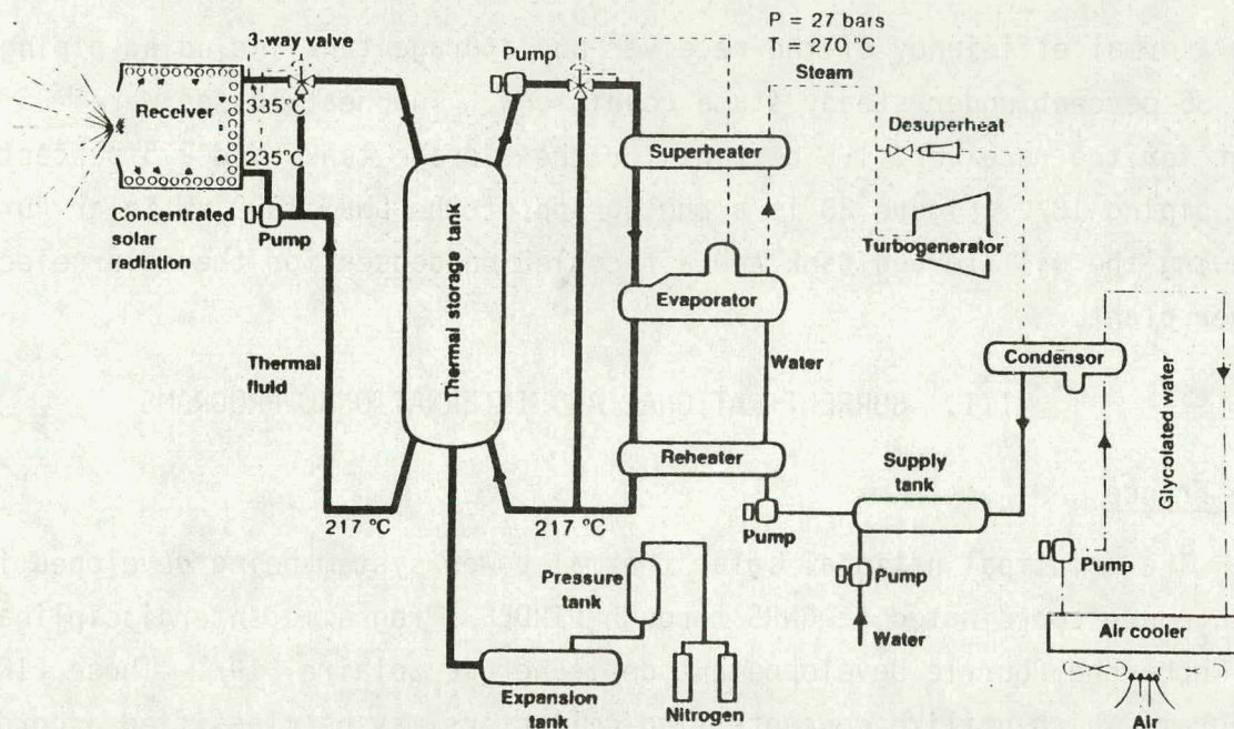
Figure 27. Schematic of Solar Thermal Power Cycle Using Oil Cooled Receiver at CNRS 1000 kW Solar Furnace, Odeillo, France.
