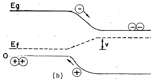
Fig. 10. (a) a typical current-voltage curve for an ideal solar cell with the short circuit approaching the constant light-generated current J_L . The maximum power point is shown as P_{max} . (b) A typical electron energy diagram for a p-n junction under illumination of sunlight with the external resistance set such that the output voltage is at value V . This same voltage V is thus imposed on the junction which will reduce the current delivered to the external load.
