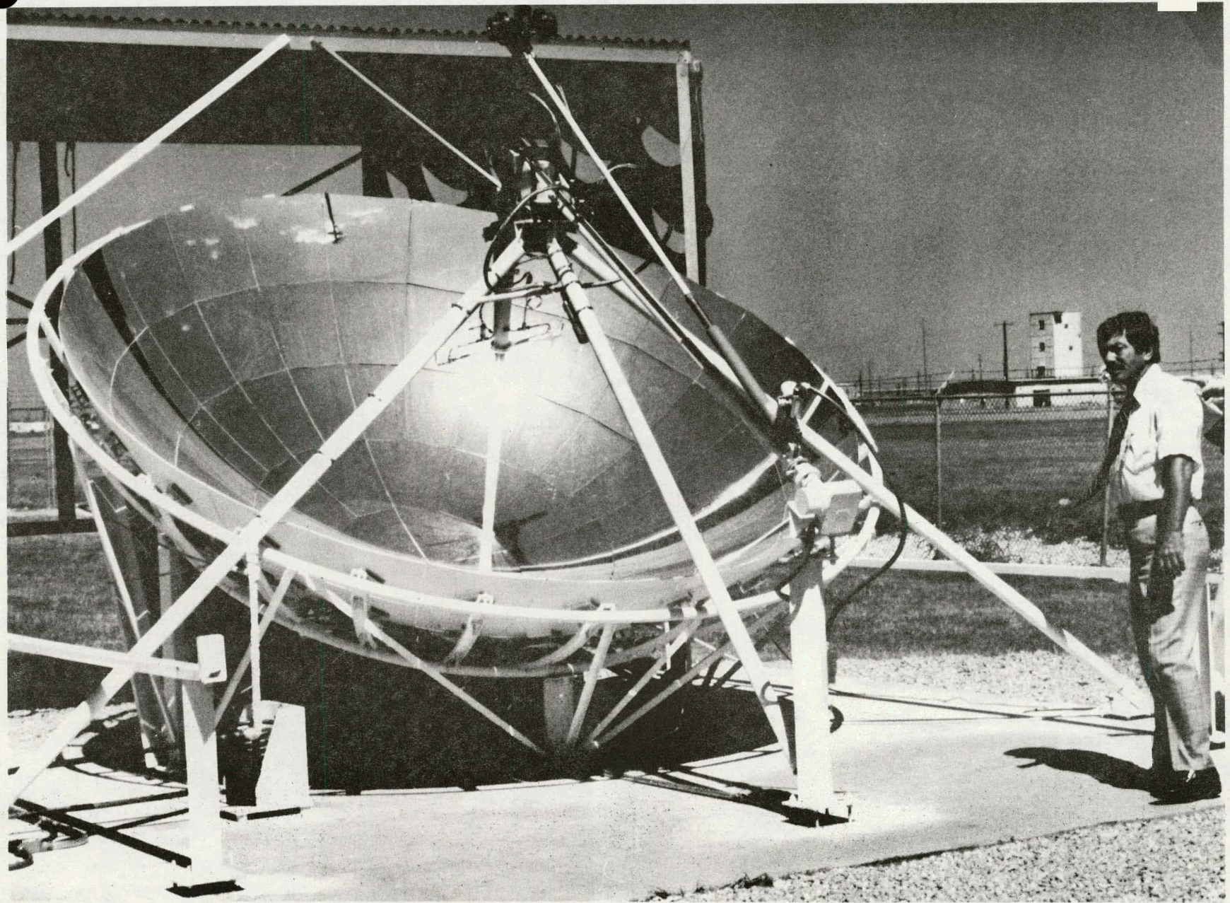
Figure 21. Prototype of Fixed-Mirror Distributed Focus Collector
