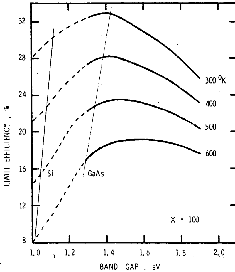
Fig. 17. Limit conversion efficiency at 100 AMI suns vs. bandgap and temperature. The straight lines represent the Si and GaAs bandgaps (23)
