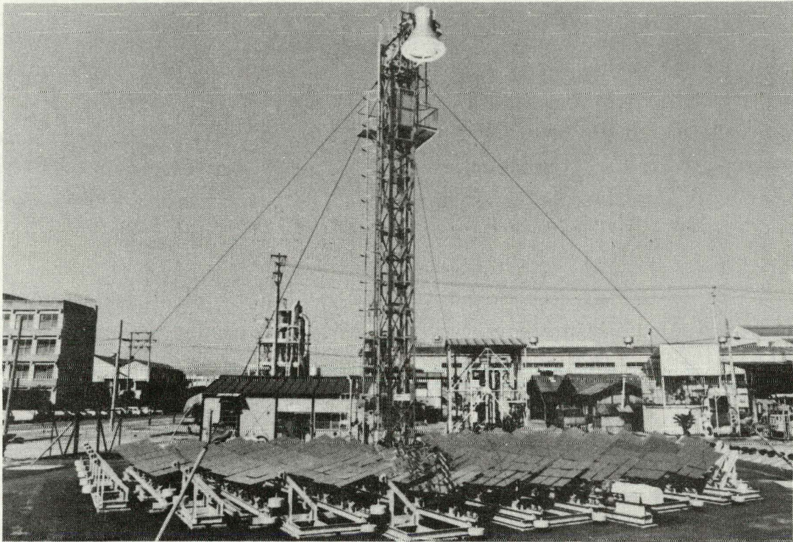
Figure 19. Central Receiver Test Facility Developed by Mitsubishi Heavy Industries, Hiroshima, Japan.
