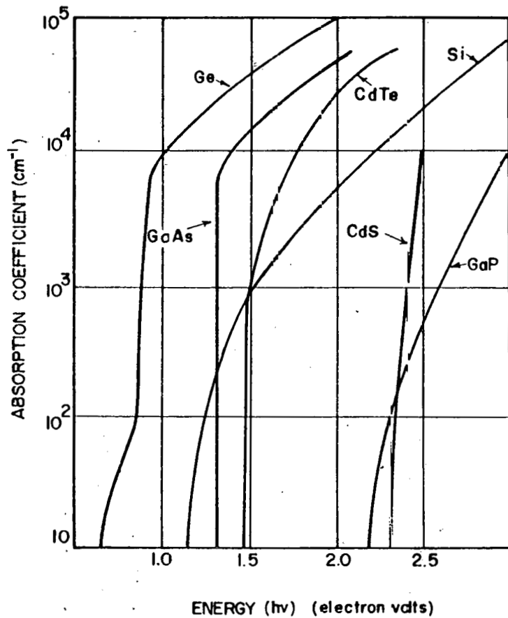
Fig. 5. The optical absorption coefficients as a function of photon energy for a number of materials of interest for solar cells. Materials having steep curves (sharp absorption edges) are indicative of direct absorbers and could be made into thin film solar cells.
