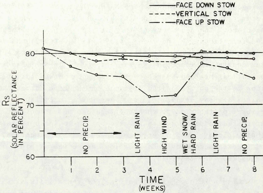
REFLECTIVITY VS. TIME FOR DIFFERENT STORAGE ORIENTATIONS IN STTF HELIOSTAT FIELD
