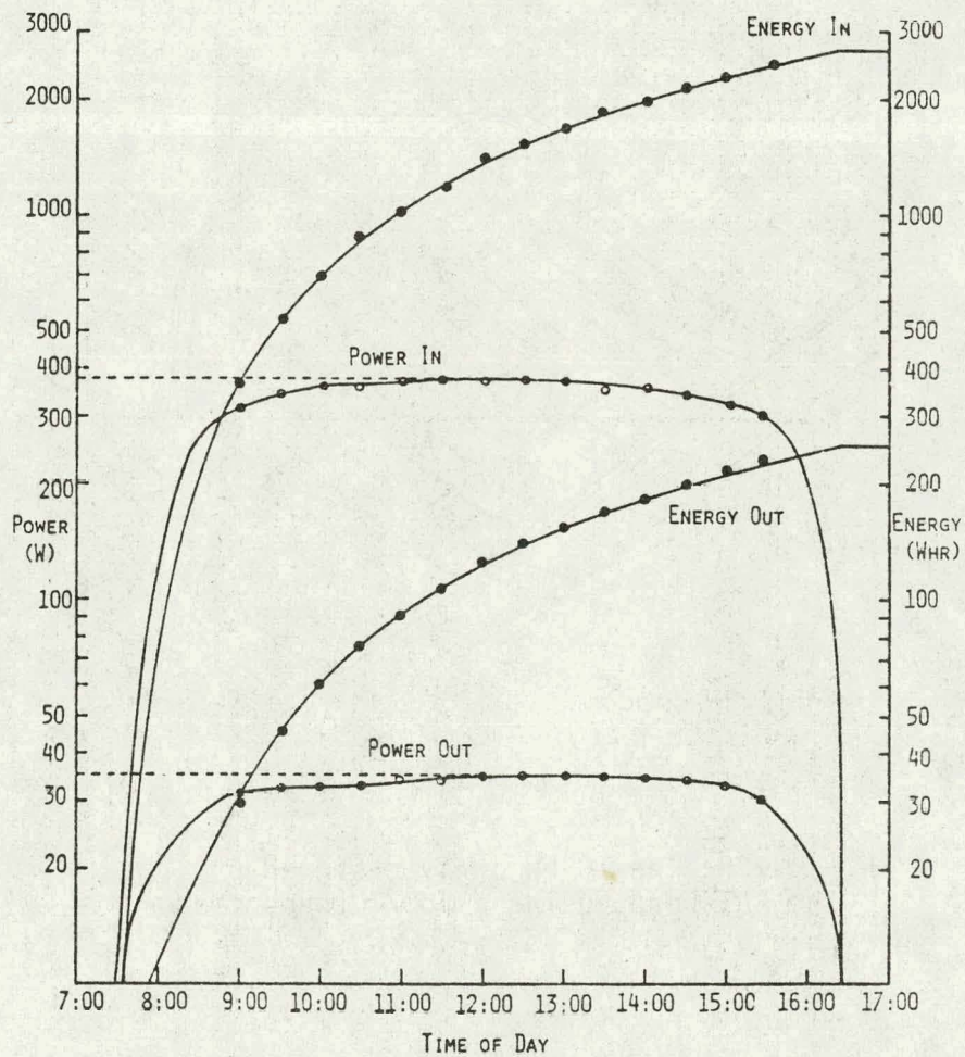
Fig. 37. Martin Marietta module performance test results.
