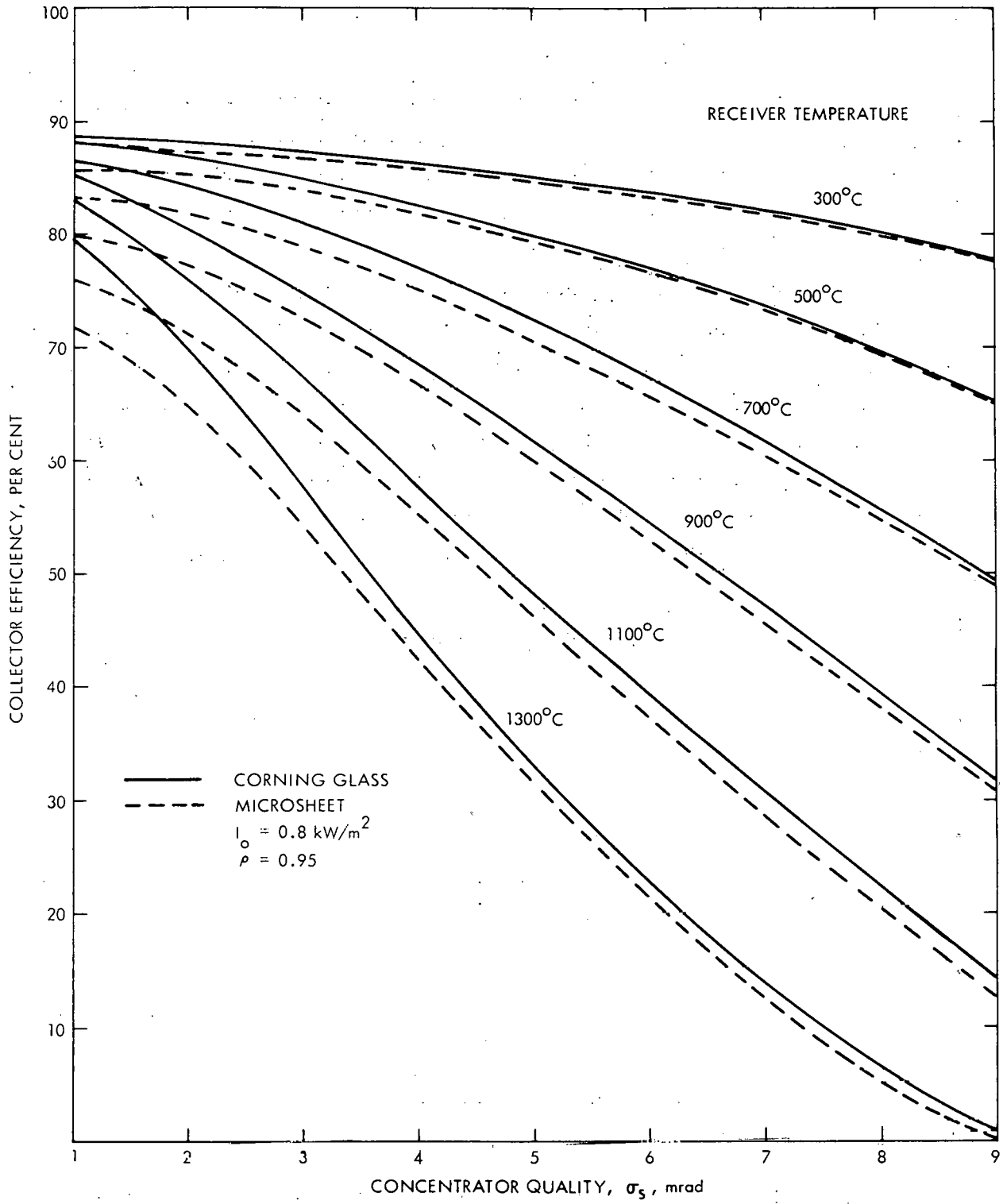
Figure 8. Collector Efficiency
