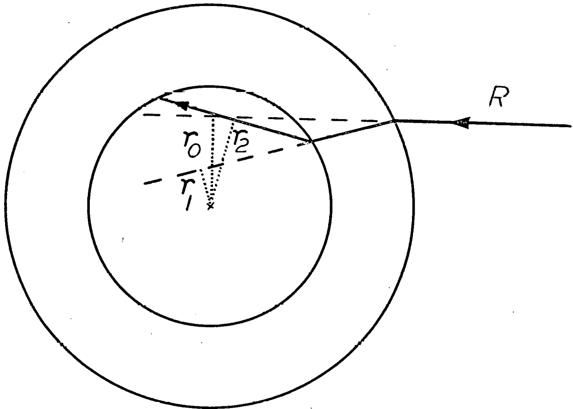
Fig. 4. Refraction of light ray by glass tube. The impact parameters r_0 and r_2 are equal.
