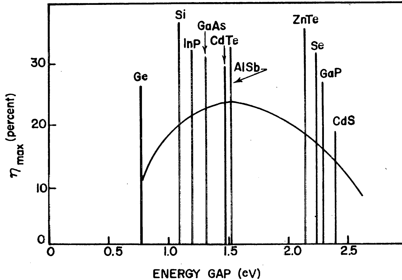
Fig. 11. A calculated curve of the maximum efficiency that can be obtained as a function of the energy gap of the semiconductor made into a p-n junction and illuminated with the solar spectrum outside the atmosphere, AMO (Loferski, 1963).
