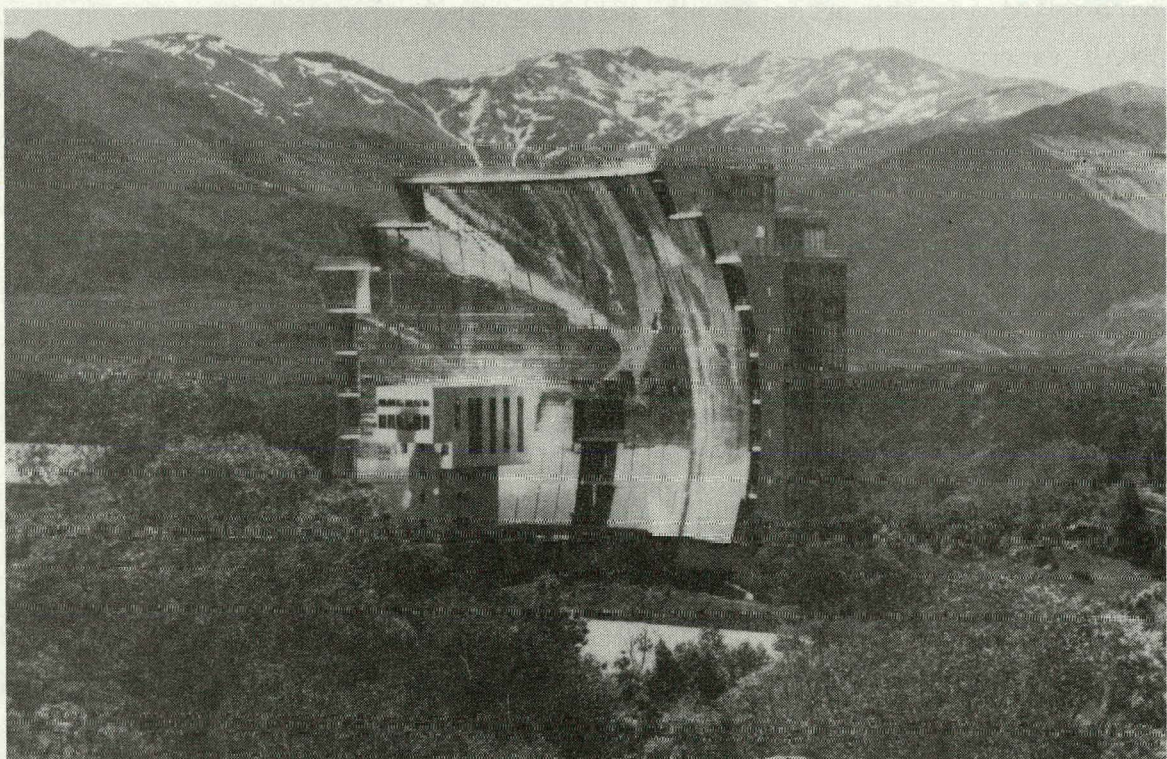
Figure 8. Paraboloid Concentrator of CNRS 1000 kW Solar Furnace at Odeillo, France.
