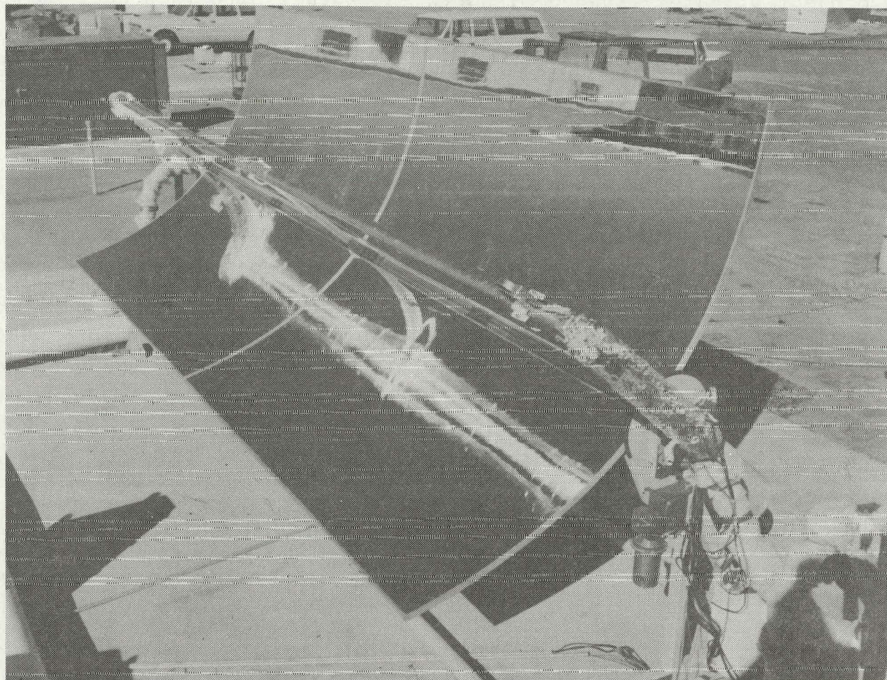
FIGURE 4. Hexcel Parabolic Trough Collector
