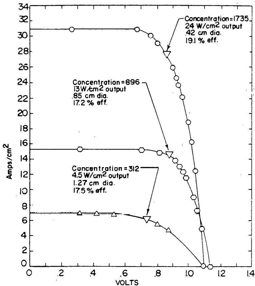
Fig. 26. Current-voltage curves for a GaAs concentration cell made and tested by Varian Assoc. (26)
