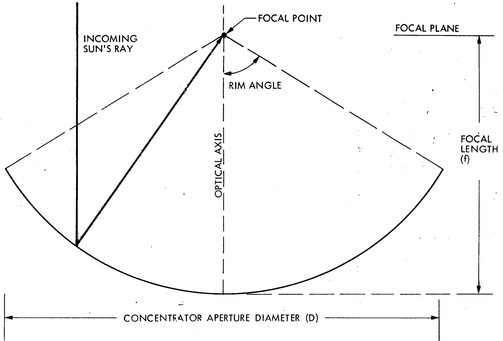
Figure 1. Concentrator Optics
