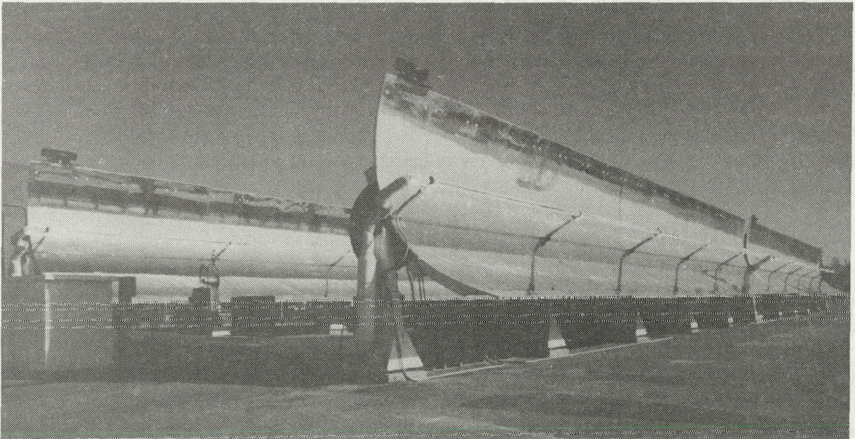
FIGURE 11. Sandia Parabolic Trough Collector Field
