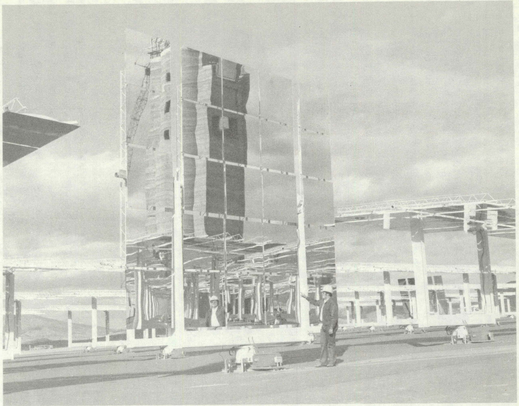
STTF HELIOSTAT IN VERTICAL POSITION
