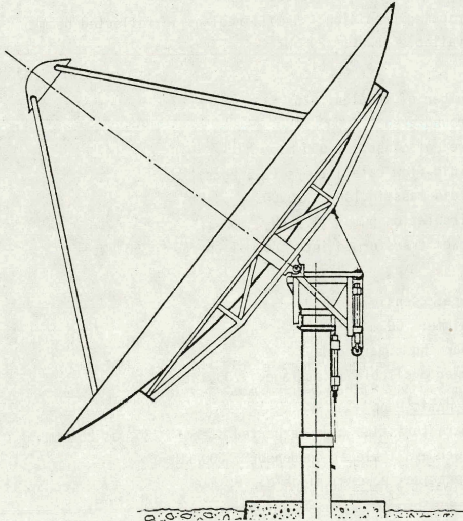
Figure 31. Concentrating Collector-Receiver Design Being Developed for THEK System.
