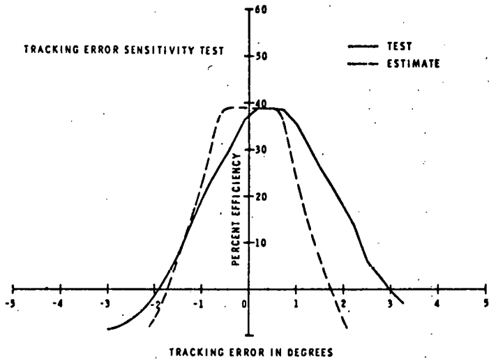
Tracking Error Sensitivity Test, Northwest Quadrant
