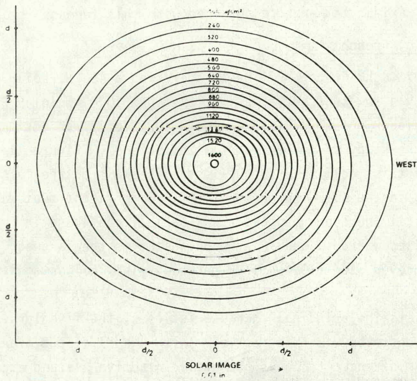
Figure 10. Heat Flux Contour Map of the CNRS 1000 kW Solar Furnace.
