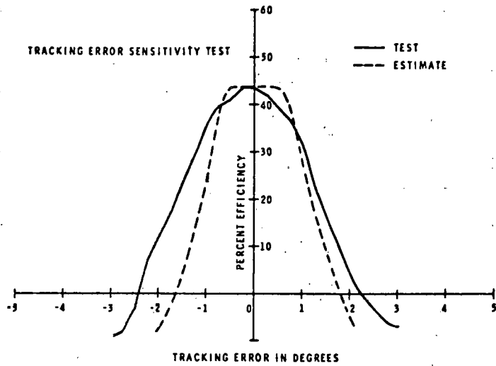
Tracking Error Sensitivity Test, Southwest Quadrant
