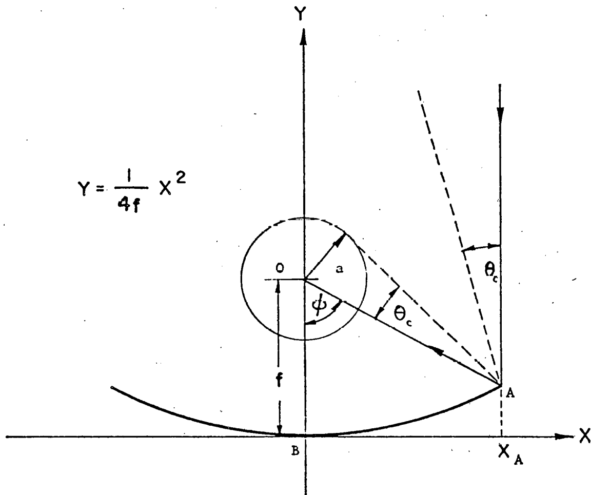
Fig. 1. Focusing parabola
