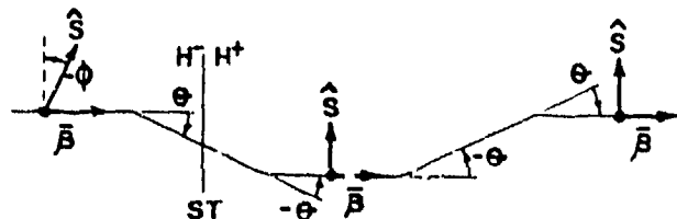
Fig. 2 - Schematic of the bends required to produce a polarization precession of \phi in the horizontal plane.
