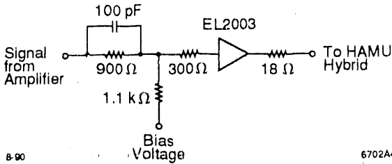
Fig. 4 Schematic of one of the four channels of the buffer hybrid.
