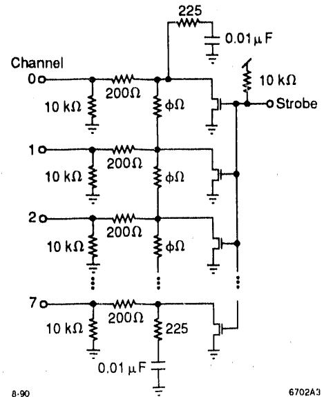
Fig. 3 Schematic of the leakage current sense pc board. The 0 \Omega (jumpers) and 225 \Omega resistors are not loaded for the central drift chamber. The resistor values are chosen for optimum resolution and settling time of the signal under the power pulse conditions for the preamplifier hybrid.
