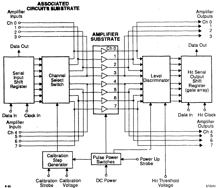
Fig. 2 Block diagram of the drift chamber preamplifier hybrid. Calibration and digital hit readout circuitry are included as well as logic to turn on the power.
