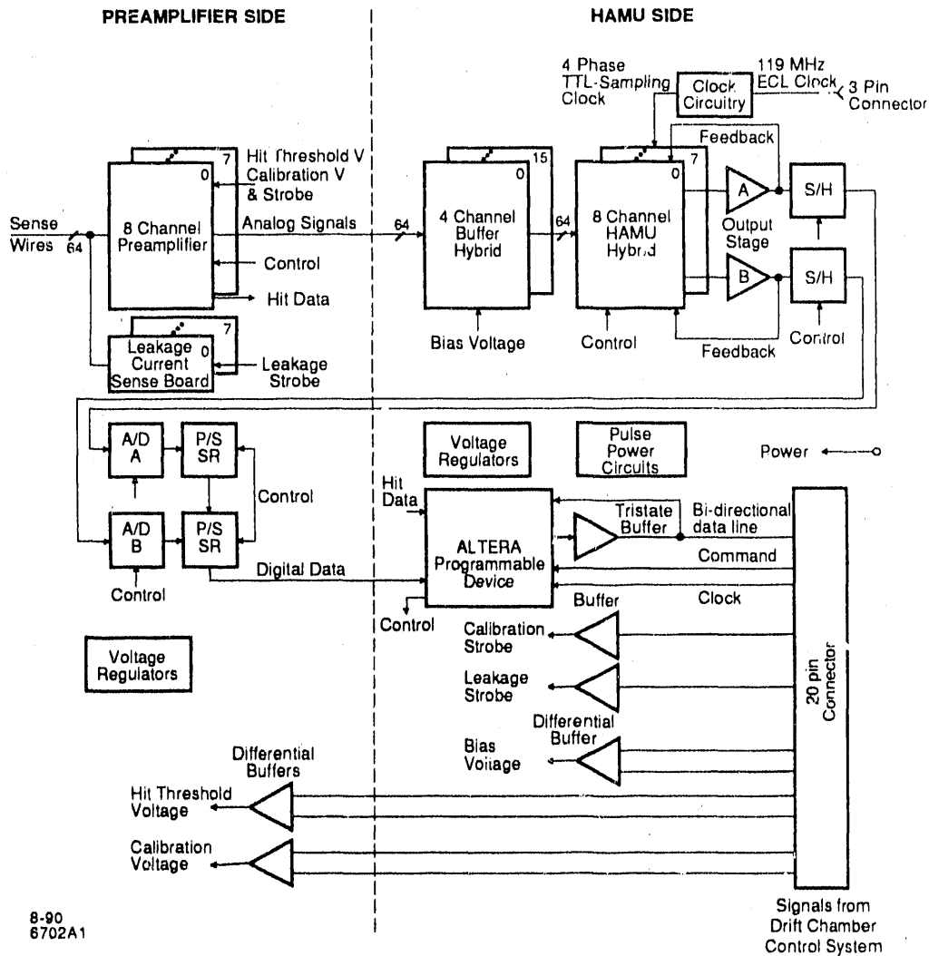
Fig. 1 Block diagram of the drift chamber motherboard. The side of the board facing the chamber is indicated as preamplifier side.
