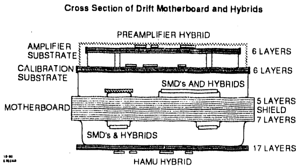
Fig. 9 Cross section of the CDC or EDC drift motherboard showing the two levels of surface mount components on both sides of the board.
