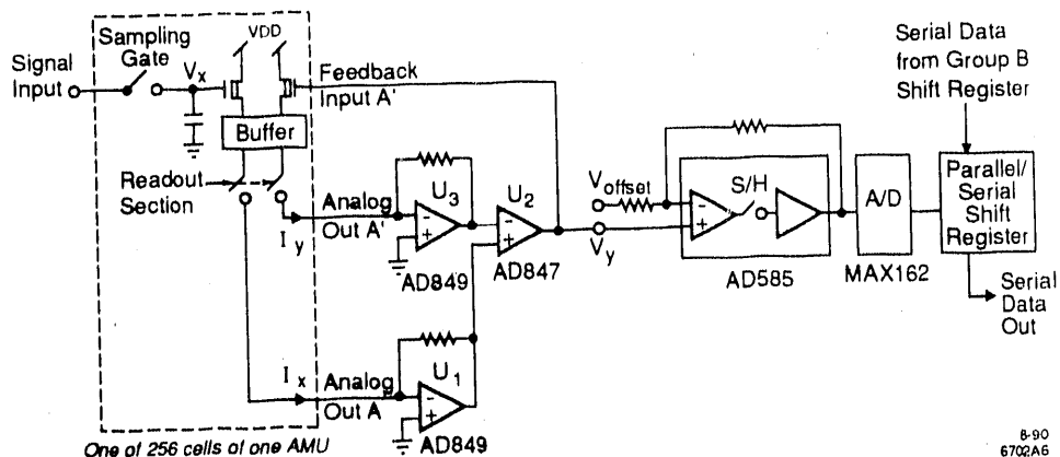
Fig. 6 Schematic of one of the two output stages on the motherboard. The outputs of 8 AMU chips are connected to one set of output buses. Shown is only one cell of one AMU.
