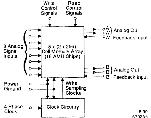
Fig. 5 Block diagram of the HAMU sampling and storage hybrid.
