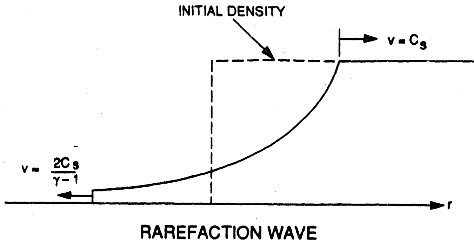
Figure 1 shows the classical rarefaction wave that progresses within the fluid at sound speed and reverses the flow. The maximum velocity of blow off from a rarefaction wave is 2C_S/(\gamma-1) .
