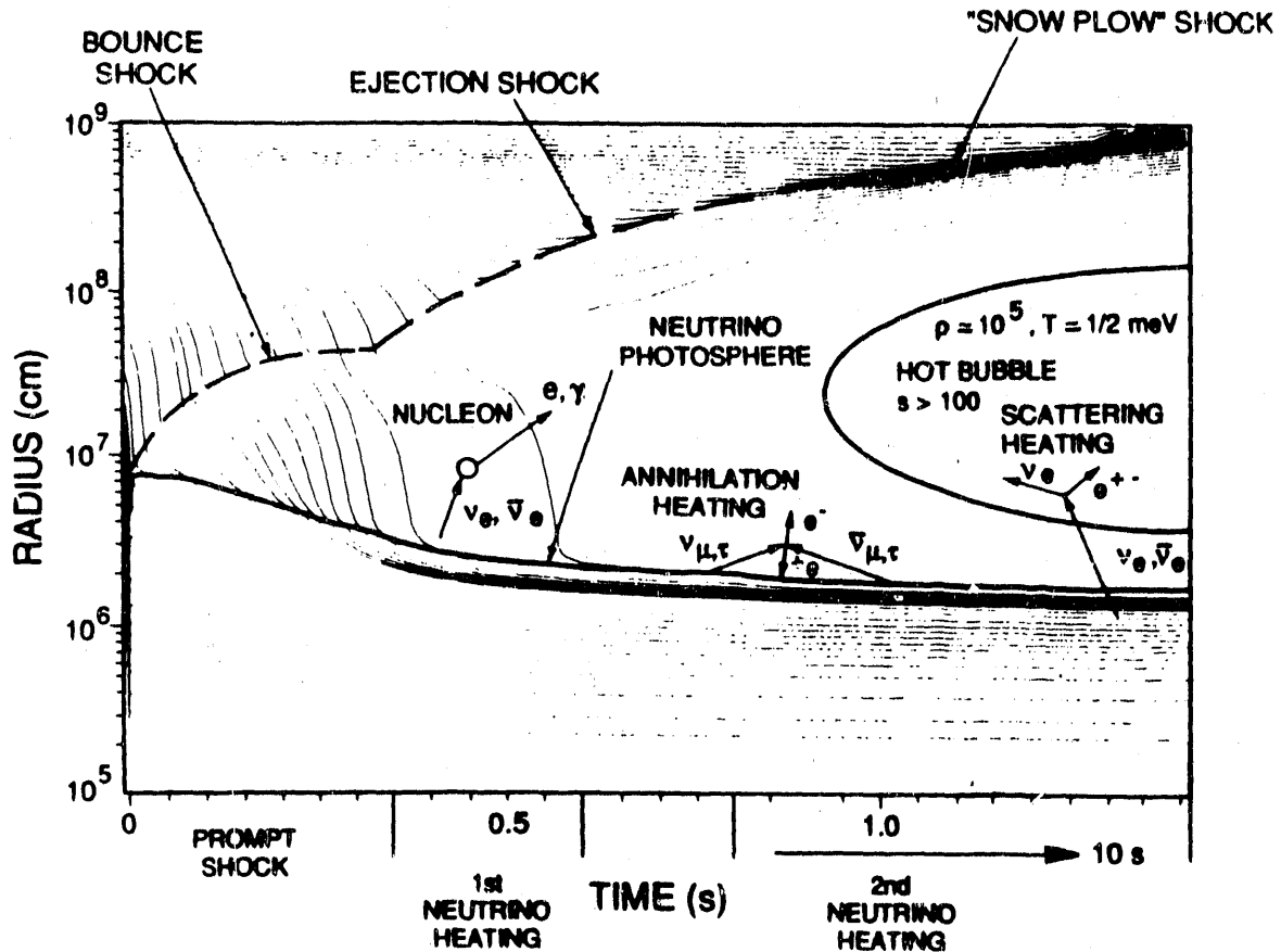
Figure 2. The sequence of processes occurring in a Type II supernova according to Wilson and Mayle.(1989). First a star collapses, owing to exhaustion of the fuel and emits electron neutrinos as the compressing matter turns into neutron-rich matter. The forming neutron star bounces producing a strong shock that weakens owing both to the thermal decomposition of the infalling nuclear matter and the reversal of the neutron star bounce trajectory. Subsequently, a large burst of neutrinos of all flavors heats the infalling matter, starting an explosive shock. Yet later, mu and tau neutrino-antineutrino annihilations in nearly opposed collisions just above the neutrino photosphere generate heat without nucleonic matter, making a hot, high-entropy ( 10^4 Boltzmann-units) bubble, which pushes out the ejected matter in a thin "snow plow" shock. The pressure is maintained because the high-entropy ensures a large scale height adjacent to the neutron star.
