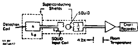
Fig. 10. Schematic of a typical induction detector.
