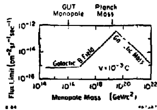
Fig. 16. Parker limit on cosmic ray GUM flux as a function of monopole mass. The information in this figure is extracted from Ref. 37. The estimated GUT mass of 10^{16} GeV/c 2 and the Planck mass of 1.22 \times 10^{19} GeV/c 2 , ( \hbar c/G ), where G is Newton's gravitational constant, are also indicated. The velocity v = 10^{-3}c is typical of what one might expect for cosmic monopoles. The shape of the curve will vary somewhat with velocity.
