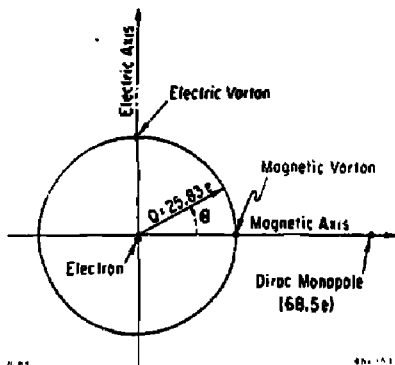
Fig. 4. Generalised electromagnetic charge plane with electric and magnetic vortons, a Dirac monopole, and electron indicated.
