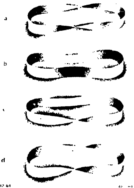
Fig. 5. Topological charge illustrated by Möbius strips.
