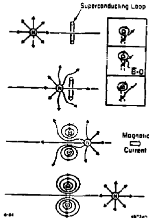
Fig. 9. Principle of induction technique, after Cabrera. 28
