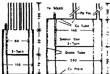
Fig. 19. Schematic depictions of the KOBE I, and KOBE II detectors, furnished by T. Watanabe.
