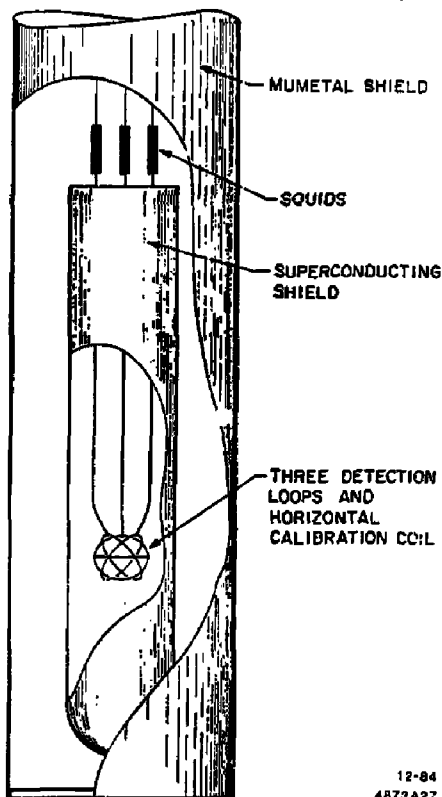
Fig. 11. Present Stanford monopole detector apparatus. 23
