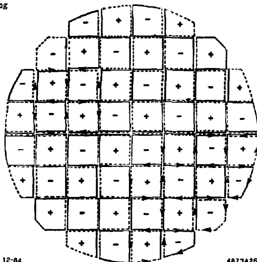
Fig. 13. Macramé gradiometer pattern, taken from Ref. 32.
