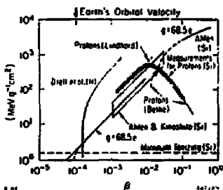
Fig. 25. Energy loss by ionization (See text).
