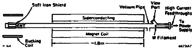
Fig. 20. SLAC monopole accelerator and detector.
