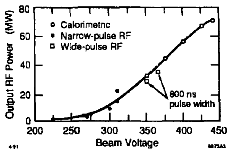
Figure 3. XC2 Output Power.
