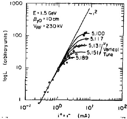
Fig. 11. SPEAR I data that show tune and beam intensity dependences of luminosity.
