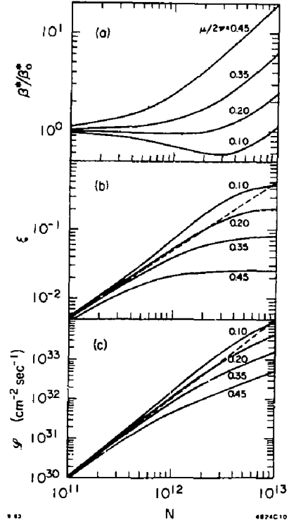
Fig. 10. Dynamic-beta behavior of \beta^* , \xi and L . \mu/2\pi is the unperturbed tune advance between collision points (modulus 1/2 ). The dashed lines in (b) and (c) are the reference values when dynamic-beta effect is ignored. We have chosen the normalization that L_0 = 10^{32} \text{ cm}^{-2} \text{ sec}^{-1} and \xi_0 = 0.05 at N = 10^{12} .
