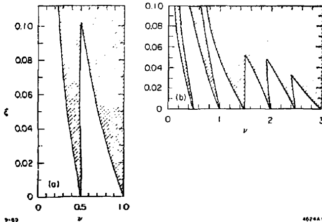
Fig. 17. Stability region for two strong beams executing small quadrupole oscillations. \nu is the total tune of the storage ring. The figures are periodic in \nu ; the periods are 1 in (a) and 3 in (b). A round beam at equilibrium has been assumed.
