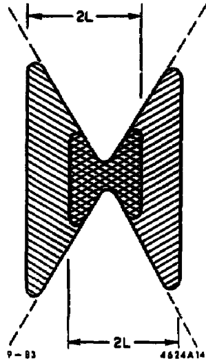
Fig. 14. Colliding beams when \beta^* is too small.
