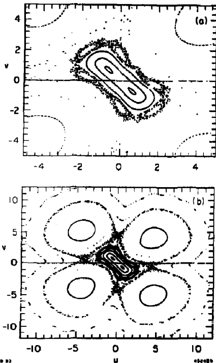
Fig. 9. Particle motion when the stochastic limit is exceeded. (b) is the same as (a) but with expanded scale. It could be misleading if we look only at (a).
