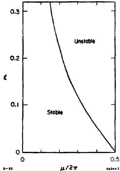
Fig. 2. Stability region for a weak beam executing small oscillations. \mu is the beta-tron phase advance between collision points. The diagram repeats with period \mu = \pi and shows a periodic sawtooth behavior which is typical of beam-beam models.
