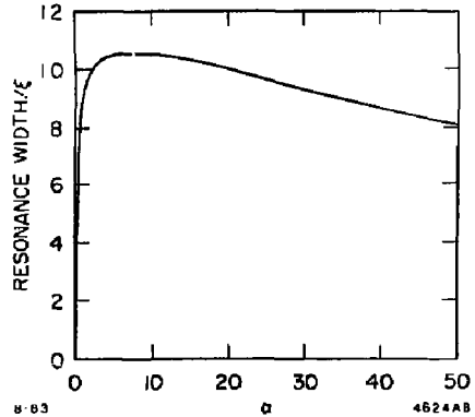
Fig. 8. The total beam-beam resonance width as a function of particle emittance.
