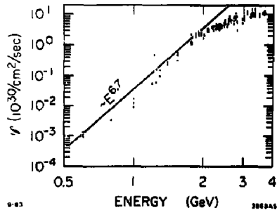
Fig. 10. Luminosity versus beam energy for the storage ring SPEAR.
