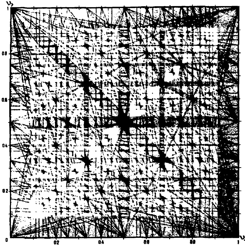
Fig. 18. Coherent instability region in the \nu_x, \nu_y space for the storage ring DCI. There is an instability when a resonance condition, Eq. (14), is met. The value of \xi is taken to be 0.05.
