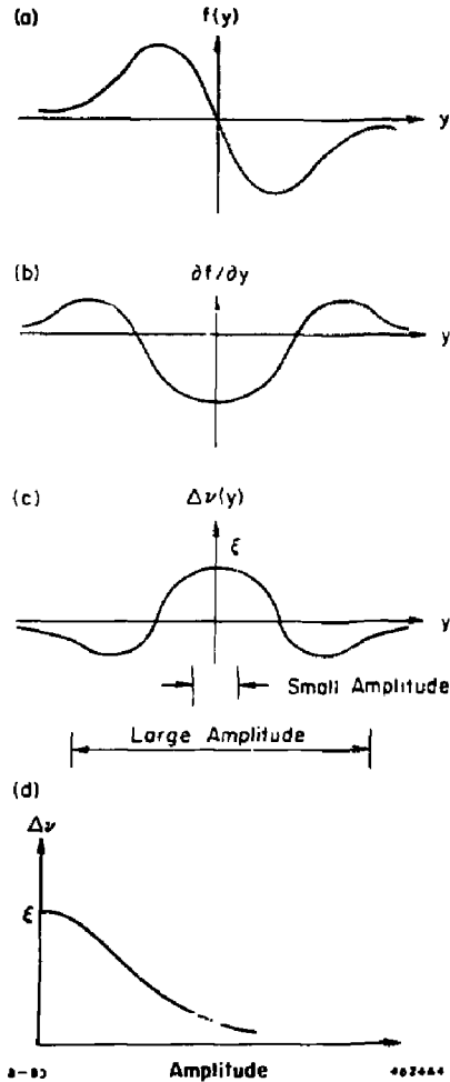
Fig. 4. Schematic illustration of the beam-beam tune shift mechanism. (a) shows the beam-beam force. (b) is the slope of this force. Before averaging, the tune shift is proportional to -\partial f/\partial y in such a way that \Delta\nu = \xi at the origin, as shown in (c). We then perform an averaging of this \Delta\nu(y) over the range reached by a given amplitude. (c) also shows two such ranges, one for a small amplitude particle and one for a large amplitude particle. The result after averaging gives the detuning curve which looks like (d).
