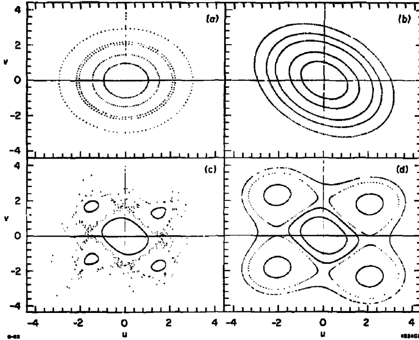
Fig. 3. Weak beam trajectories in the normalized phase space (u, v) , where u = y/\sigma , v = \beta_0^y y'/\sigma . We assume \mu/2\pi = 0.23 . (a) ignores the beam-beam force. (b) includes only the linear term of the beam-beam force. (c) includes the linear and the octupole terms and (d) takes into account of the complete beam-beam force. In each diagram, trajectories of the same five sets of initial conditions are followed. Note the qualitative difference between (c) and (d).
