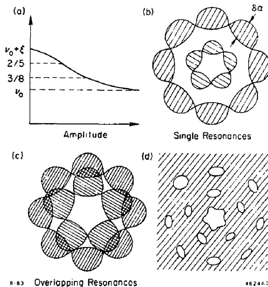
Fig. 7. Sketches of single-resonances and overlapping resonances. (a) is the detuning curve showing the tune spread is covering two single resonances. (b) shows two isolated separated single resonances in the phase space. (c) shows two overlapping resonances which actually end up looking more like (d). In (d), the shaded area represents the region of stochastic motion.
