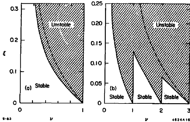
Fig. 16. Stability region for two strong rigid beams executing small center-of-mass oscillations for (a) two colliding bunches and (b) six colliding bunches. \nu is the total tune of the storage ring. The figures are periodic in \nu ; the periods are 1 in (a) and 3 in (b). The dashed lines are the strong-weak stability limit reproduced from Fig.2.
