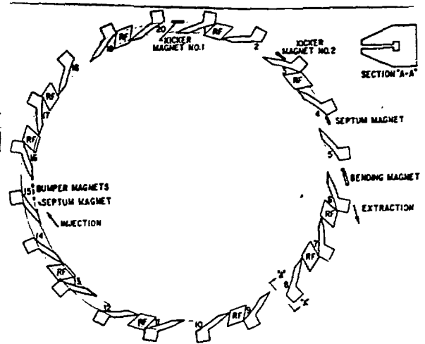
Fig. 1. Schematic View of the 1500-MeV FFAG.
