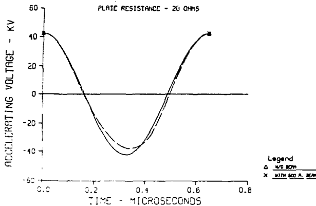
Fig. 3(a). Gap voltage waveforms with full loading and no loading with an amplifier impedance of 20 ohms.
