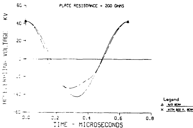
Fig. 3(b). Gap voltage waveforms with full loading and no loading with an amplifier impedance of 200 ohms.
