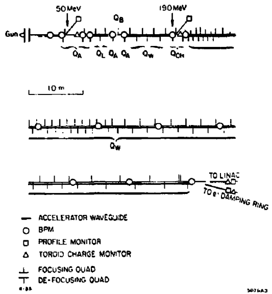
Fig. 1. SLC 1.2 GeV high current injector showing waveguide, focusing magnet and diagnostic instrument locations.
