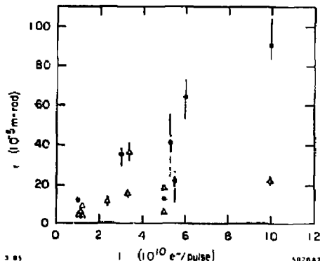
Fig. 4. Horizontal and vertical emittance data at the end of the SLC injector for different beam currents. The points at 10^{11} e^- represent the superimposed emittance of the bunch pair.
