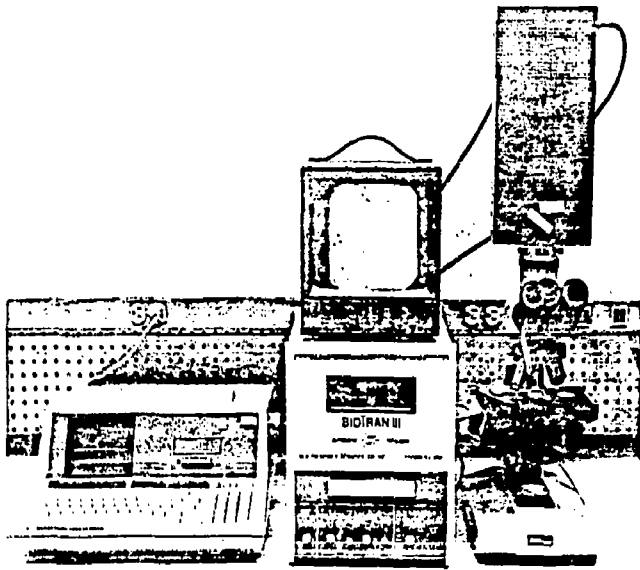
Figure 2. Bacterial colony counter for measurement of track density on CR-39 and polycarbonate, together with desk top computer.
