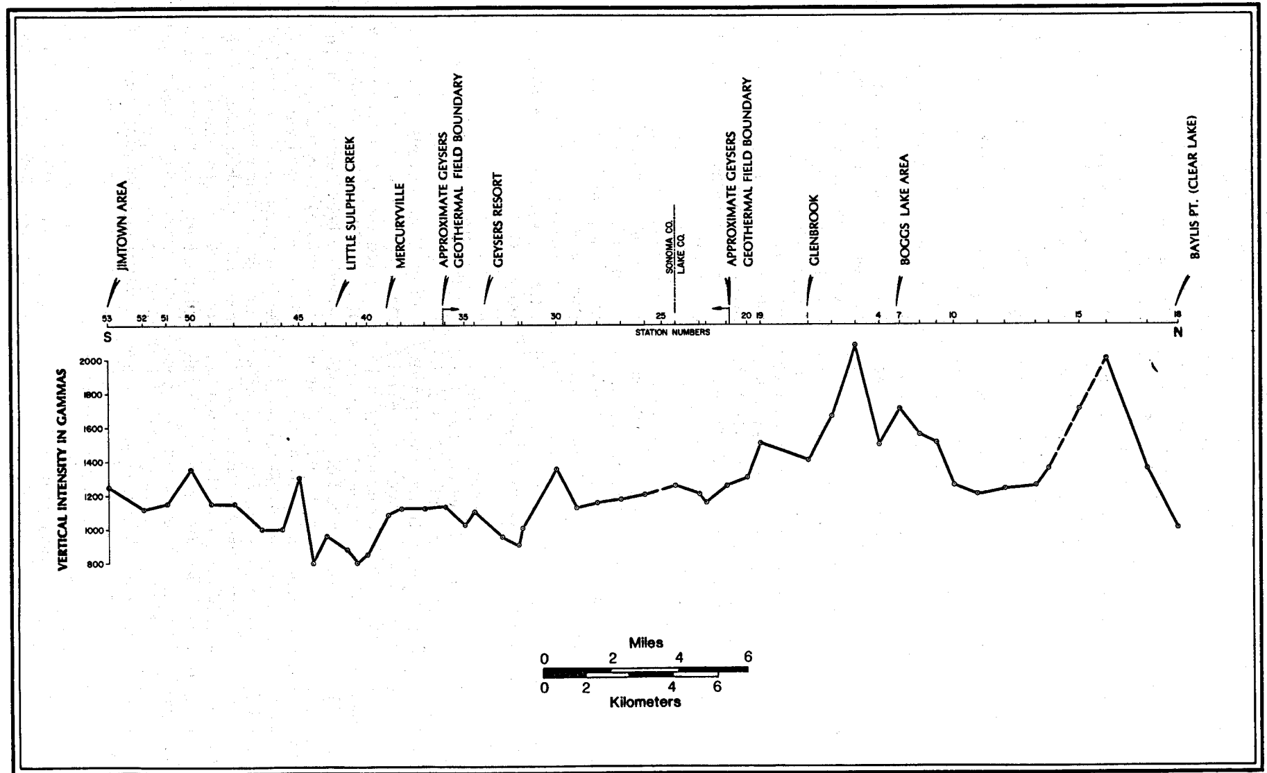
Figure 10. Ground magnetic traverse, Jimtown-Geysers-Clear Lake. See Plate VIII for location.
