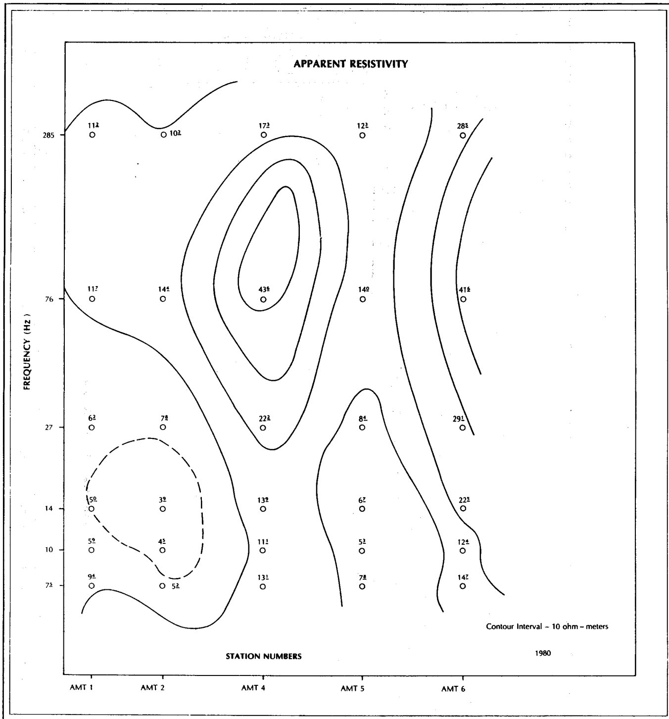
Figure 12. Pseudosection, audio-magnetotelluric data, west-east component. See Plate IX for location. Basic data from U.S. Geological Survey Open-File Report 76-7000.
