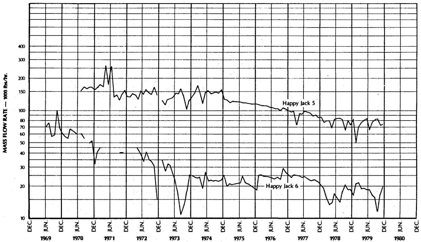
Figure 20. Steam production rate vs. time, wells "Happy Jack" 5 and 6, The Geysers Geothermal field.
