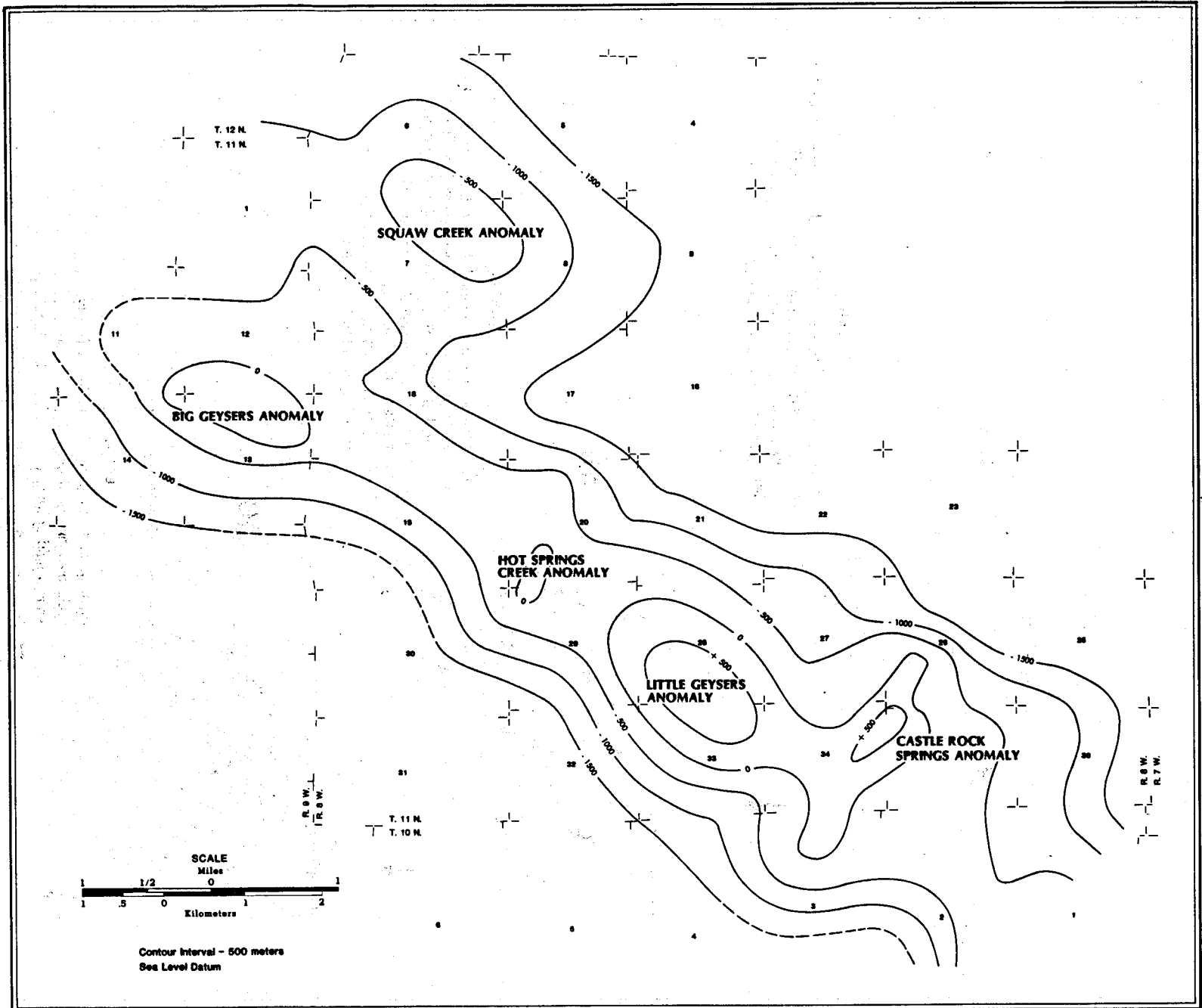
Figure 4. Idealized map of first reported steam entries at The Geysers Geothermal field. First steam entry major anomalies are indicated. Contours are in meters. California Division of Oil and Gas. Richard P. Thomas, 1981.
