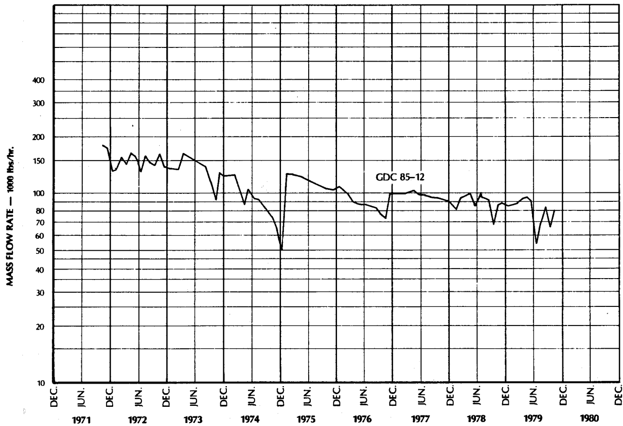
Figure 19. Steam production rate vs. time, well "GDC" 85-12 The Geysers Geothermal field.
