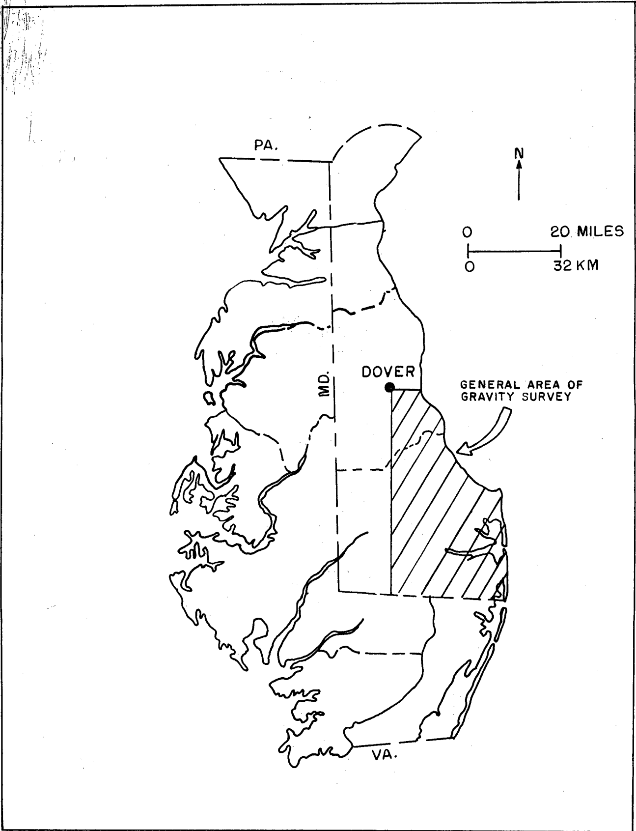
Figure 1. Map showing area of gravity survey.
