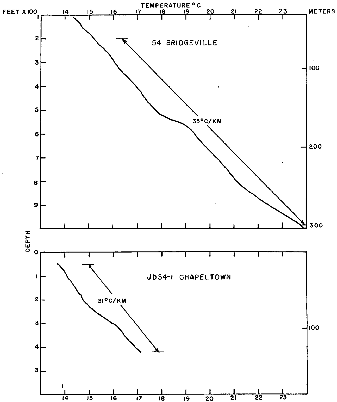
Figure 5. Temperature profiles in DOE test well 54 and domestic well Jb54-1.
