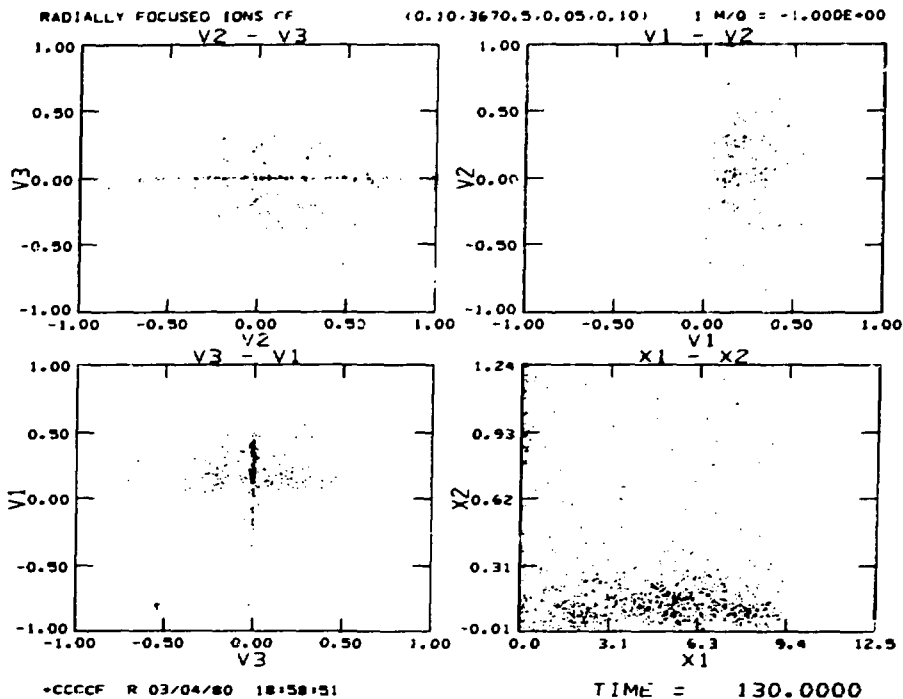
Fig. VIII-4. Configuration space \{X1(z) and X2(r)\} and velocity space \{V1(V_z), V2(V_r), and V3(V_\theta)\} simulation plots of a focused ion beam neutralized with hot comoving electrons. Normalized beam parameters are velocity v_0/c , focal angle \theta , mass ratio m_i/m_e , electron temperature V_{th}/c , V_0/c = V_e/c = 0.1 , \tan \theta = 0.1 , m_i m_e = 3670.5 , V_{th}/c = 0.05 , a_0 \omega_p/c = 1.0 .
