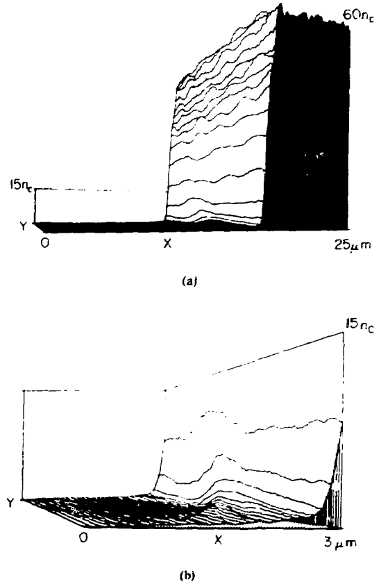
Fig. VI-11. Electron density profile for a wave simulation at eE_0/m_e\omega_0 = 0.3 , T_c = 625 eV, M_e/m_e = 100 , T_e/T_i = 10 , and 23° angle of incidence to the density gradient: (a) vs x and y for a self-consistent pressure balance density of 45 n_c , and (b) a blow-up plot of the base of the sharp gradient region that isolates the plasma wave. Contours in (a) and (b) are separated by only 0.1 \mu\text{m} .
