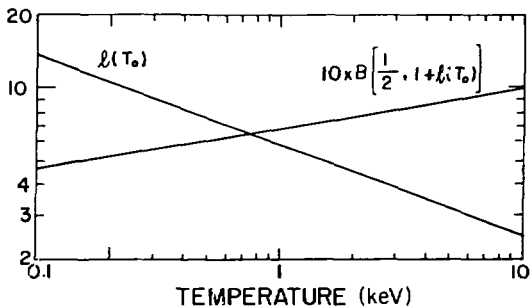
Fig. VI-7. Plot of function \ell (the exponent in the power-law fit of \langle \sigma v \rangle to fuel temperature) and B (the beta function) versus fuel temperature.
