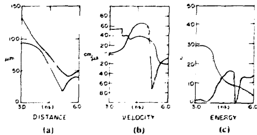
Fig. VI-4. Polaris shell collision from three perspectives.
