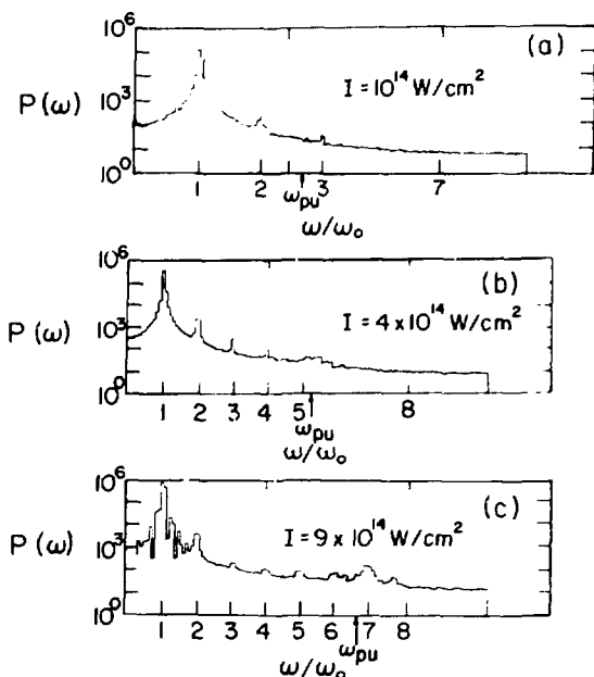
Fig. VI-12. Fourier power spectrum of the light leaving the left boundary of the simulation box for three laser intensities (a) 10^{14} W/cm 2 (that is, v_e/c = 0.1 ), (b) 4 \times 10^{14} W/cm 2 , and (c) 9 \times 10^{14} W/cm 2 . The emission at harmonics of the laser \omega_{pe} corresponds to the plasma frequency at the upper shelf density.
