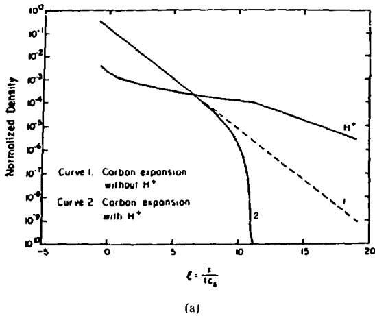
Fig. IV 9(a). Normalized carbon ion density (curve 2) and hydrogen ion density (curve H) versus self similar parameter \xi . Dotted line is single-species (carbon) solution.
