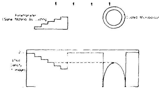
Fig. VII 17. Average coating thickness is measured by comparing the optical density in the center of the microballoon image with the optical density of a penetrometer.
