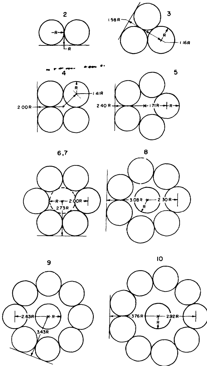
Fig. IX-9. Planar multiring laser amplifier layouts.
