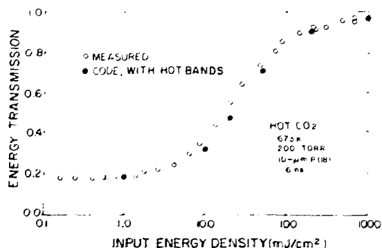
Fig. III-26. Transmission for 10- \mu m P(18) laser pulses. Other parameters are the same as in Fig. III-25.
