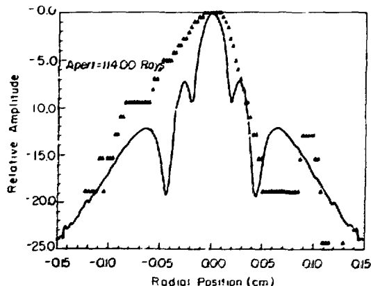
Fig. VII-14. Magnetoelastic beam profile—improved fit of data.
