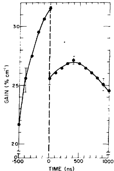
Fig. III-24. Gain vs time data for 1:4::N 2 :CO 2 laser mix at 1200 torr. E/N = 2.5 \times 10^{-16} v·cm 2 . Saturated extraction occurs at t = 0 . Note the nearly instantaneous recovery to 80% of preextraction gain.
