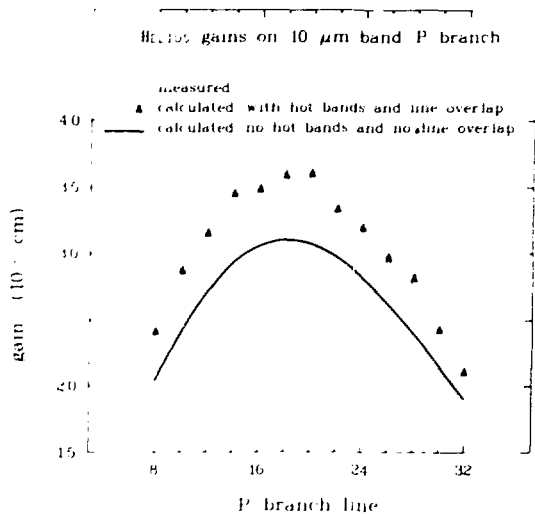
Fig. III-44. Comparison of calculated and observed gain vs line on the 10\ \mu\text{m} P branch transitions.
