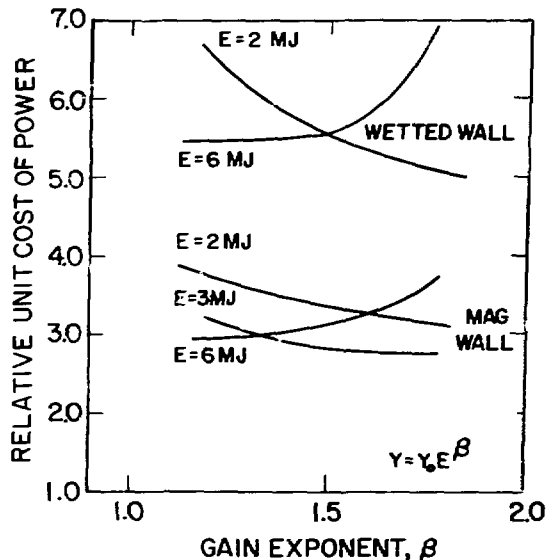
Fig. IX-2. Effect of gain exponent.
