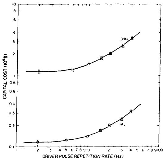
Fig. IX-8. Capital cost as function of driver pulse repetition rate for 1- and 10-MJ CO 2 lasers in Los Alamos multiring configuration for inertial fusion commercial applications (... salt-window option; Δ, aerowindow option).
