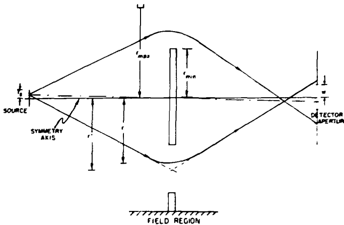
Fig. V-17. Schematic of a typical thin lens magnetic spectrometer.
