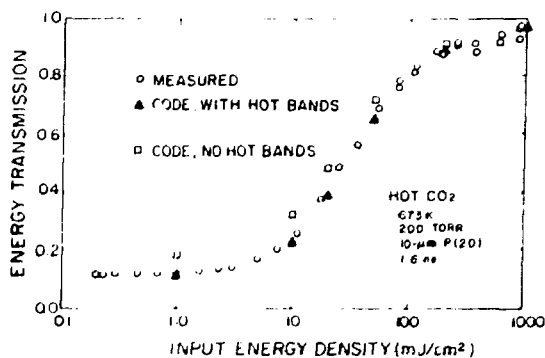
Fig. III-25. Transmission of 1.6-ns, 10- \mu m P(20) laser pulses through 118 cm of hot CO 2 at 200 torr; the spatial profile of the input pulse is flat. 20 Circles, measured data; squares, theory without hot band contribution; and triangles, theory with hot band effects.
