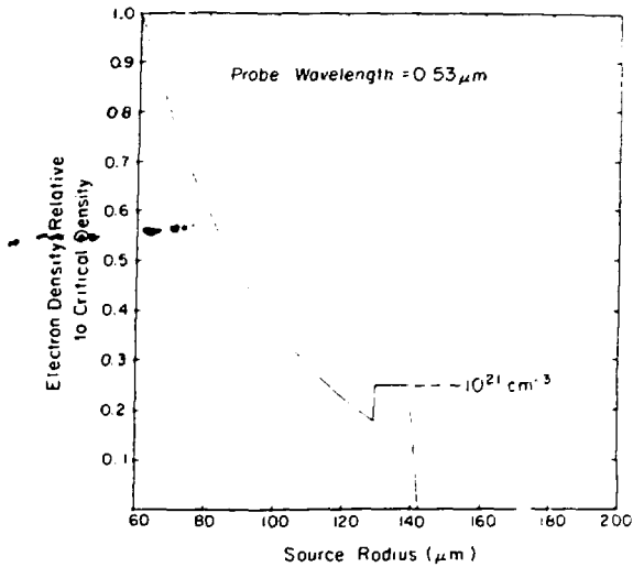
Fig. V-36. "Mesa" density profile.
