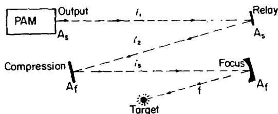
Fig. III-56. Schematic of angular multiplexing output optics.
