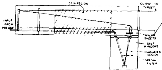
Fig. III-1. Old optical layout of Helios power amplifier.
