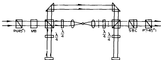
Fig. VII-19. Transmission-reflection interferometer.
