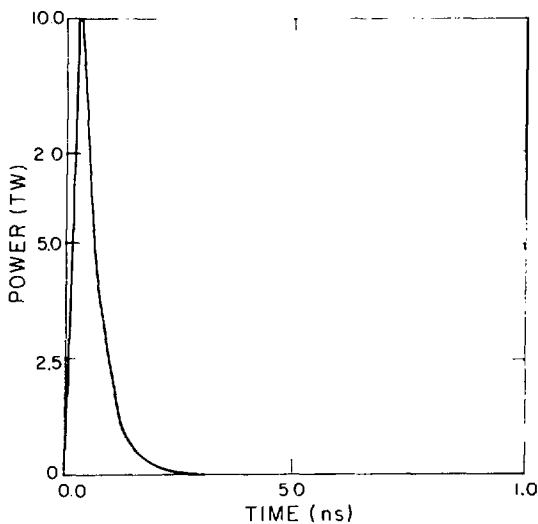
Fig. VI-2. Laser pulse shape.
