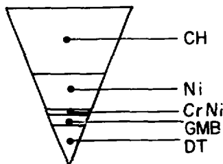
Fig. VII-22. Pie diagram of an ablative implosion target.
