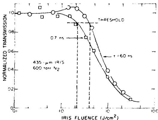
Fig. III-61. Normalized transmission vs input fluence at the iris edge. Transmissions are normalized to the small-signal values. The breakdown threshold fluence is a weak function of pulse length.
