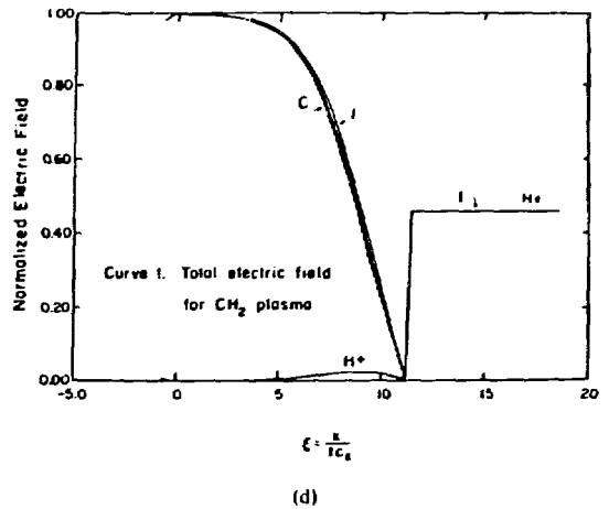
Fig. IV-9(d). Normalized total electric field caused by \text{CH}_2 plasma (curve 1) and decomposed electric fields caused by carbon electron flow (curve C) and hydrogen electron flow (curve H).
