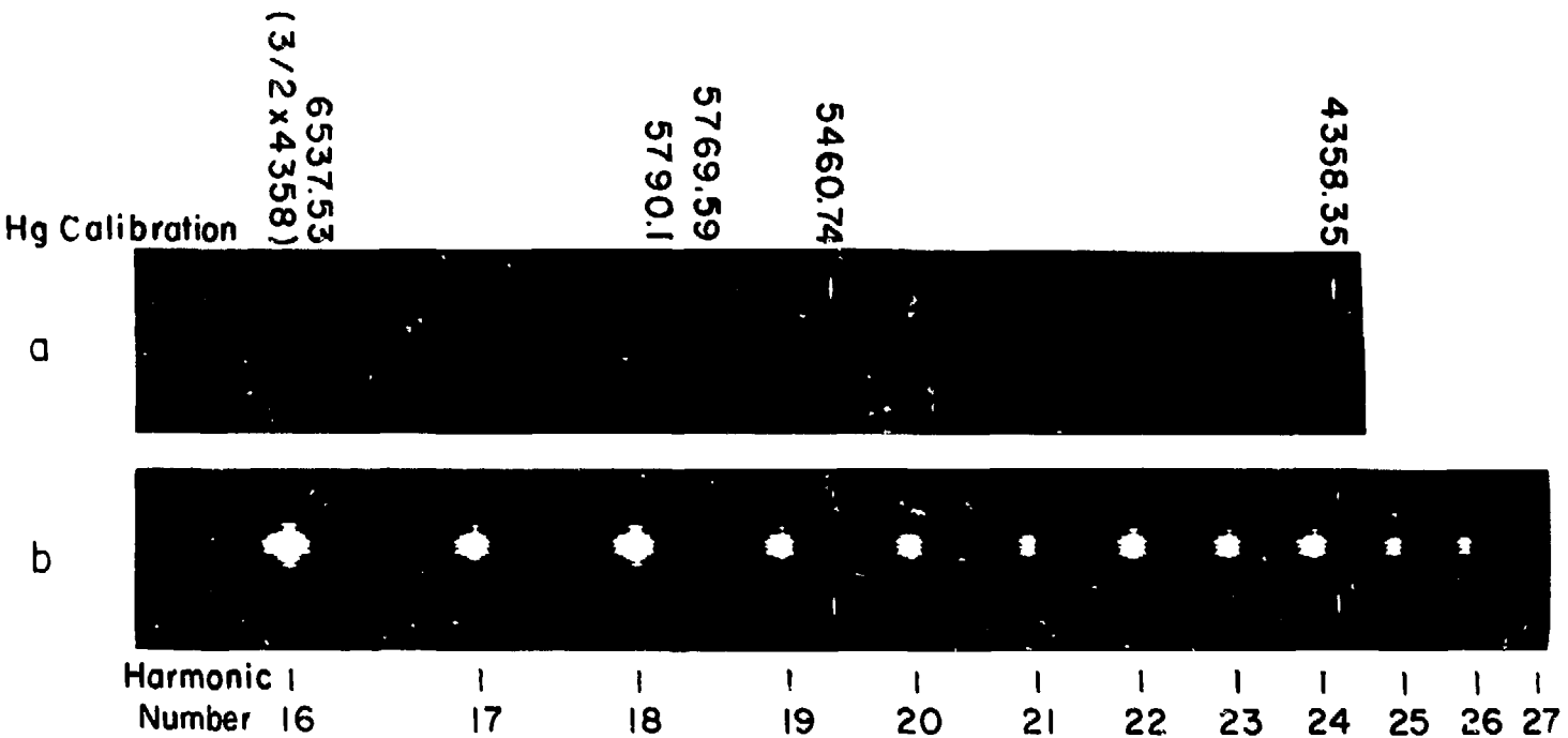
Fig. IV 7. Harmonic spectra obtained in parasitics experiments at (a) Gemini and (b) Helios.
