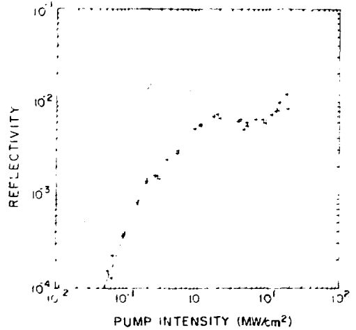
Fig. III-63. Phase conjugate reflectivity in a 2 cm long sample of KCl:KReO 4 with small signal absorption coefficient of 3. The solid line is the Abrams Lind model. The dashed line is the revised model.
