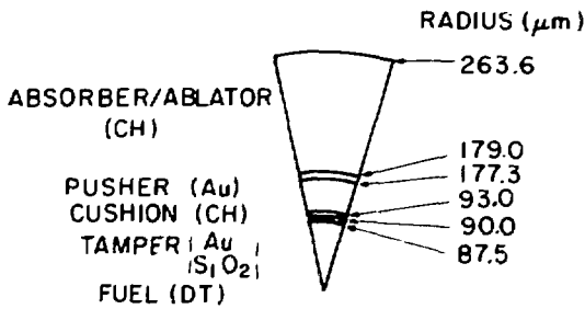
Fig. VI-1. Polaris target for Helios
