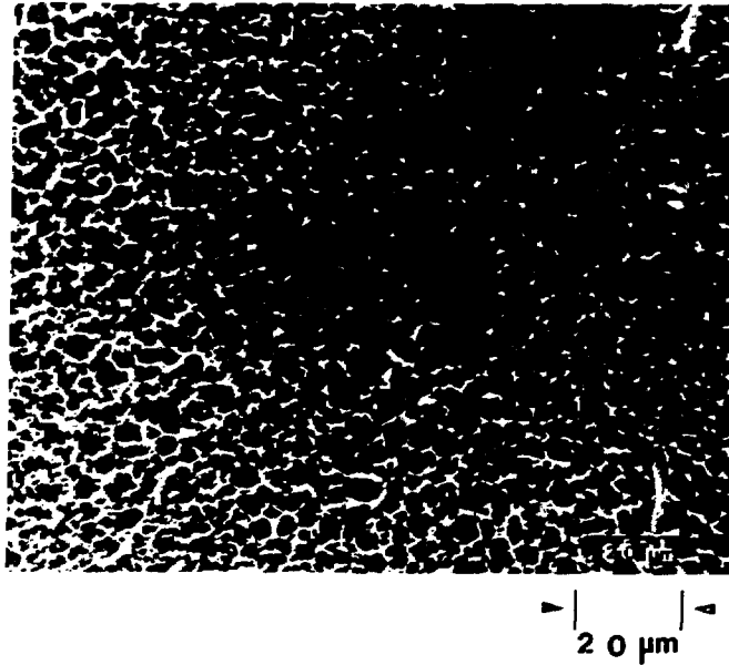
Fig. VII 37. Carboxymethyl cellulose foam. Density = 0.05 g/cm 3 .
