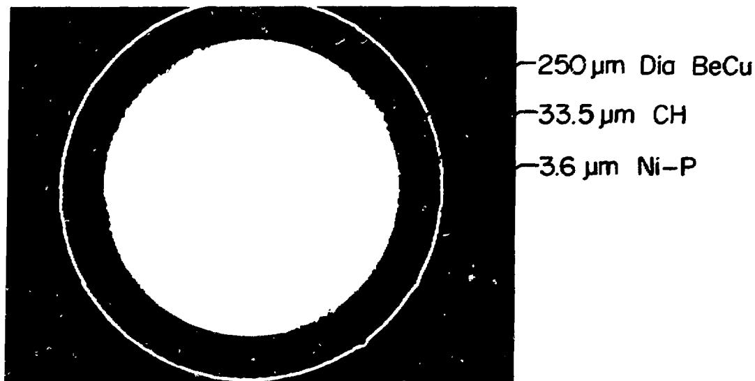
Fig. VII-26. Target for hot-electron measurements.
