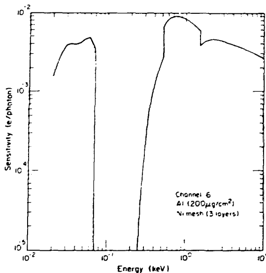
Fig. V-14. Detector response for a clean-machined aluminum cathode with a 4 lines/mm nickel mesh anode and a 200- \mu\text{g}/\text{cm}^2 aluminum filter window with three layers of 4 lines/mm nickel mesh as an x-ray neutral density filter.
