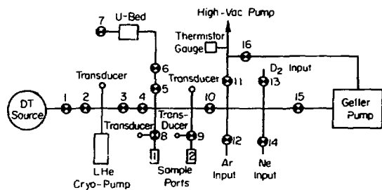
Fig. VII-8. High-pressure gas fill system.
