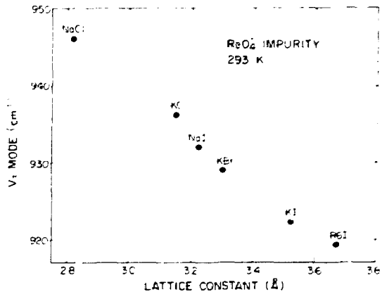
Fig. III 58. V 3 resonance for the ReO 4 impurity for six crystals with different lattice constants.
