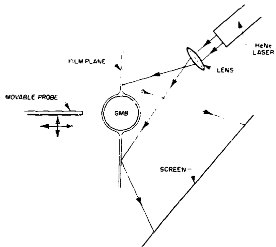
Fig. VII-3. Schematic of GMB centering.
