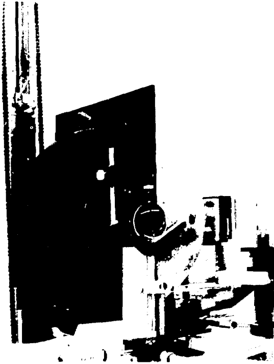
Fig. IV-3. Integrating sphere. The inner gold surface has been polished to provide very high reflectance ( \sim 98\% ) for 10.6\text{-}\mu\text{m} wavelength light. The black matte finish on the outside minimizes reflections that can produce parasitic oscillation in the laser system.
