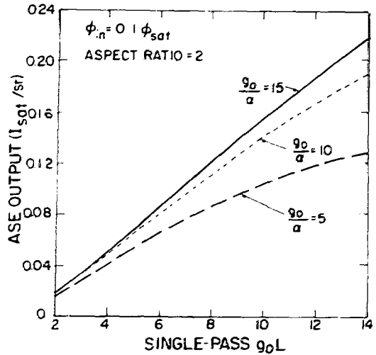
Fig. III-54. ASE output from a double-pass amplifier driven at 10% of saturation intensity.
