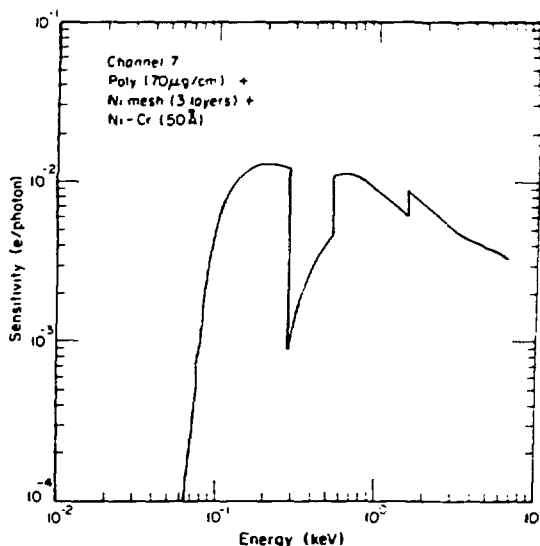
Fig. V-15. Detector response for a clean-machined aluminum cathode with a 4 lines/mm nickel mesh anode and a 70- \mu\text{g}/\text{cm}^2 polypropylene plus 50- \text{\AA} nickel-chrome filter window with three layers of 4 lines/mm nickel mesh as an x-ray neutral density filter.
