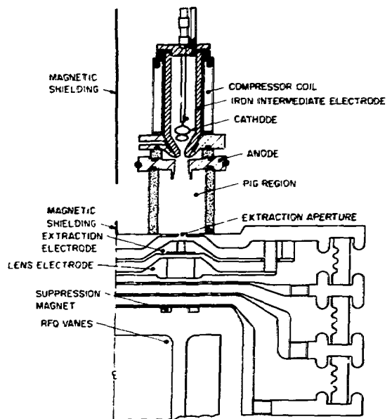
Fig. VIII-1. One quadrant of RFQ accelerator injector.
