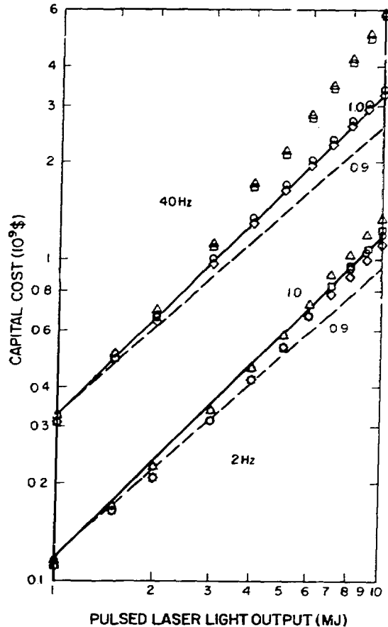
Fig. IX-7. Capital cost as function of driver pulsed-energy output for 2- and 40-Hz CO 2 lasers for inertial fusion commercial applications. \Delta , salt window option and AVCO single-ring configuration; \circ , aerowindow option and AVCO single-ring configuration; \Delta , salt window option and Los Alamos multiring configuration; \circ , aerowindow option and Los Alamos multiring configuration; and solid line, 1.0 exponent scaling with energy for salt window option that might apply to large construction projects.
