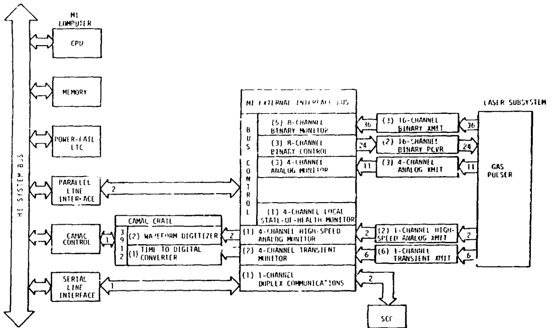
Fig. II-17. Typical Antares MI processor.
