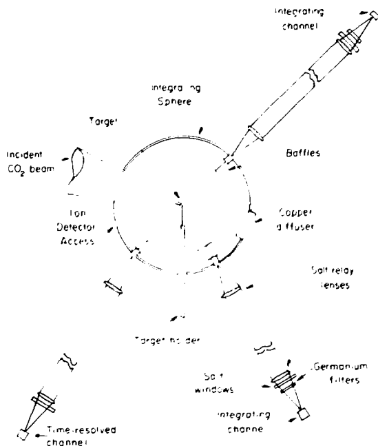
Fig. IV 1. Experimental configuration of an integrating sphere.
