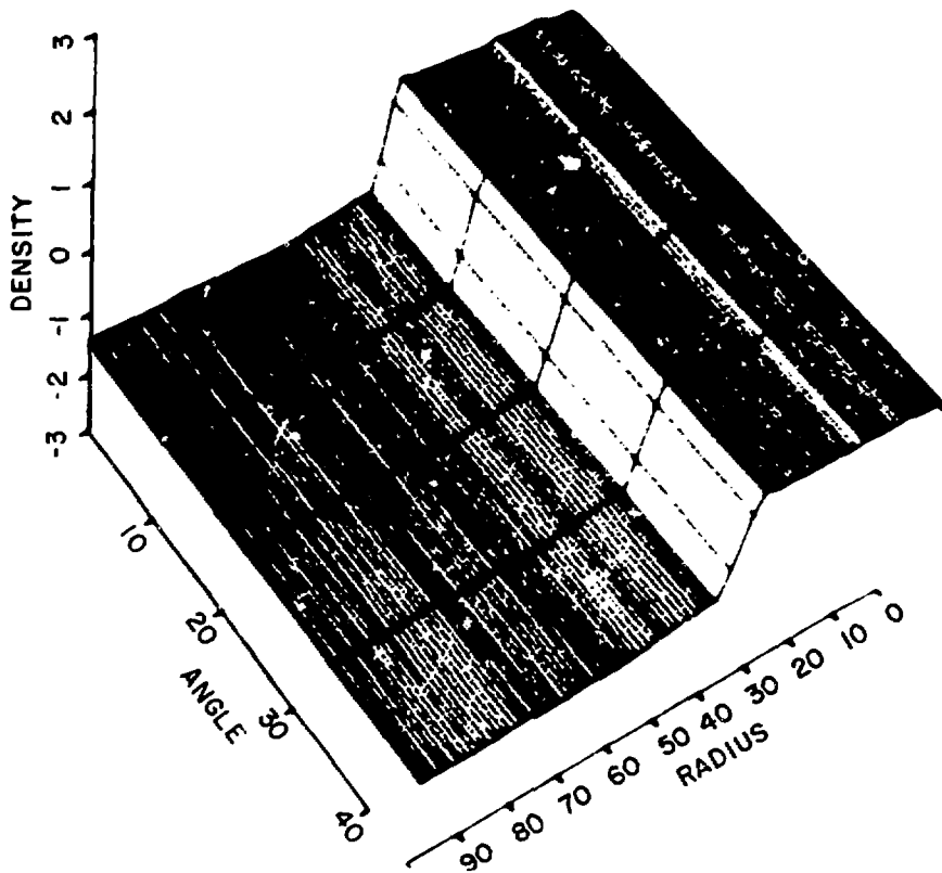
Fig. VI-20. Shell after rebound from the origin.
