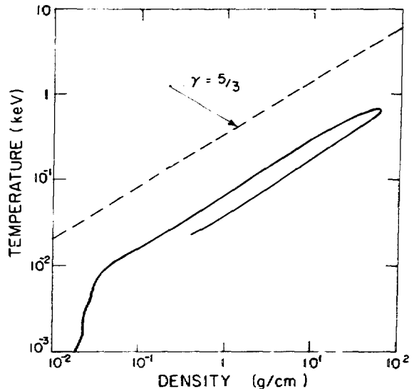
Fig. VI-5. Temperature density history of DT fuel.
