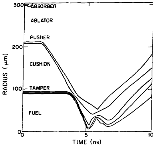
Fig. VI-3. Target interface time histories.
