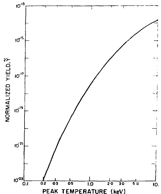
Fig. VI-8. Normalized neutron yield \tilde{Y} versus peak fuel temperature T_0 .
