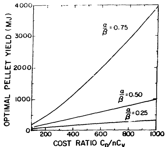
Fig. IX-1. Optimal pellet yield.
