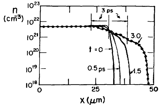
Fig. VI-13. Electron density n_e (dotted line) and ion charge density Zn_i (solid line) curves for the expansion of a Z = 10 , A = 25 plasma with T_e/T_i = 10 . Evolution to \omega_p \Delta t = 1.2 \times 10^4 with \omega_p \Delta t = 4 , \Delta x/\lambda_D = 47.8 .
