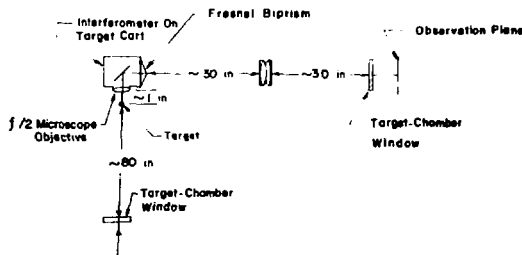
Fig. V-29. The f/2 microinterferometer arrangement for Helios.
