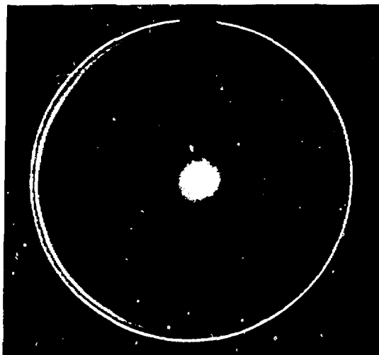
Fig. VII-23. Photomicrographs of sections through bare spots on chromium-nickel flashed 2\text{-}\mu\text{m} electroless nickel-plated GMBs. Two distinct layers are evident; the chromium-nickel layer is extremely nonuniform.
