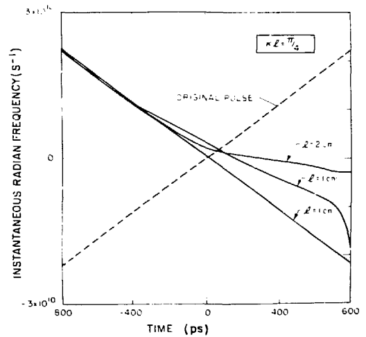
Fig. III-75. Study of the chirp reversal process. The instantaneous frequency shift vs time curve is shown for the positively chirped input pulse. Again (as in the previous two figures) the cw on-resonance conjugate reflectivity is set to unity, but the physical thickness of the conjugator is varied. For a physically thin conjugator (one that is sufficiently broadband), the chirp reversal is nearly perfect, but for thicker conjugators, the chirp at the peak of the pulse is significantly reduced.
