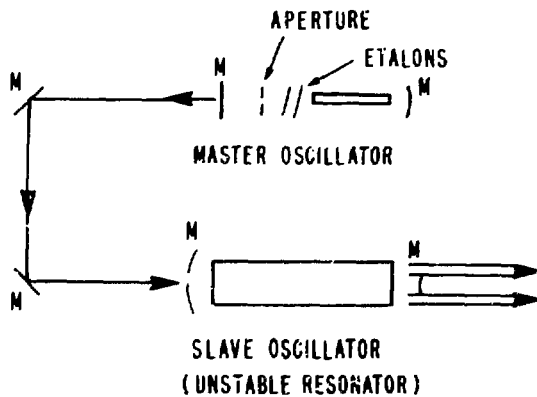
Fig. III-79. Injection-locked KrF master-slave oscillator system.
