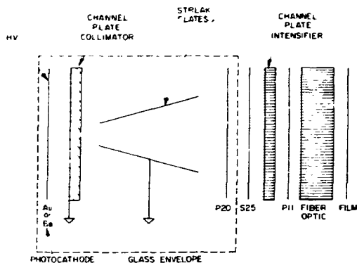
Fig. V-7. Cross section of MULTIFLEX detector system.
