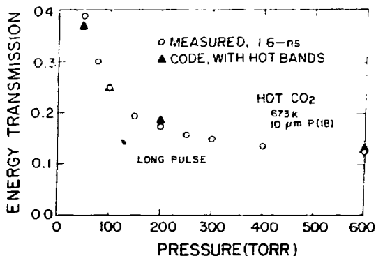
Fig. III-27. Small-signal transmission of weak 1.6-ns, P(18) laser pulses through 118 cm of hot (673 K) CO 2 at various pressures. The dashed line is the theoretical transmission for long (or cw) pulses.
