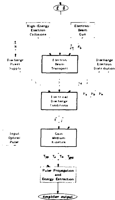
Fig. III-40. Logic structure of model. The boxes indicate the processes included in the model, and the arrows show how they relate to each other. (The ellipses contain the variables producing the interdependencies.) The solid arrows indicate computational flow, whereas the dotted arrows indicate feedback loops producing self-consistency. Several approximations discussed in the text have been used to simplify the interconnections as much as possible.
