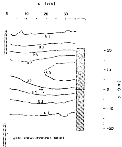
Fig. III-43. Distribution of discharge power P = \vec{E} \cdot \vec{J} in Helios amplifier, under the conditions shown in Fig. III-42. Contours are normalized to peak pumping = 1.05 \times 10^8 \text{ W/cm}^2 .
