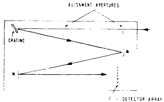
Fig. III-22. Multiline spectrometer for pulse-shape and line-content measurements in Helios.
