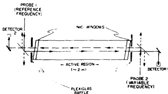
Fig. III-6. Experimental layout for gain-vs-frequency measurements in Helios.
