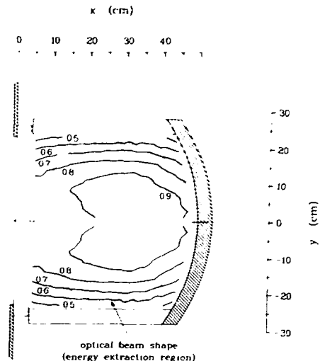
Fig. III-46. Discharge power uniformity corresponding to conditions shown in Fig. III-45. The curved anode and dielectric shields increase the power-loading at the edges of the discharge. (Structures shown are theoretical only, because any real dielectric and anode would have to be shaped to avoid excessive electrical stresses.) The figure shows a 44-cm-diam optical beam extraction region.
