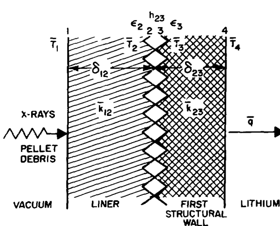
Fig. IX-6. Heat-transfer model for protective liner.
