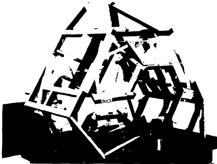
Fig. II-15. Scale model of Antares target-chamber space frame.
