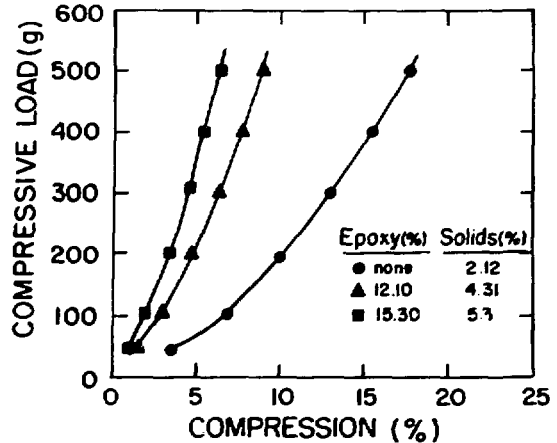
Fig. VII-43. Compressive-stress station curves for stainless steel fiber felts as a function of added epoxy binder.
