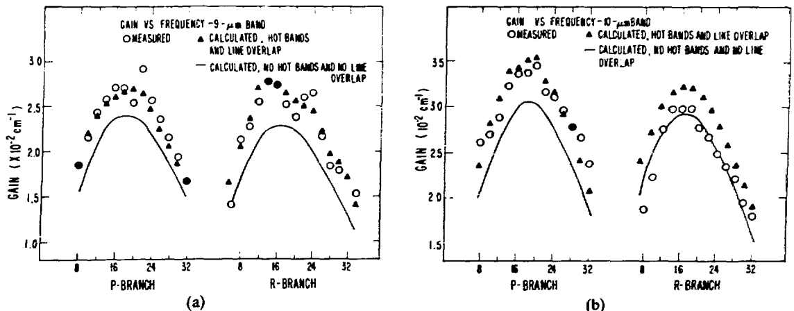
Fig. III-7. Calculated and measured gains in the (a) 9\text{-}\mu\text{m} and (b) 10\text{-}\mu\text{m} bands of an 1800-torr \text{CO}_2 amplifier.
