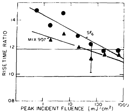
Fig. III-13. Risetime ratio of pulses traversing a gas cell. The pulse wavelength is 10.6\text{ }\mu\text{m} P(20).
