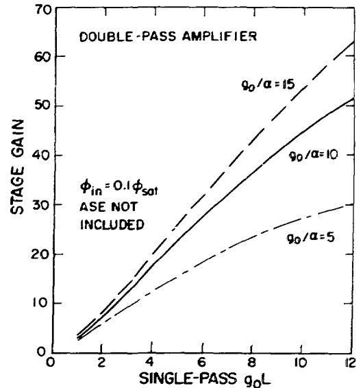
Fig. III-50. Stage gain for a double-pass amplifier without ASE.
