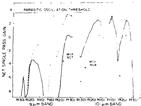
Fig. III-3. Net single-pass small-signal gain G(\lambda) for all the 9 and 10- \mu\text{m} CO 2 laser lines having significant gain in the Helios power amplifiers for Mix 804 and Mix 907. The parasitics threshold region for these amplifiers with a target in place lies between a net gain of 3 to 3.5. The pressures of the gas mixes used for this calculation were 18 torr of Mix 907 (a pressure that just stabilizes the Helios amplifiers) and 20 torr of Mix 804. Both had an absorber-cell path length of 77.5 cm.
