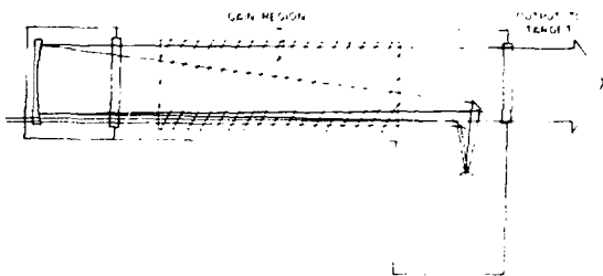
Fig. III-2. Modified optical layout of Helios power amplifier.
