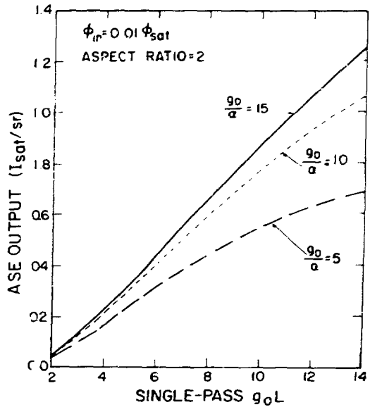
Fig. III-55. ASE output from a double-pass amplifier driven at 1% of saturation intensity.
