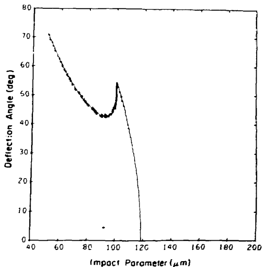
Fig. V-32. Plot of scattering angle vs impact parameter.
