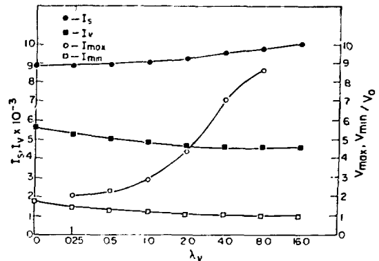
Fig. VI-30. The values of I_s , I_v , and the maximum and minimum cell volumes are plotted for various values of \lambda_v . V_{\text{min}} decreases less than V_{\text{max}} increases from its value for \lambda_v = 0 .
