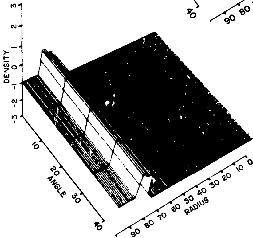
Fig. VI 17. Shock beginning its passage through spherical shell.
