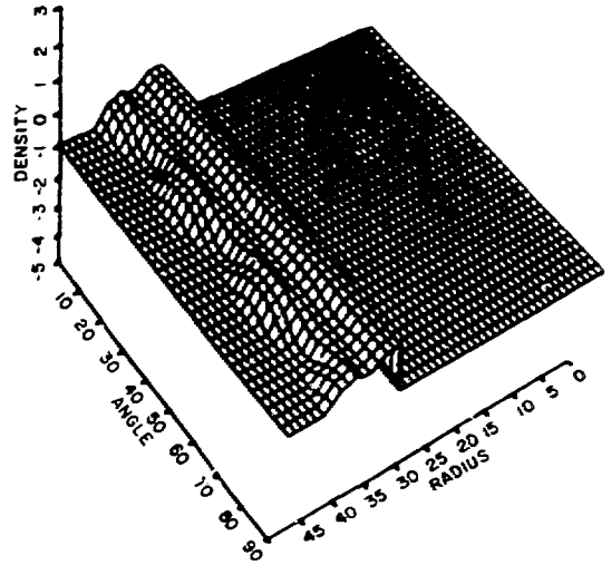
Fig. VI-25. Shell after passage of shock.
