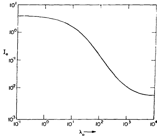
Fig. VI-34. Corresponding to the meshes shown in Fig. VI-33, I_0' decreases as \lambda_0 increases.
