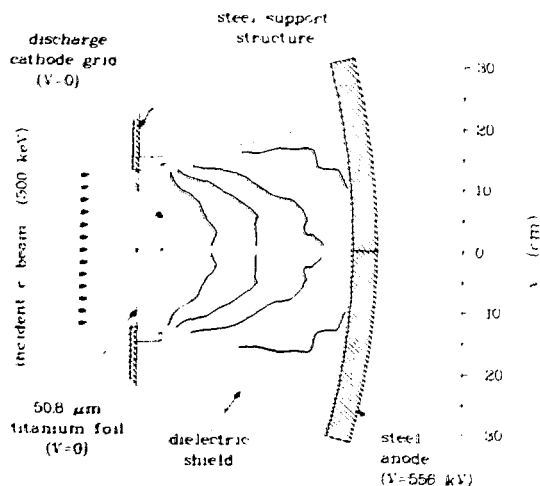
Fig. III-10. Transverse view of a single section of an Antares PAM showing the gain profile at 2 \mu\text{s} with a dielectric shield to confine the discharge.
