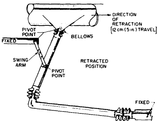
Fig. VII-45. Swing-arm assembly used to retract the cryogenic shroud.
