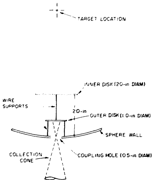
Fig. IV 2. Integrating sphere baffle detail.
