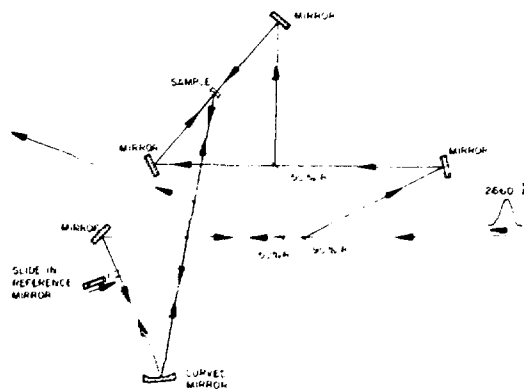
Fig. III-77. Experimental arrangement. Most of the ultrashort pulse is directed to provide the counterpropagating pump waves; the remainder is brought to the sample as a probe beam.
