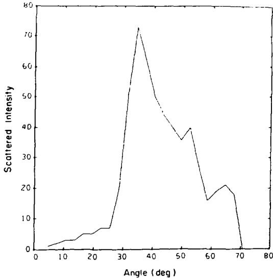
Fig. V-37. Intensity-vs-angle plot incident on the "mesa" profile.
