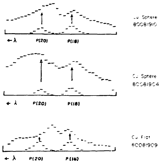
Fig. IV-13. Representative backscatter spectra from copper targets.
