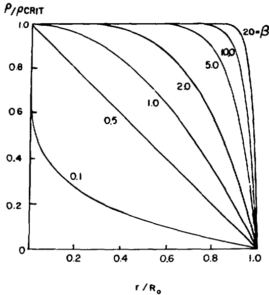
Fig. V-23. Electron density as a function of \beta .
