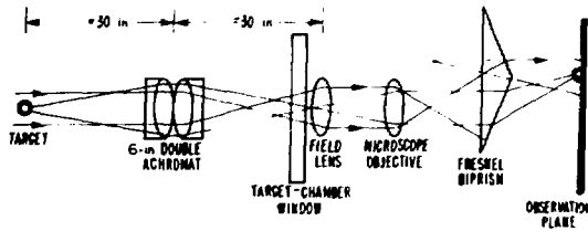
Fig. V-28. The f/5 microinterferometer scheme for Helios.
