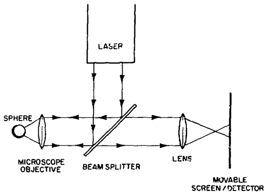
Fig. VII-2. Schematic of confocal alignment.
