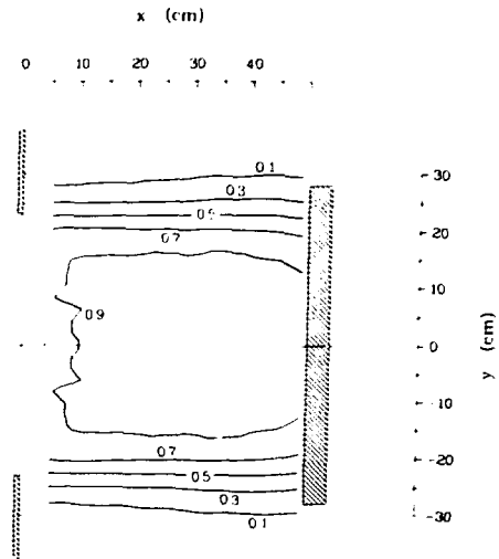
Fig. III-48. Discharge power uniformity for the conditions shown in Fig. III-47. By combining the techniques shown in Figs. III-44 and III-47, larger amplifiers than those shown here could be designed with high uniformity.
