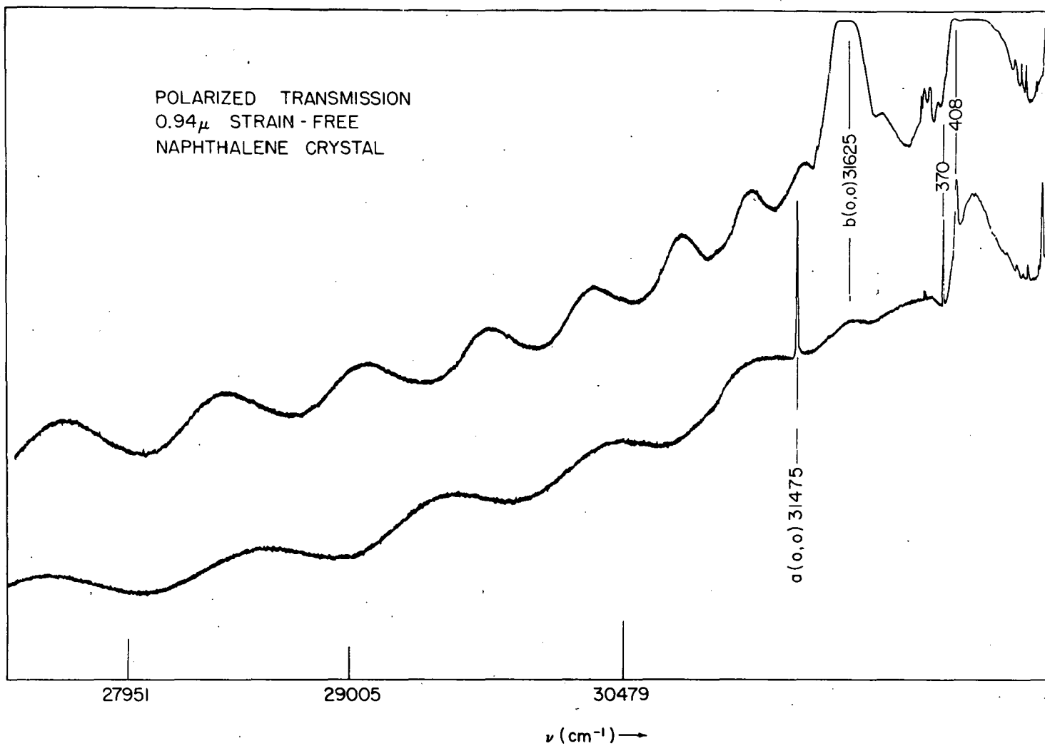
Figure 22. Polarized transmission 0.94 \mu strain-free naphthalene crystal
