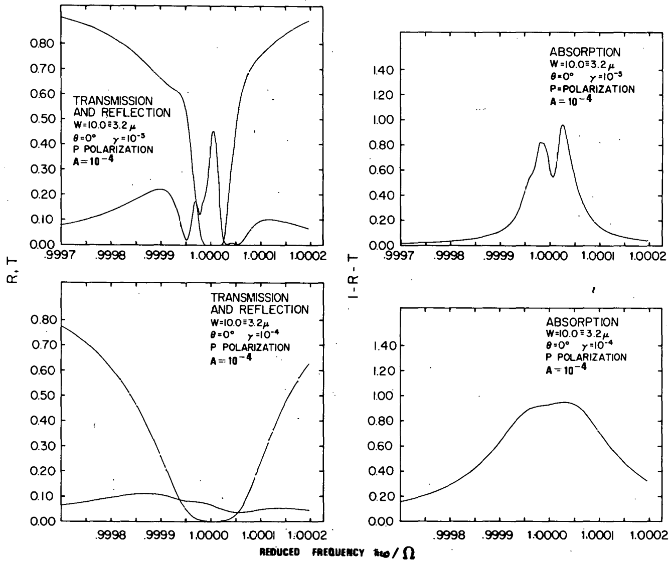
Figure 18. Computer generated reflection, transmission and absorption
