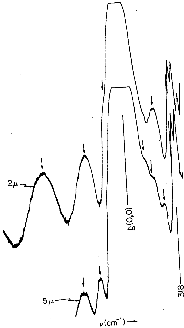
Figure 23. Thickness dependent interference modes in the b(0,0) region
