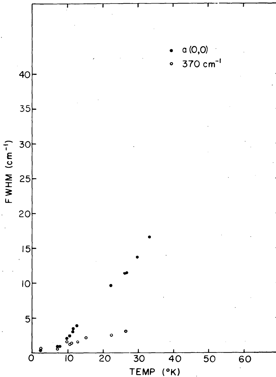
Figure 37. Comparison of FWHM of a(0,0) and 370 \text{ cm}^{-1} bands in pure, strain-free naphthalene crystal
