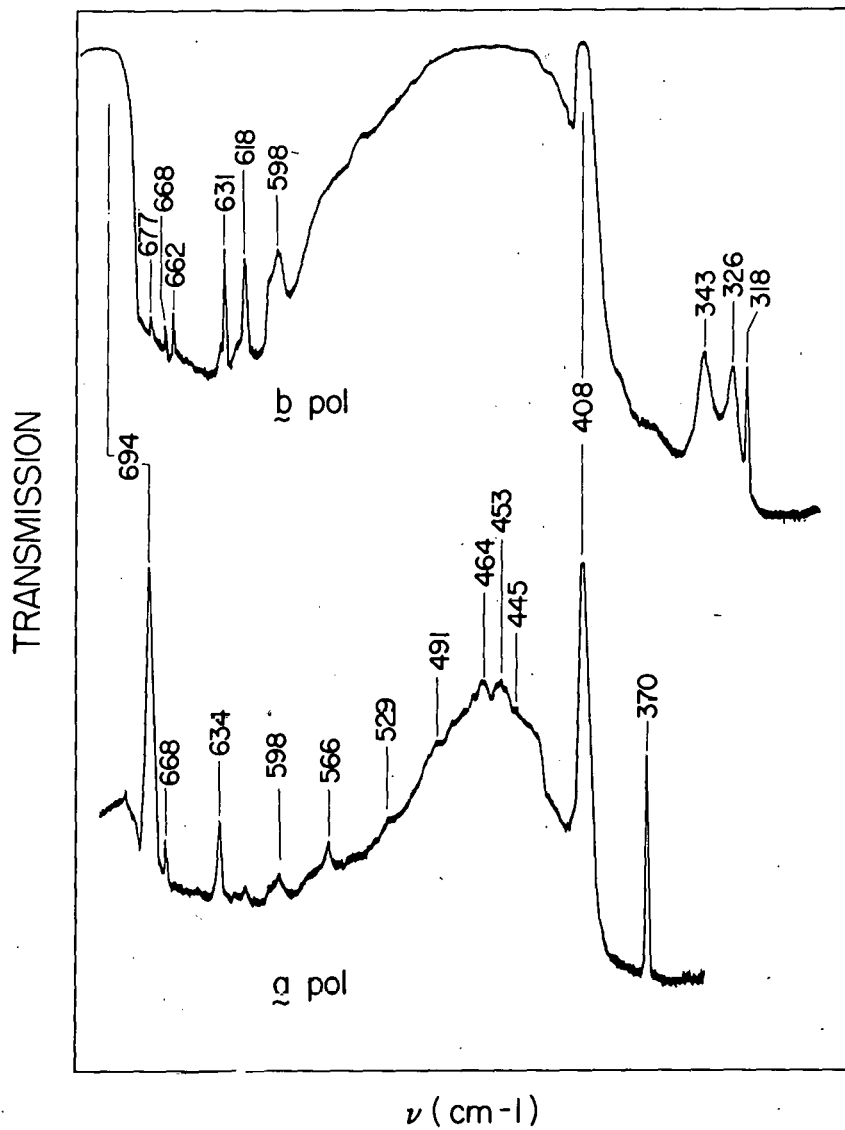
Figure 25. Enlargement of the "M" band region in perfect crystal
