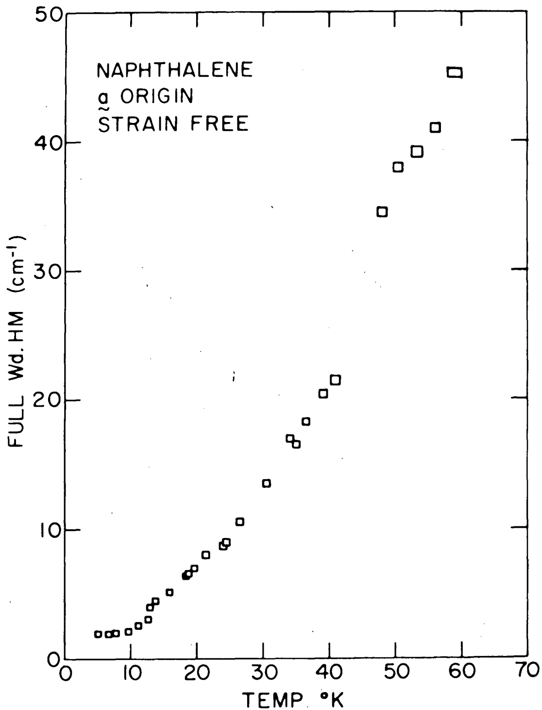
Figure 36. a(0,0) full width-half maxima for >5 \mu pure strain-free naphthalene crystal
