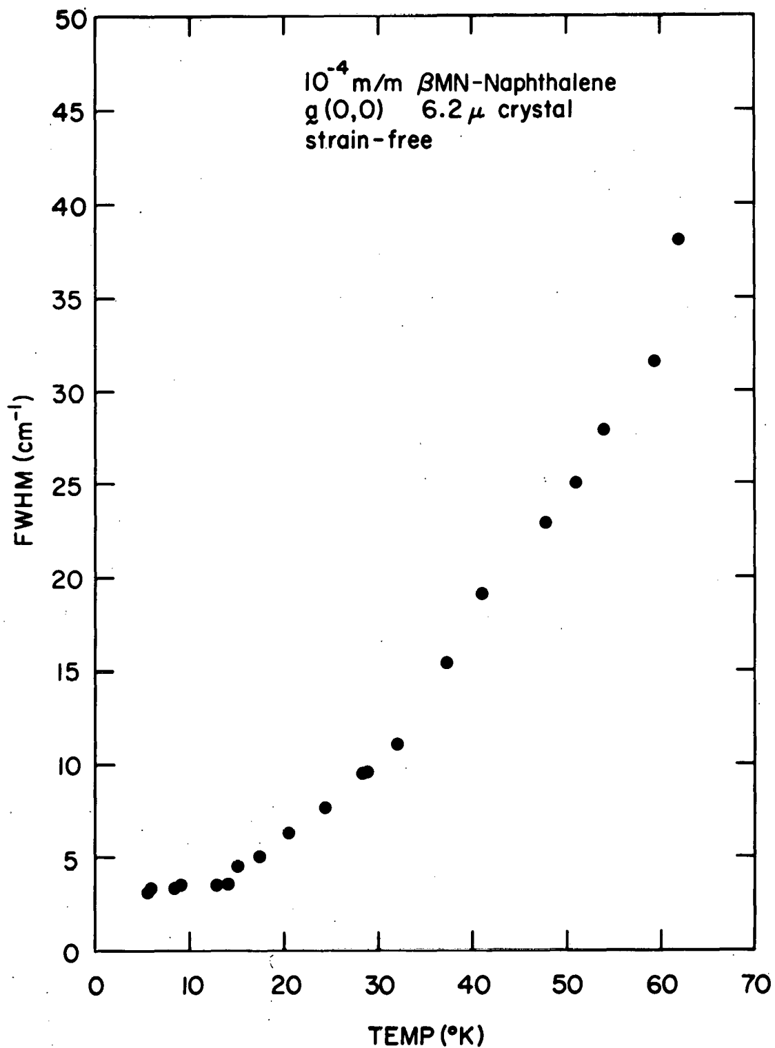
Figure 43. FWHM behavior for 10 -4 m/m \beta MN doped naphthalene crystal
