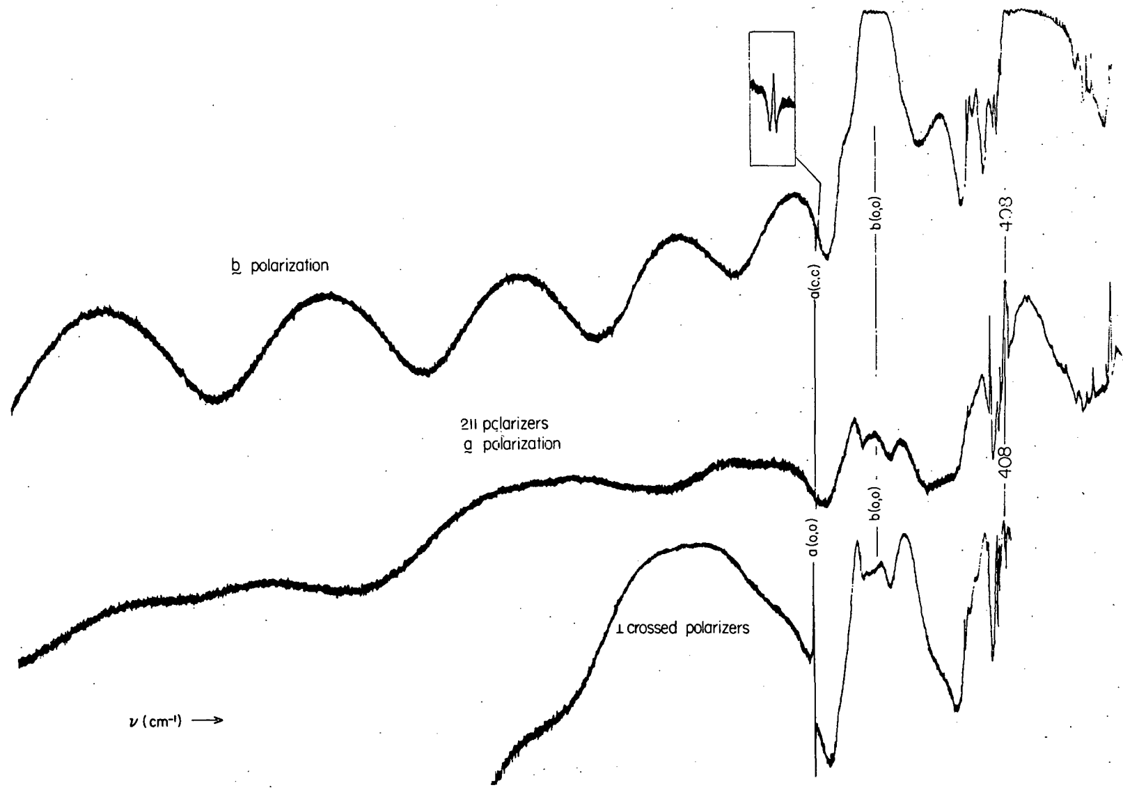
Figure 46. Depolarization effect in S_{0+1} naphthalene spectrum
