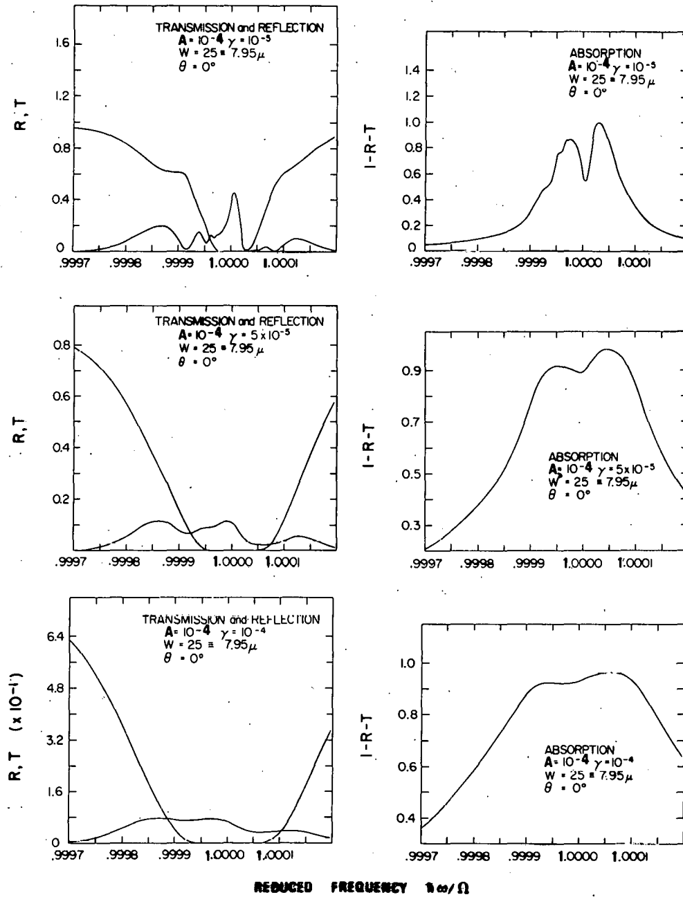
Figure 19. Computer generated reflection, transmission and absorption
