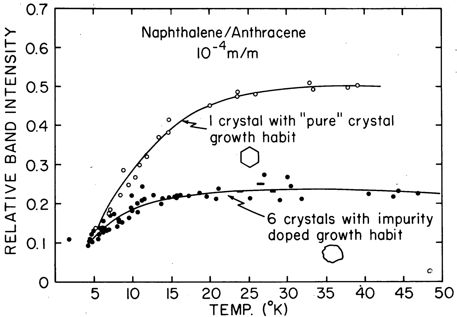
Figure 44. \alpha(0,0) area increase with temperature for anthracene doped naphthalene crystals
