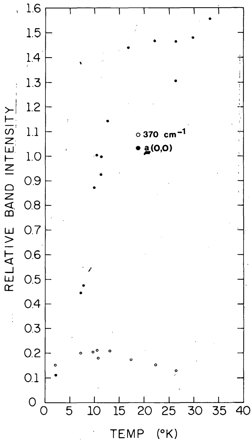
Figure 33. Area of \underline{a}(0,0) and 370\text{ cm}^{-1} band as a function of temperature for 2.3\ \mu crystals
