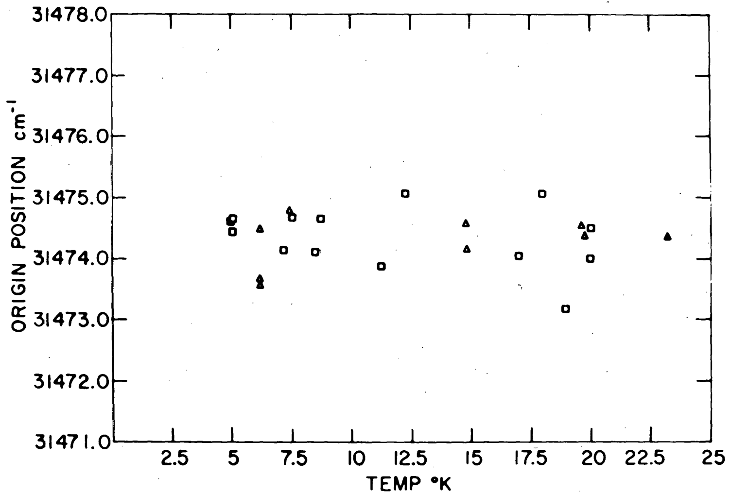
Figure 38. Energy shift of \underline{a}(0,0) vs temperature for two perfect crystals
