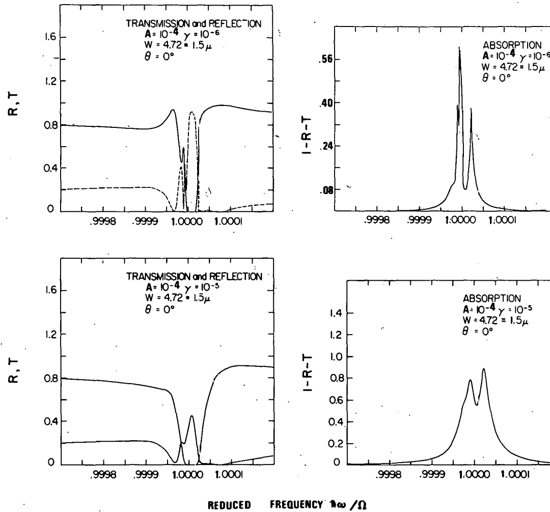
Figure 17. Computer generated reflection, transmission and absorption
