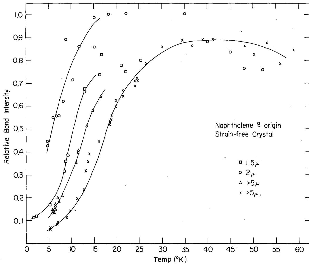
Figure 32. Area of a(0,0) for several perfect crystals as a function of temperature
