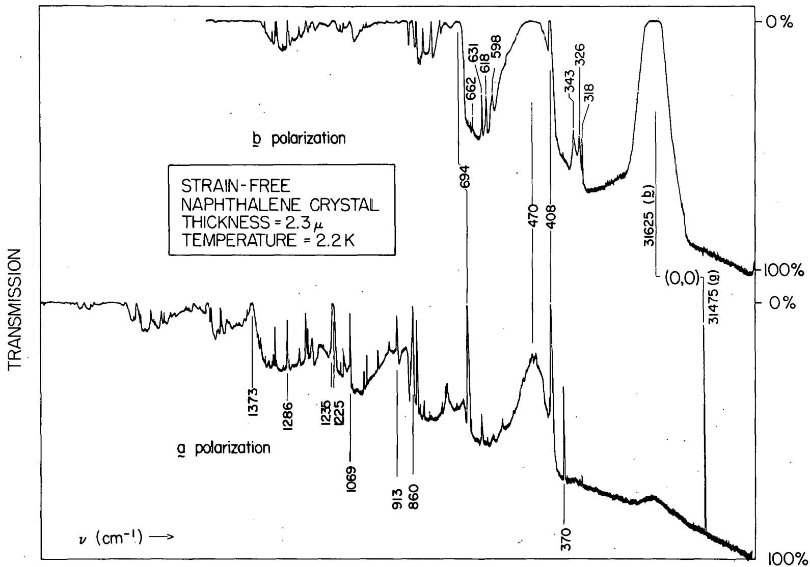
Figure 24. S_{1+0} absorption in perfect naphthalene crystal
