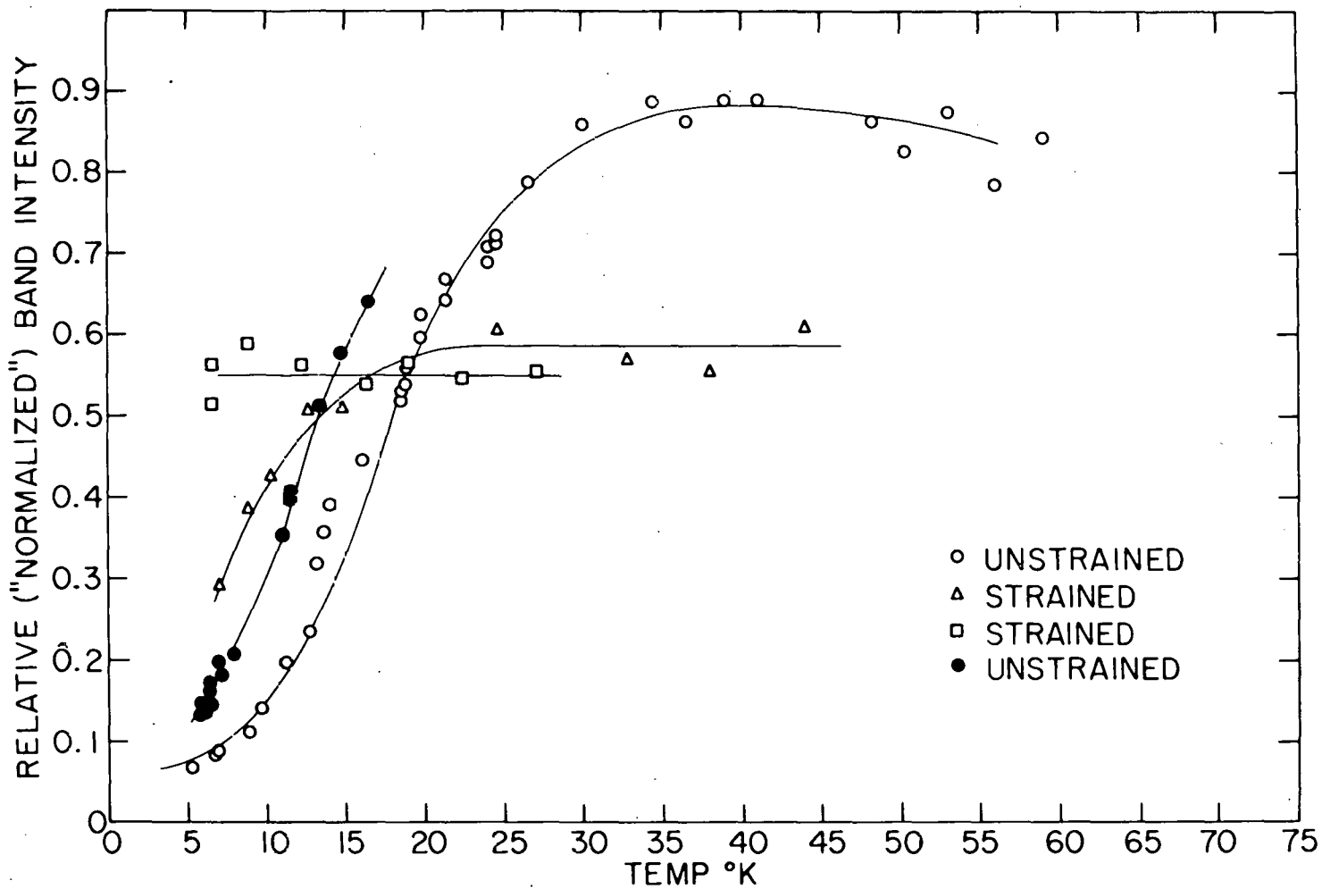
Figure 39. Temperature dependence of \mu(0,0) area in pure crystals
