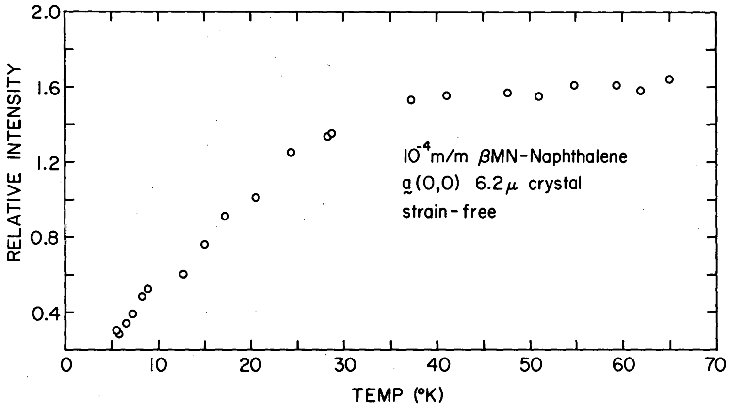
Figure 42. a(0,0) area increase in 10^{-4} m/m \beta MN doped naphthalene crystal
