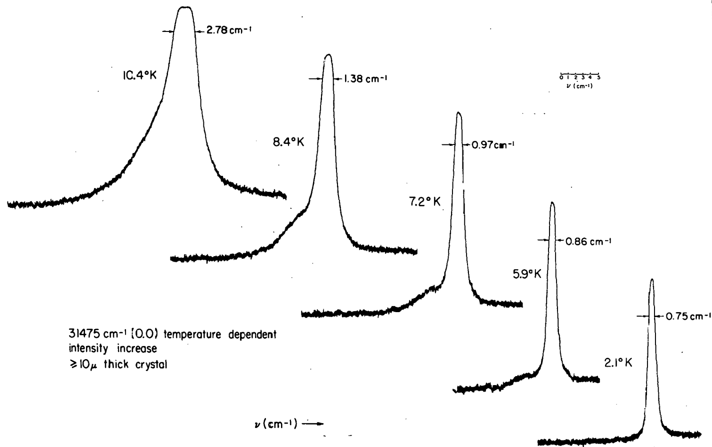
Figure 26. Spectral profile of the naphthalene \tilde{a}(0,0) band as a function of temperature
