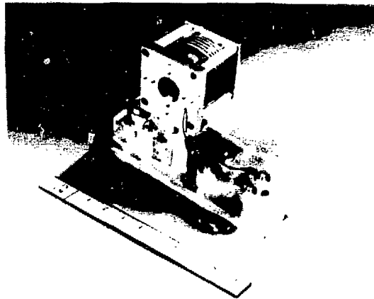
Figure 3. Photograph of MEVVA III.
