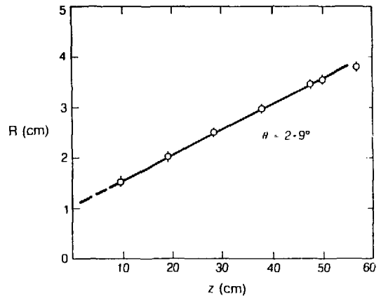
Figure 6. Beam half-width vs. distance from extractor.
