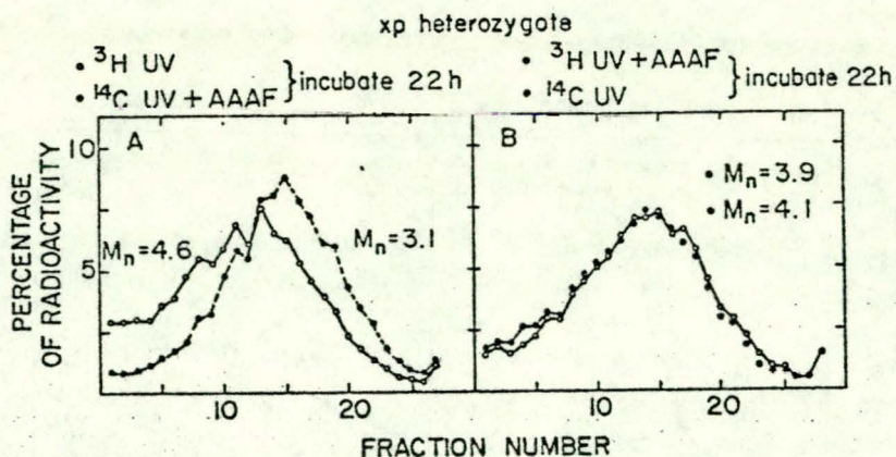
Fig. 4. Sedimentation profiles, in alkali of the DNAs from Experiment (1) of Fig. 1 with the radioactive labels reversed.
