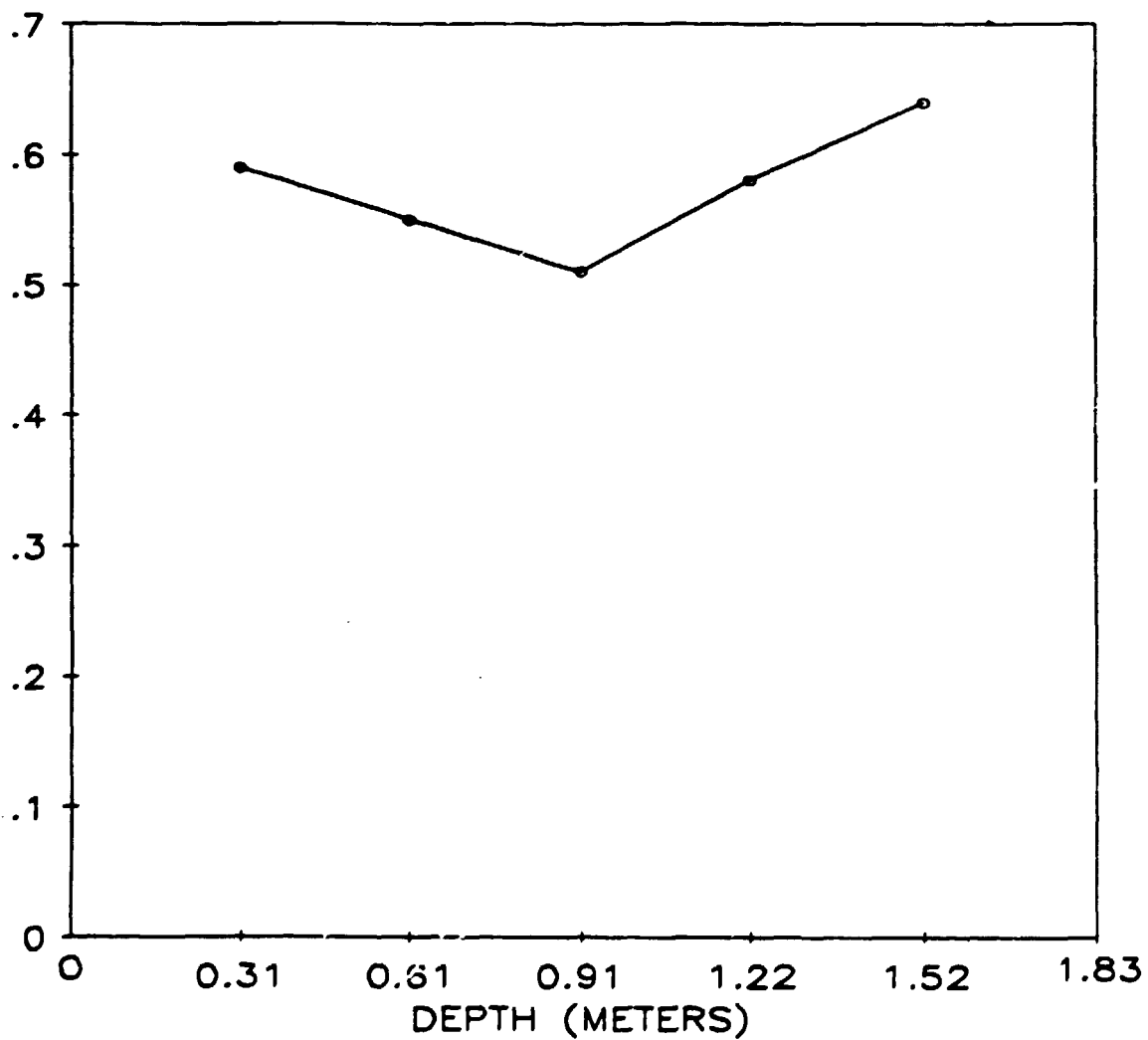
Fig. 5. Gamma profile for auger hole 3 (LJ039A3) at 5 Branca Court, Lodi, New Jersey.
