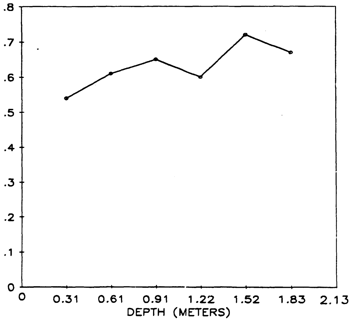
Fig. 4. Gamma profile for auger hole 2 (LJ039A2) at 5 Branca Court, Lodi, New Jersey.
