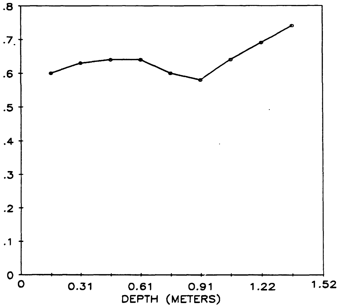
Fig. 3. Gamma profile for auger hole 1 (LJ039A1) at 5 Branca Court, Lodi, New Jersey.
