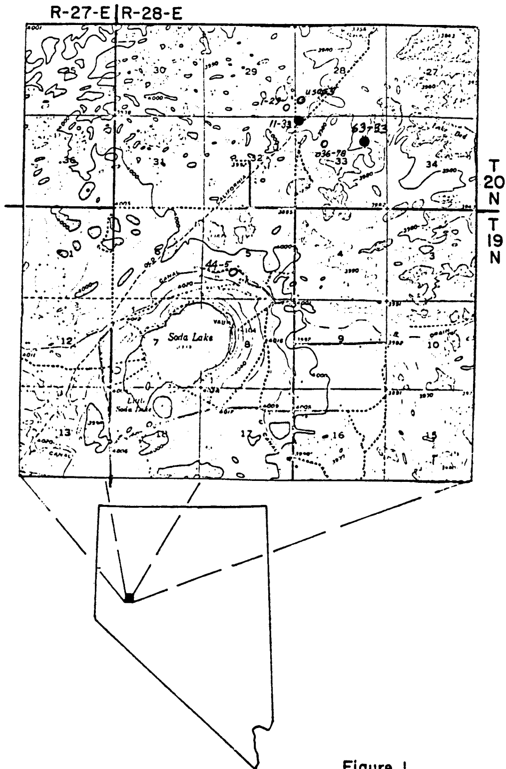
Figure 1 SODA LAKE, NEVADA GEOTHERMAL TEMPERATURE HOLES
