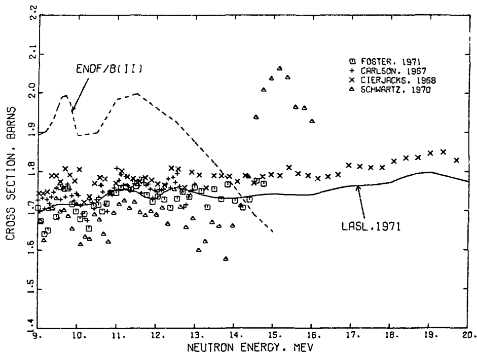
Fig. 8. Measured and evaluated total cross section for ^{27}\text{Al} from 9 to 20 MeV. The experimental data are averages of 3 points for the Carlson (Ca67) results, 8 points for Eierjacks (E168), and 5 points for Schwartz (Sc70).
