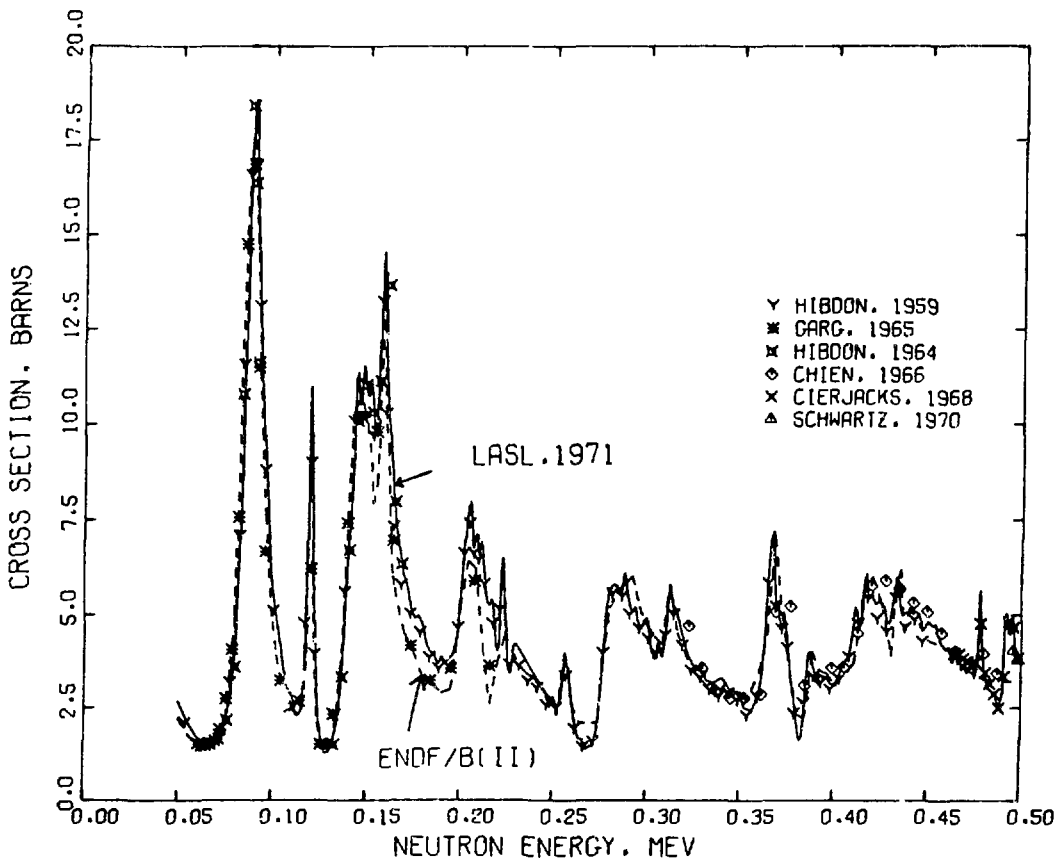
Fig. 3. Measured and evaluated total cross section for 27 Al from 0.05 to 0.50 MeV. The experimental data are averages of 5 points for the Hibdon (Hi59) results, 10 points for Garg (Ga65), 4 points for Hibdon (Hi64), 5 points for Chien (Ch66), 15 points for Cierjacks (Ci68), and 10 points for Schwartz (Sc70).
