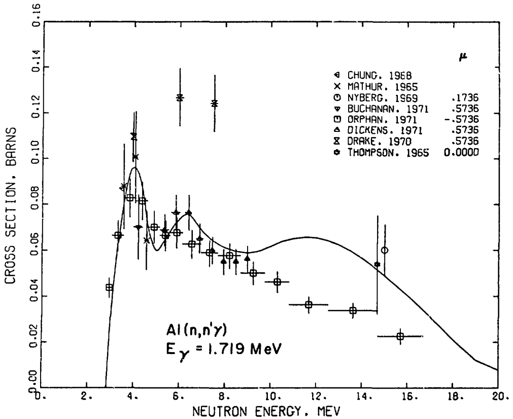
Fig. 43. Measured and evaluated ^{27}Al(n,n'\gamma) cross section for the 1.719-MeV photon from the 2.732 \rightarrow 1.013-MeV transition in ^{27}Al
