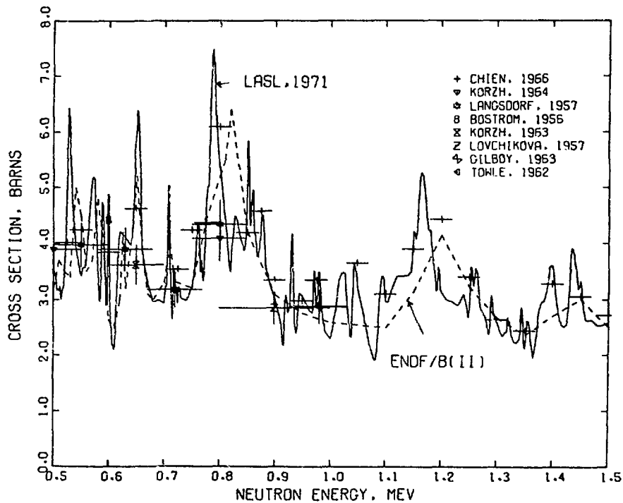
Fig. 10. Measured and evaluated elastic scattering cross section for ^{27}\text{Al} from 0.5 to 1.5 MeV.
