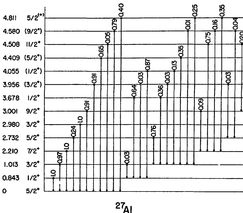
Fig. 21. Energy-level decay scheme for ^{27}\text{Al} . Note that the energy scale is distorted.
