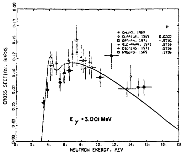
Fig. 47. Measured and evaluated ^{27}\text{Al}(n,n'\gamma) cross section for the 3.001-MeV photon from the 3.001 + 0 -MeV transition in ^{27}\text{Al} .
