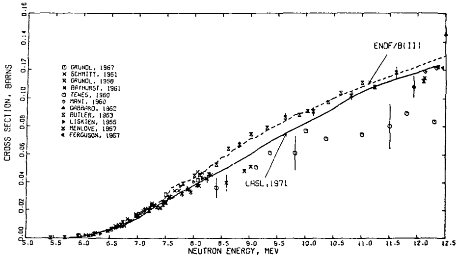
Fig. 39. Measured and evaluated ^{27}\text{Al}(n,\alpha)^{24}\text{Na} cross section from 5.0 to 12.5 MeV.
