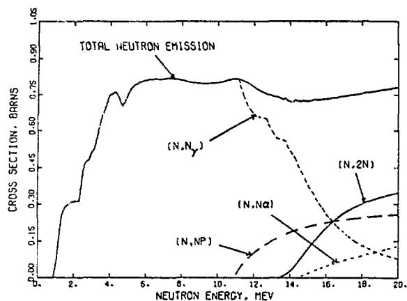
Fig. 34. The total neutron-emission cross section compared to its constituent (n,n_\gamma) , (n,np) , (n,n\alpha) , and (n,2n) reactions. The (n,n_\gamma) curve is defined as that part of the (n,n') cross section which results in photon emission.
