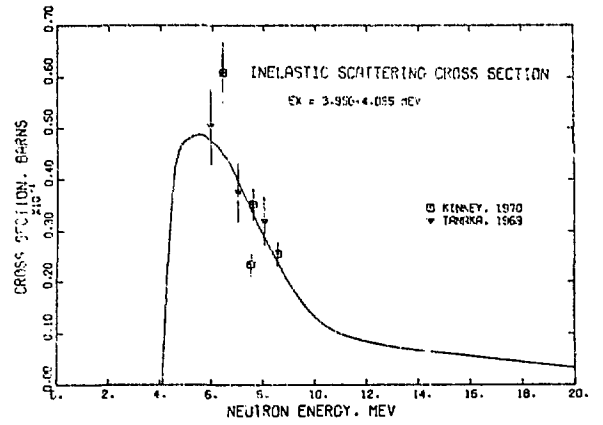
Fig. 29. Measured and evaluated inelastic-scattering cross section to the combined 3.956- and 4.055-MeV levels of ^{27}\text{Al} .
