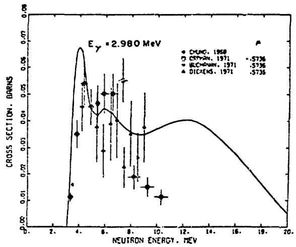
Fig. 46. Measured and evaluated ^{27}\text{Al}(n,n'\gamma) cross section for the 2.980-MeV photon from the 2.980 \rightarrow 0-MeV transition in ^{27}\text{Al} .
