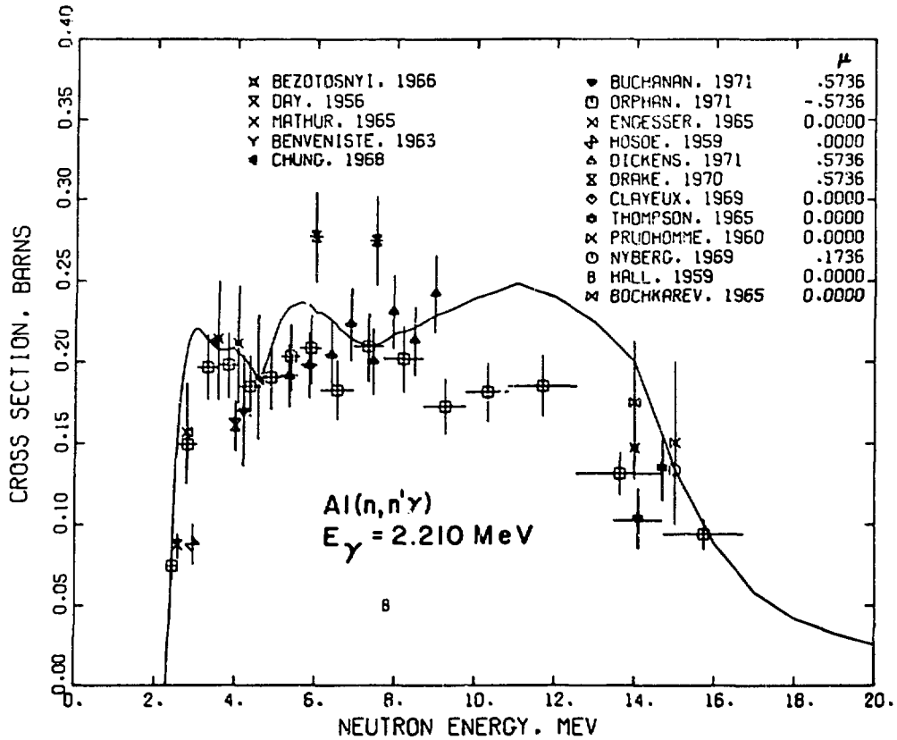
Fig. 44. Measured and evaluated ^{27}\text{Al}(n,n'\gamma) cross section for the 2.210-MeV photon from the 2.210 \rightarrow 0-MeV transition in ^{27}\text{Al} .
