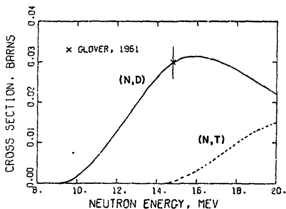
Fig. 38. Evaluated ^{27}\text{Al}(n,d)^{26}\text{Mg} and ^{27}\text{Al}(n,t)^{25}\text{Mg} cross sections compared to the (n,d) measurement by Glover (G161).
