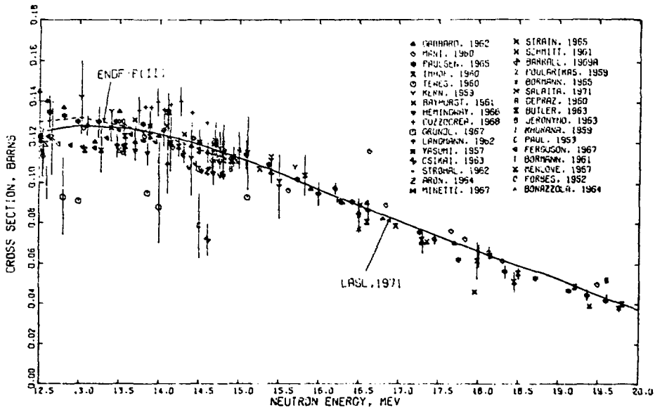
Fig. 40. Measured and evaluated ^{27}\text{Al}(n,\alpha)^{24}\text{Na} cross section from 12.5 to 20 MeV.
