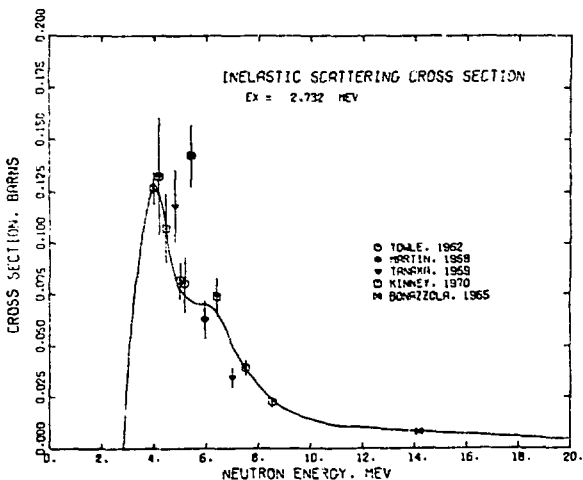
Fig. 24. Measured and evaluated inelastic-scattering cross section to the 2.732-MeV level of ^{27}\text{Al} .
