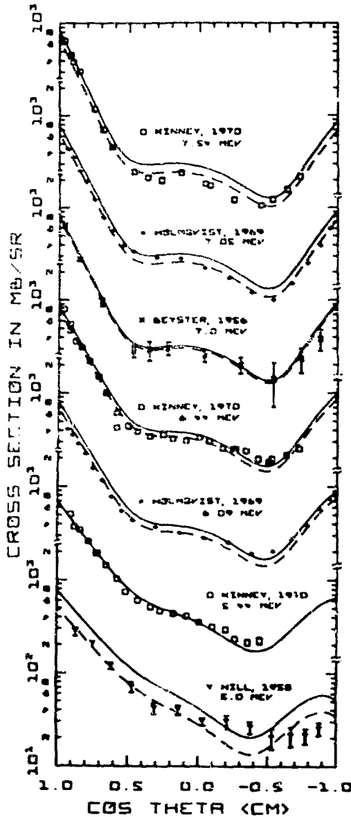
Fig. 58. Measured and evaluated angular distributions for elastic scattering from 5.0 to 7.54 MeV. See caption to Fig. 56 for details.
