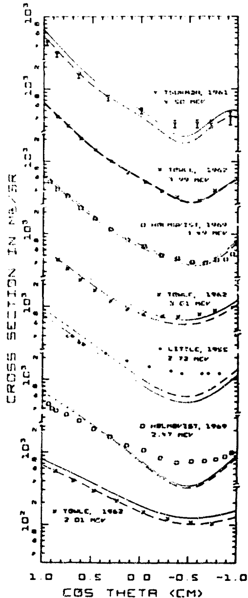
Fig. 57. Measured and evaluated angular distributions for elastic scattering from 2.01 to 4.50 MeV. See caption to Fig. 56 for details.
