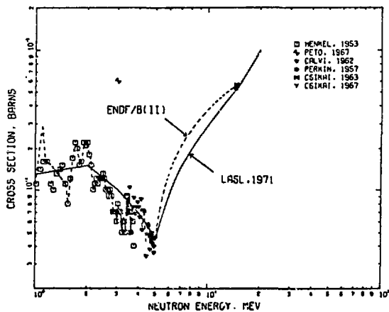
Fig. 20. Measured and evaluated ^{27}\text{Al}(n,\gamma)^{28}\text{Al} cross section from 1 to 20 MeV.
