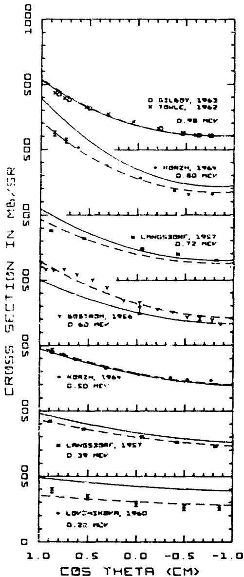
Fig. 56. Measured and evaluated angular distributions for elastic scattering from 0.22 to 0.98 MeV. The dashed curves represent the evaluated shapes normalized to the measurements; the solid curve gives the same shapes normalized to the evaluated elastic cross sections.
