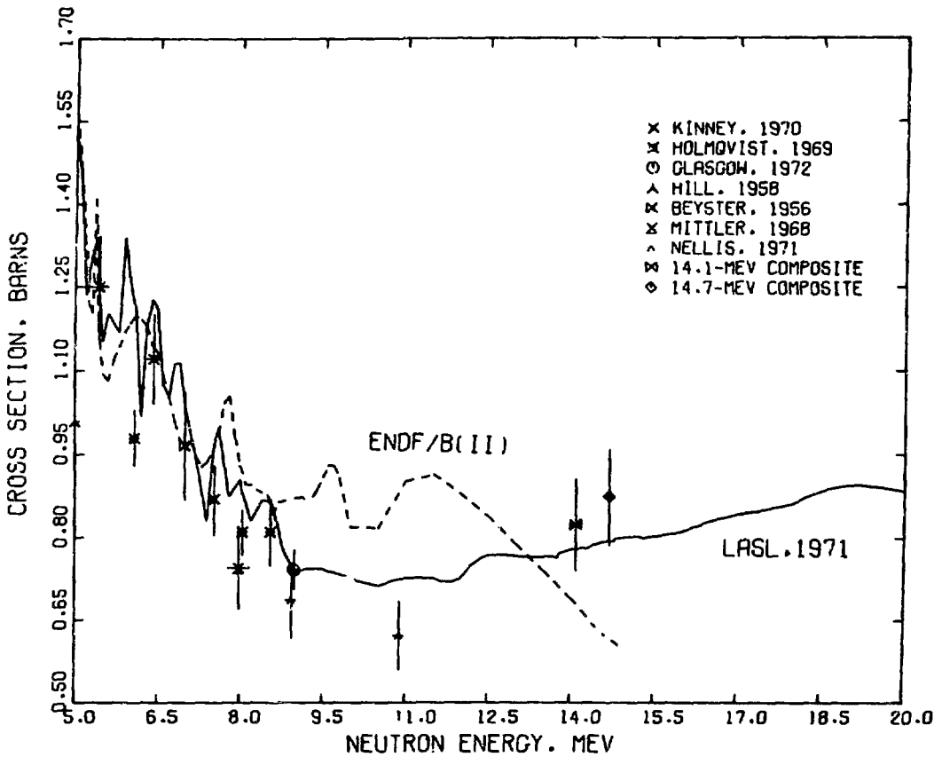
Fig. 14. Measured and evaluated elastic scattering cross section for ^{27}\text{Al} from 5 to 20 MeV. The 14.1-MeV point was obtained by fitting a composite of measurements near that energy (Bo65a, Co58, Sa59, St65, Yu58); similarly, the 14.7-MeV point results from three measurements near that energy (An59, Ba58, Kh58). The composites are shown in Fig. 59.
