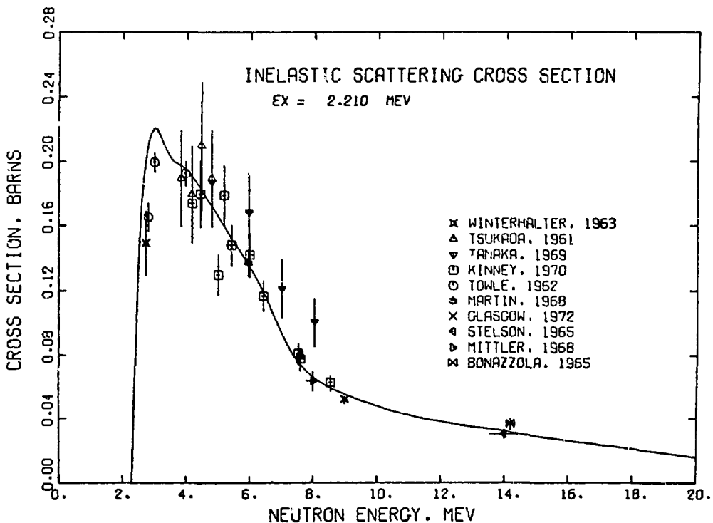
Fig. 23. Measured and evaluated inelastic-scattering cross section to the 2.210-MeV level of ^{27}\text{Al} .
