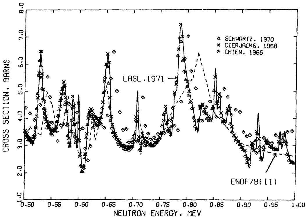
Fig. 4. Measured and evaluated total cross section for ^{27}\text{Al} from 0.5 to 1.0 MeV. The experimental data are averages of 6 points for the Schwartz (Sc70) results, 10 points for Cierjacks (Ci68), and 5 points for Chien (Ch66).
