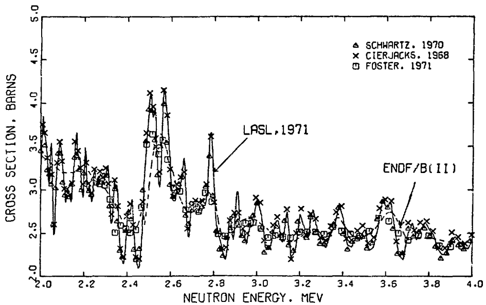
Fig. 6. Measured and evaluated total cross section for ^{27}\text{Al} from 2 to 4 MeV. The experimental data are averages of 5 points for the Schwartz (Sc70) results, 8 points for Cierjacks (Ci68), and 2 points for Foster (Fo71).
