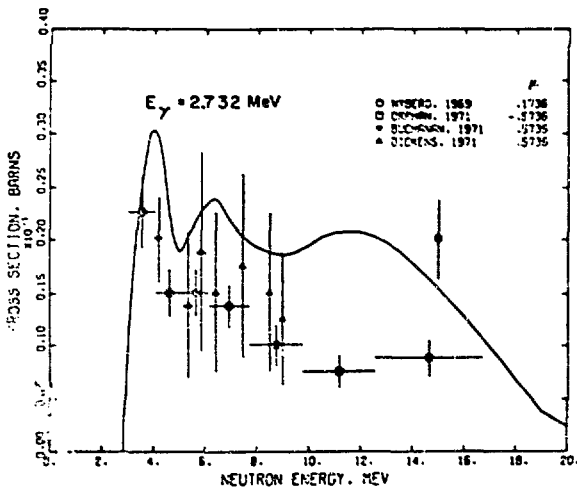
Fig. 45. Measured and evaluated ^{27}\text{Al}(n,n'\gamma) cross section for the 2.732-MeV photon from the 2.732 \rightarrow 0-MeV transition in ^{27}\text{Al} .
