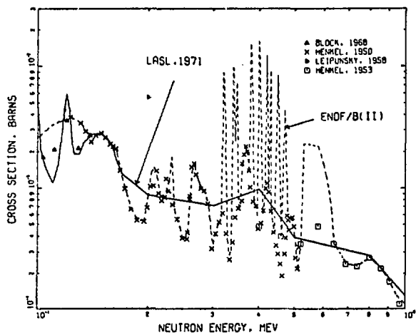
Fig. 19. Measured and evaluated ^{27}\text{Al}(n,\gamma)^{28}\text{Al} cross section from 0.1 to 1.0 MeV.
