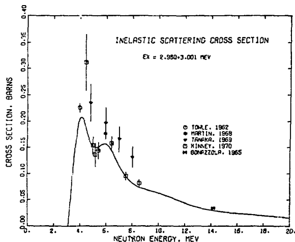
Fig. 26. Measured and evaluated inelastic-scattering cross section to the combined 2.980- and 3.001-MeV levels of ^{27}\text{Al} .
