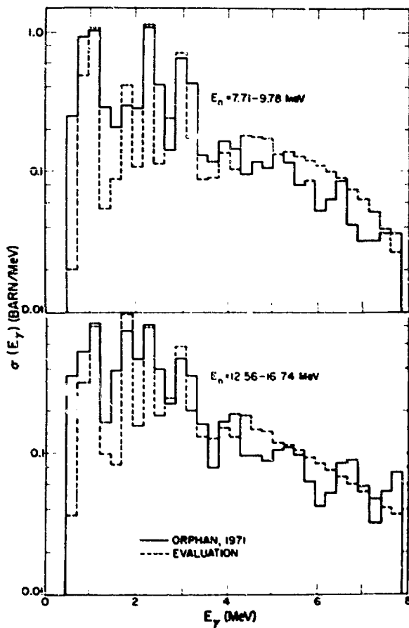
Fig. 54. Measured and evaluated photon energy spectra from all reactions averaged over the neutron energy regions 7.71-9.78 MeV and 12.56-16.74 MeV.
