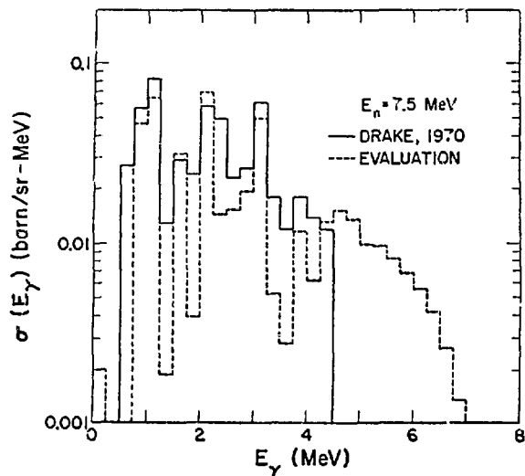
Fig. 53. Measured and evaluated photon energy spectra from all reactions at E_n = 7.5 MeV.
