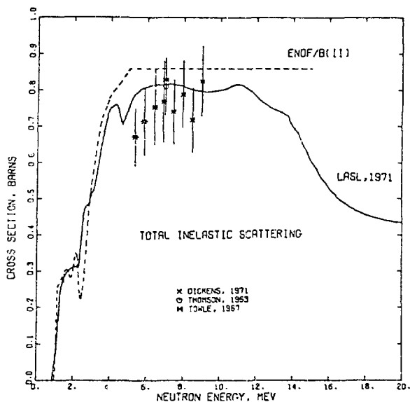
Fig. 32. Measured and evaluated total inelastic-scattering cross section for ^{27}\text{Al} . The (n,np) and (n,n\alpha) reactions are included.
