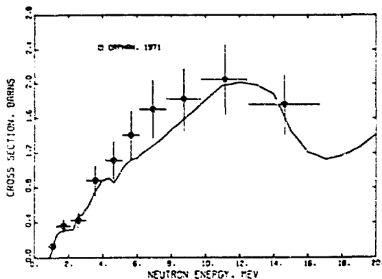
Fig. 55. Measured and evaluated total photon-production cross section from all ^{27}\text{Al}(n,xy) reactions.
