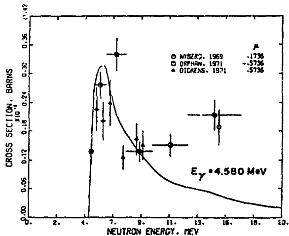
Fig. 50. Measured and evaluated ^{27}\text{Al}(n,n'\gamma) cross section for the 4.580-MeV photon from the 4.580 + 0 -MeV transition in ^{27}\text{Al} .
