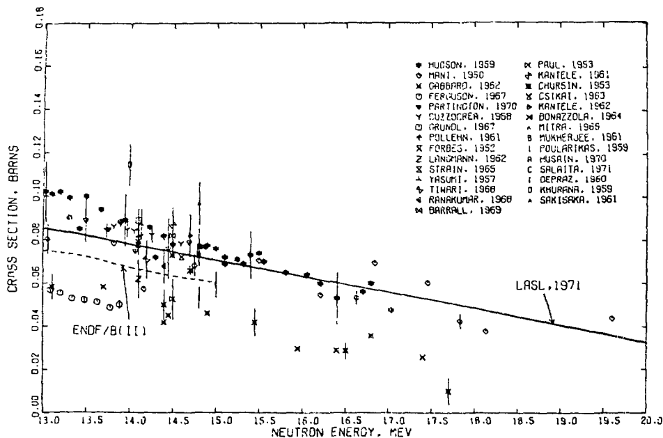
Fig. 37. Measured and evaluated ^{27}\text{Al}(n,p)^{27}\text{Ng} cross section from 13 to 20 MeV.
