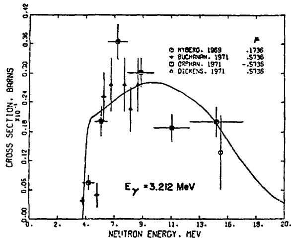
Fig. 49. Measured and evaluated ^{27}\text{Al}(n,n'\gamma) cross section for the 3.212-MeV photon from the 4.055 + 0.843 -MeV transition in ^{27}\text{Al} .
