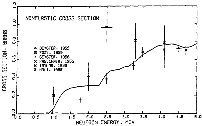
Fig. 13. Measured and evaluated nonelastic cross section for ^{27}\text{Al} from 0.5 to 5.0 MeV.
