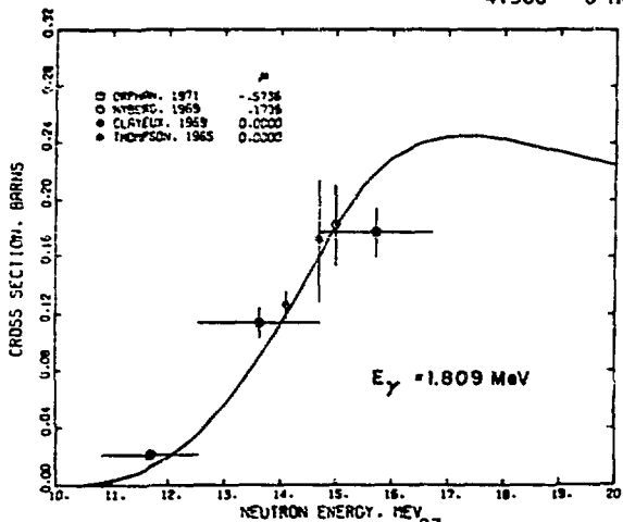
Fig. 51. Measured and evaluated ^{27}\text{Al}(n,x\gamma) cross section for the 1.809-MeV photon from the 1.809 + 0 -MeV transition in ^{26}\text{Mg} .
