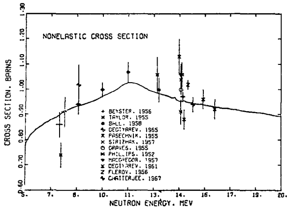
Fig. 15. Measured and evaluated nonelastic cross section for ^{27}\text{Al} from 5 to 20 MeV.
