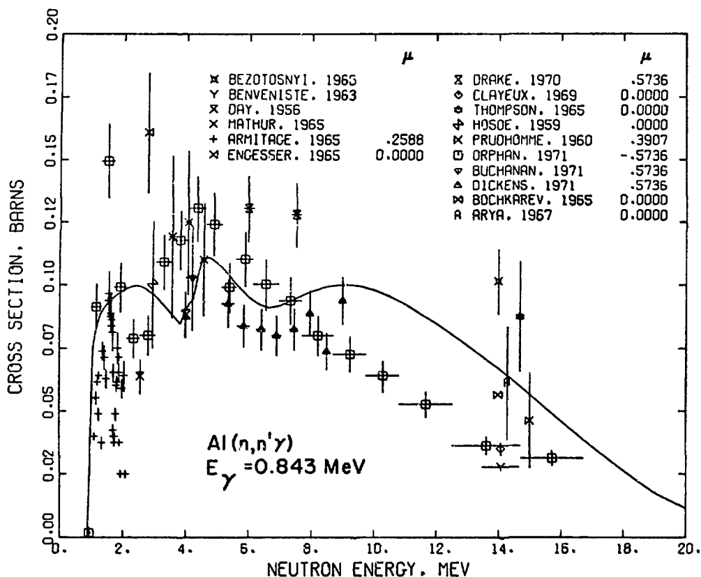
Fig. 41. Measured and evaluated ^{27}\text{Al}(n,n'\gamma) cross section for the 0.843-MeV photon from the 0.843 + 0-MeV transition in ^{27}\text{Al} .
