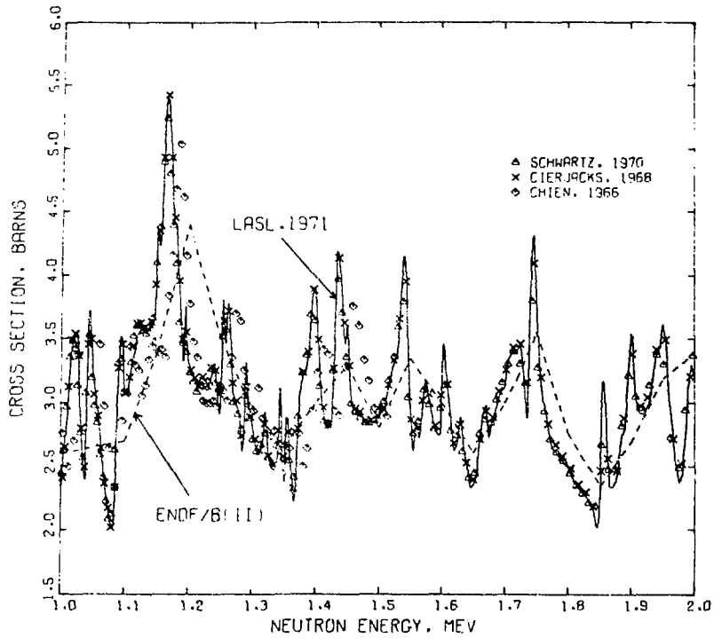
Fig. 5. Measured and evaluated total cross section for ^{27}\text{Al} from 1 to 2 MeV. The experimental data are averages of 6 points for the Schwartz (Sc70) results, 10 points for Cierjacks (Ci68), and 5 points for Chien (Ch66).
