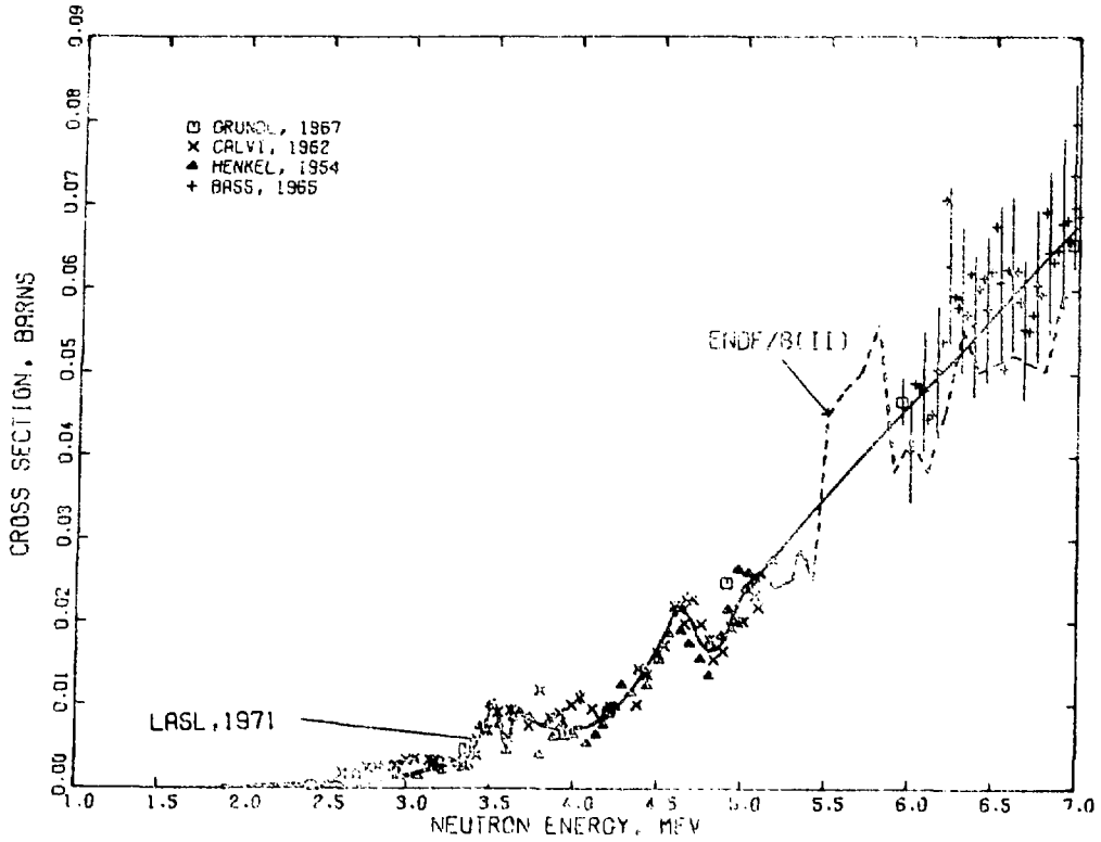
Fig. 35. Measured and evaluated ^{27}\text{Al}(n,p)^{27}\text{Mg} cross section from 1 to 7 MeV.
