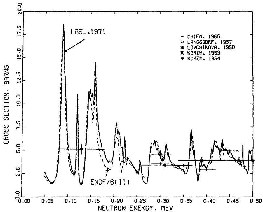
Fig. 9. Measured and evaluated elastic scattering cross section for ^{27}\text{Al} from 0.05 to 0.50 MeV.
