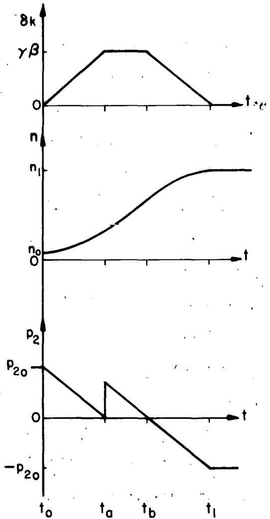
FIGURE 2.3 TIME-OPTIMAL STARTUP OF PROMPT-NEUTRON KINETICS WITH VELOCITY-LIMITED CONTROL
