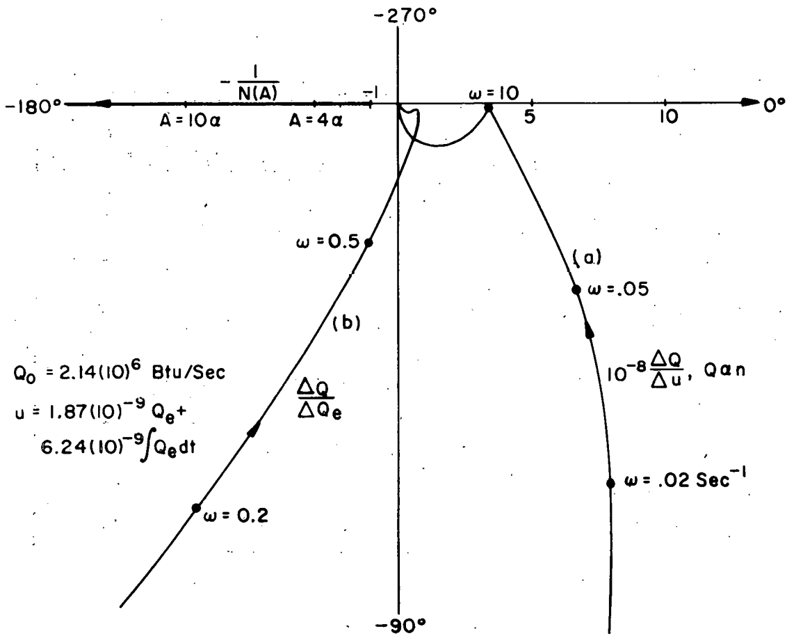
FIGURE 2.21 FREQUENCY RESPONSE OF AN OPEN-LOOP NEUTRONIC CONTROL SYSTEM - SHOWING EFFECT OF REACTIVITY LIMITING (SIX PRECURSOR MODEL)
