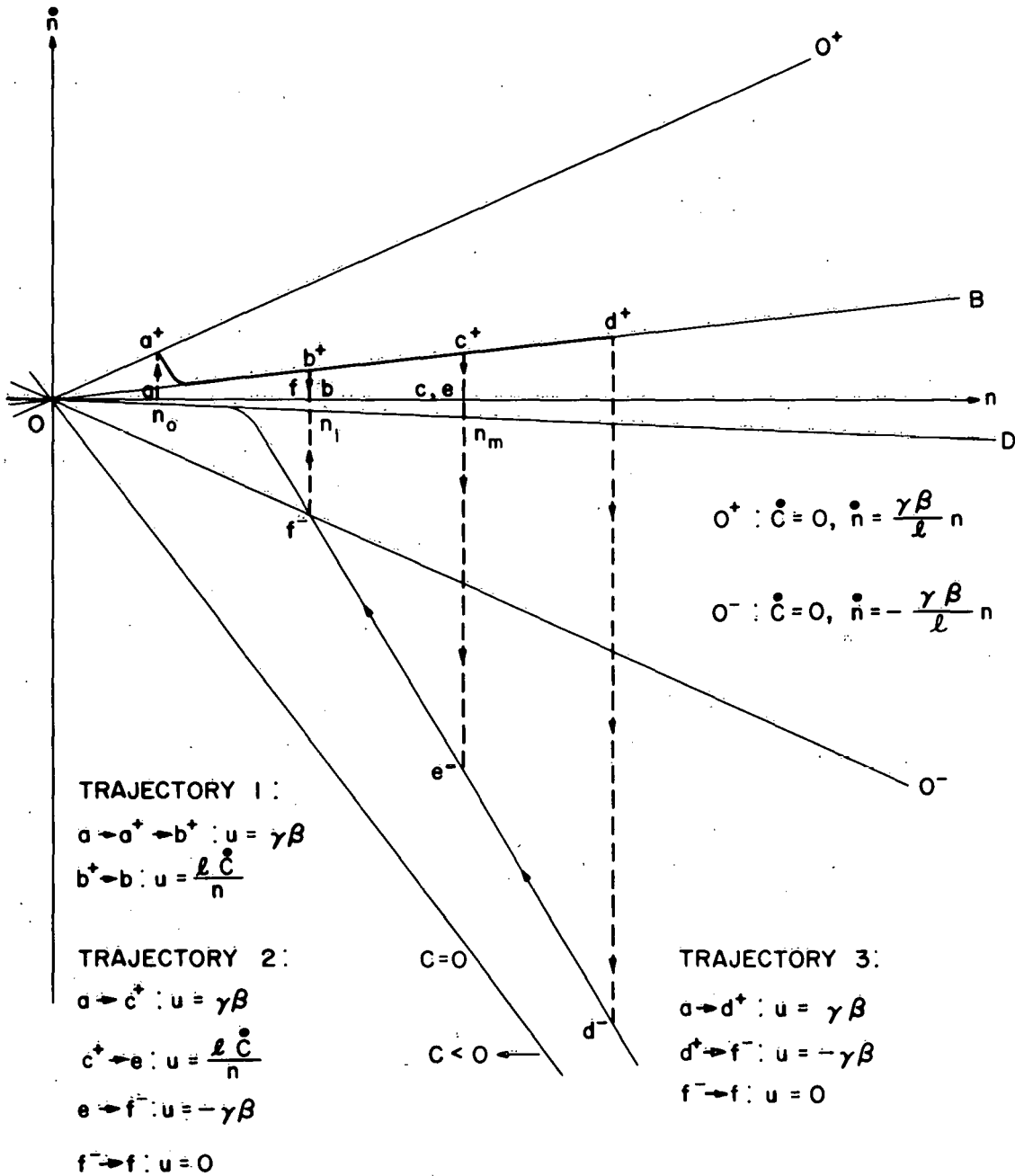
FIGURE 2.7 n VS \dot{n} BANG-BANG CONTROLLED PHASE-PLANE TRAJECTORIES (LABELLED POINTS REFER TO SIMILAR POINTS IN FIGURES 2.4 AND 2.6)
