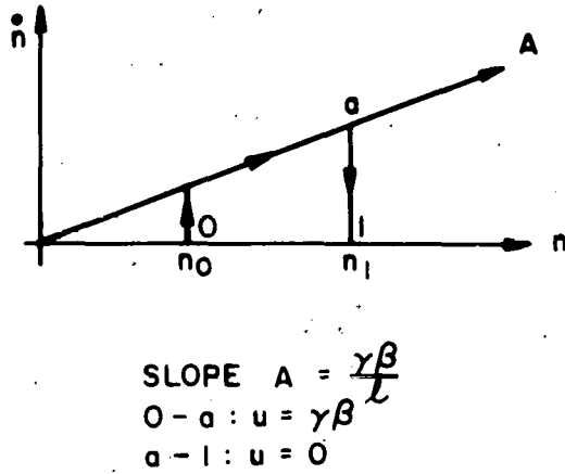
FIGURE 2.1 TIME-OPTIMAL INCREASE OF PROMPT-NEUTRON DENSITY
