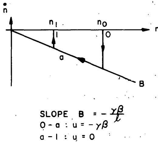
FIGURE 2.2 TIME-OPTIMAL DECREASE OF PROMPT-NEUTRON DENSITY
