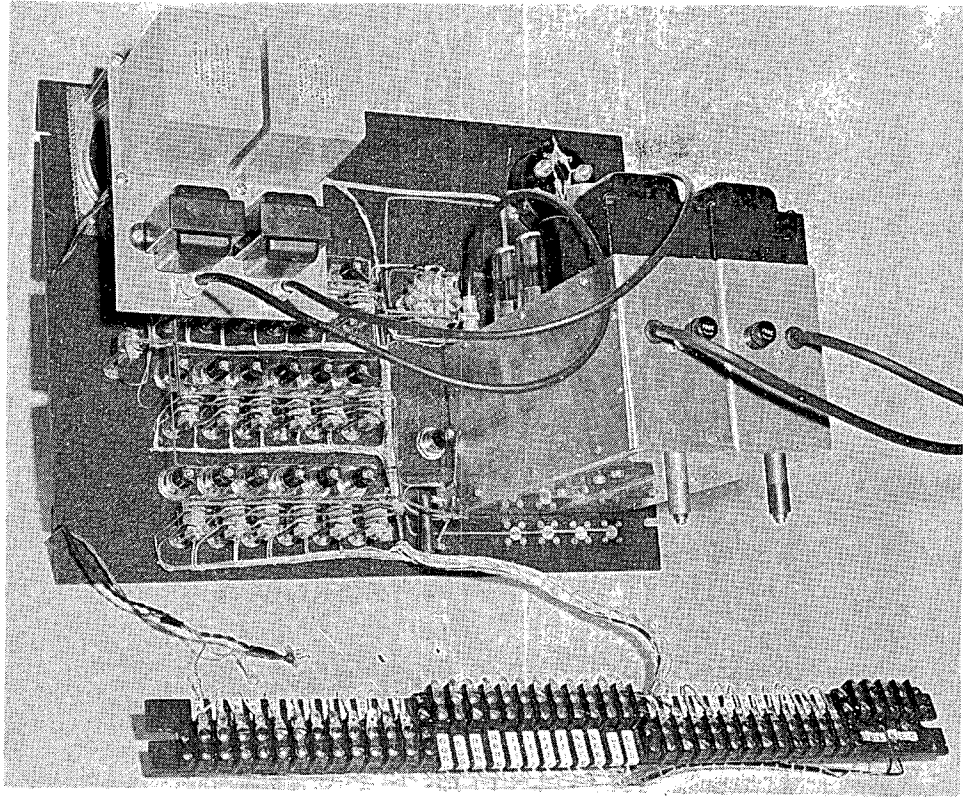
Fig. 16—Radiation-monitoring switchboard, rear view. (Front view is shown in Fig. 3.)
