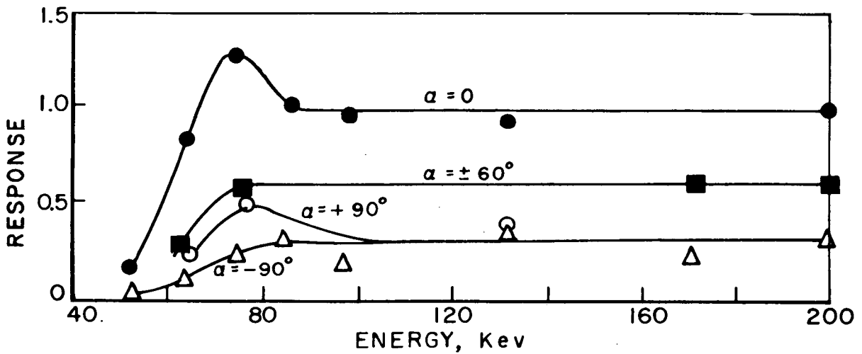
Fig. 26—Energy and directional response of LR detectors to gamma radiation.
