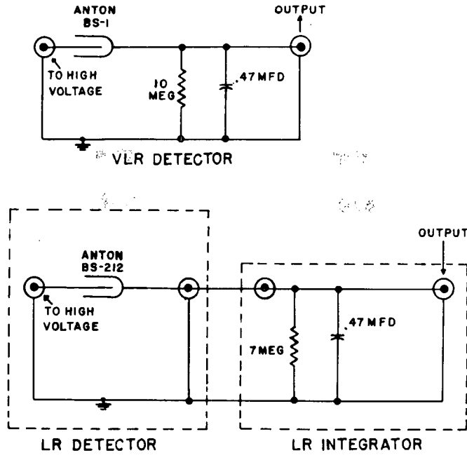
Fig. 13—Detector circuits.
