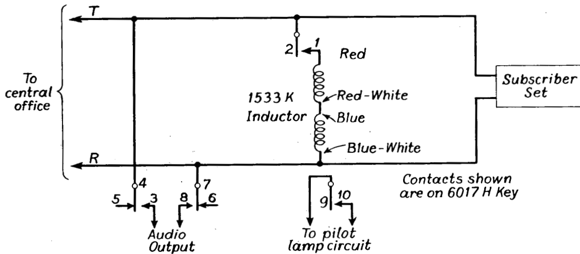
Fig. 22—Line terminating equipment, remote station (American Telephone & Telegraph Co.).
