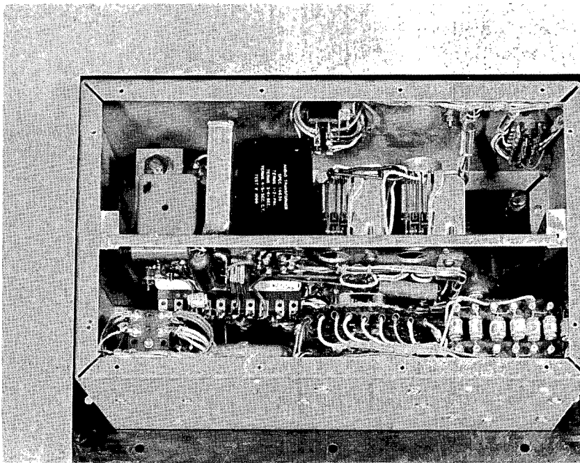
Fig. 6—Remote data station, front view.
