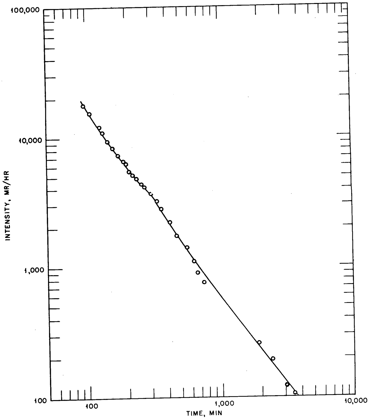
Fig. 5—Decay pattern for Butler building, center forward, shot Shasta.
