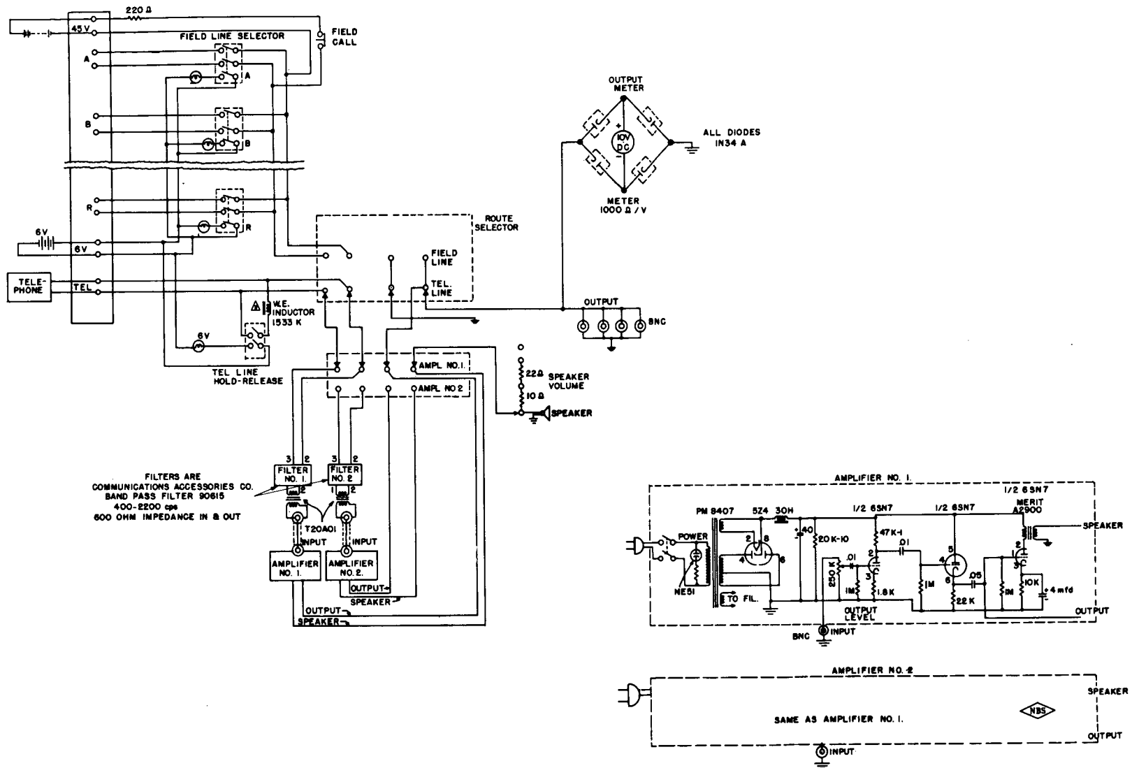
Fig. 18—Radiation-monitoring switchboard circuit diagram.
