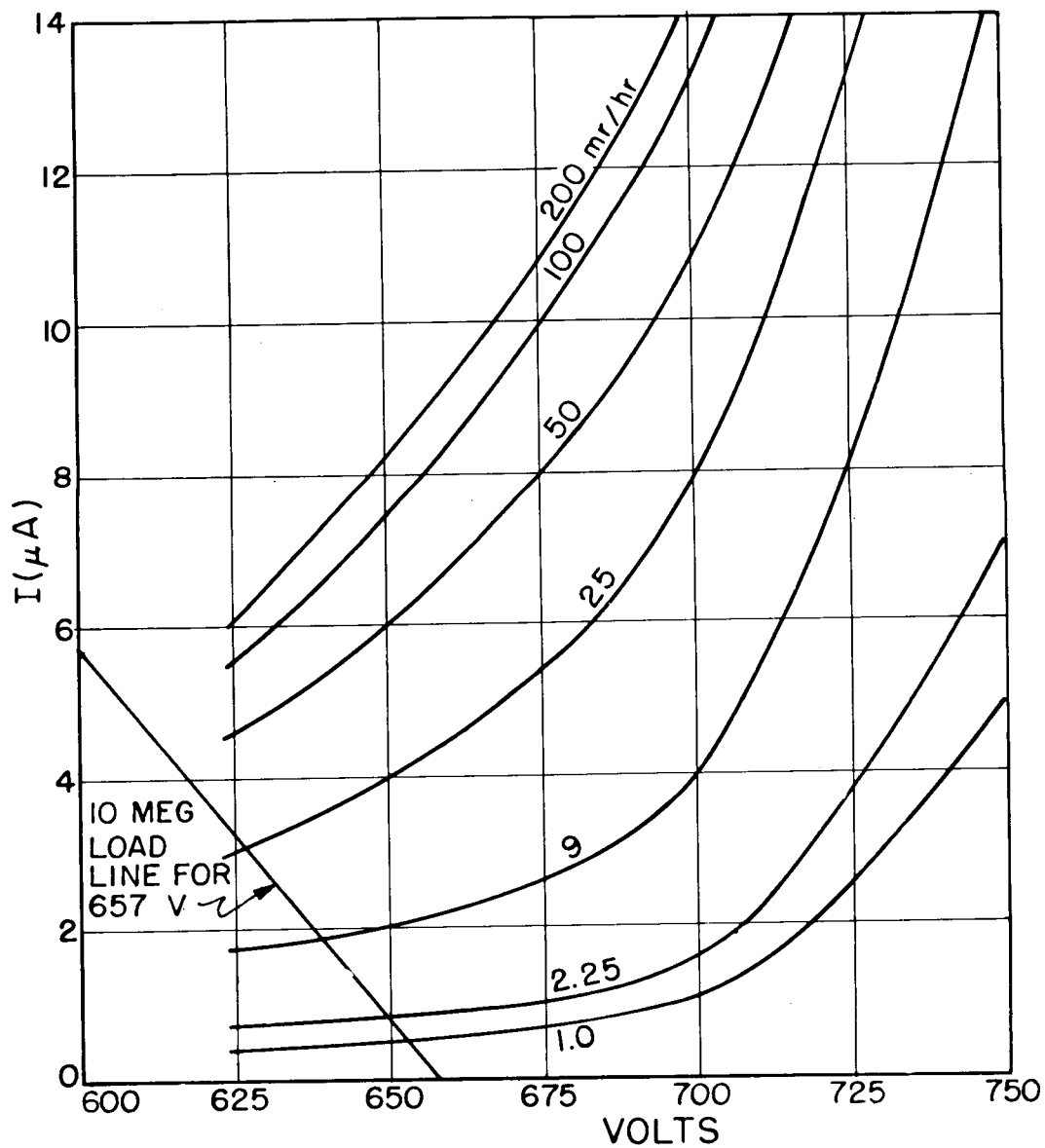
Fig. 25—Voltage-current characteristic of BS-1 counter tube (Anton).
