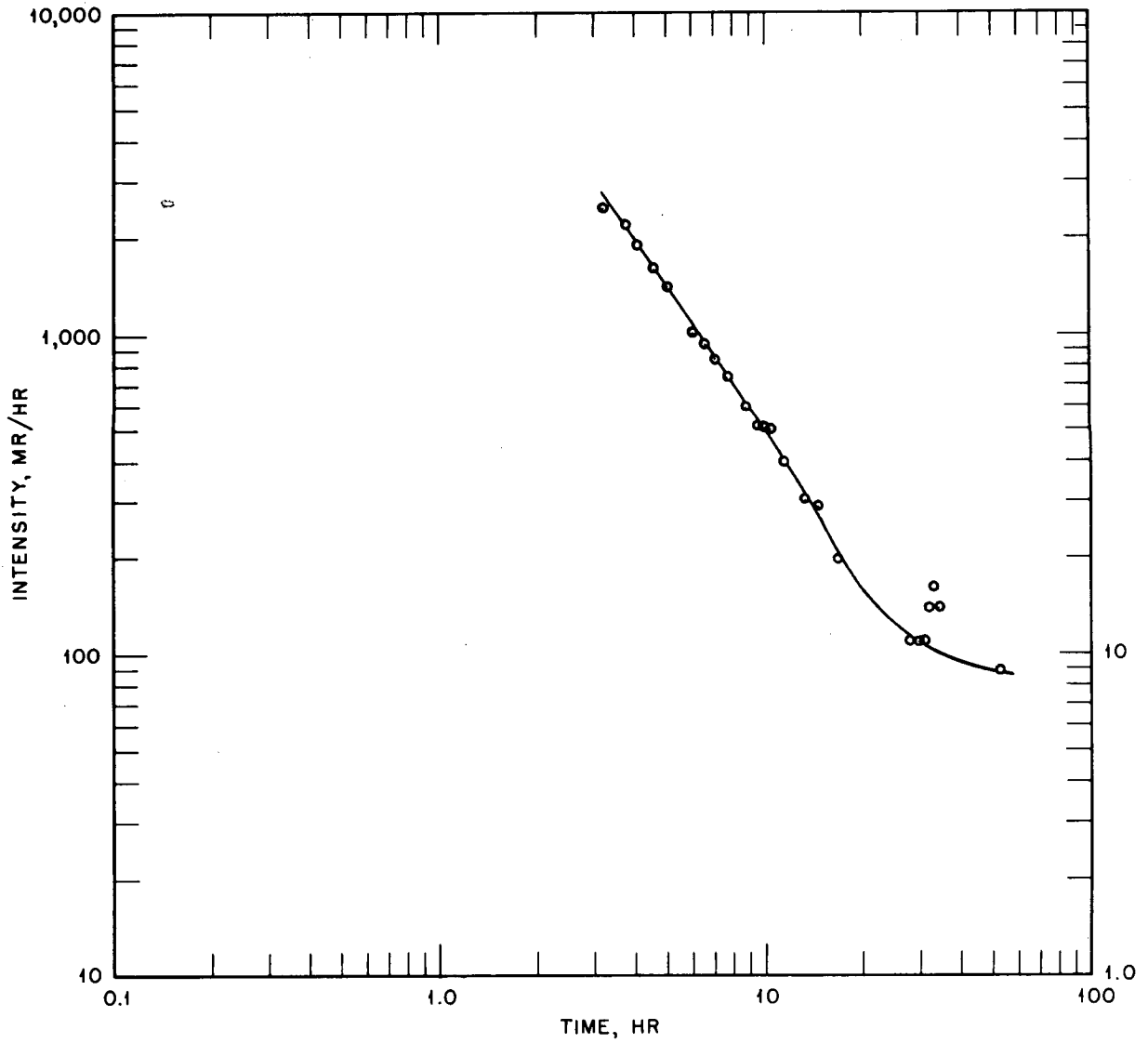
Fig. 17—Decay pattern for Project 32.3 manned shelter, left pad, shot Diablo.
