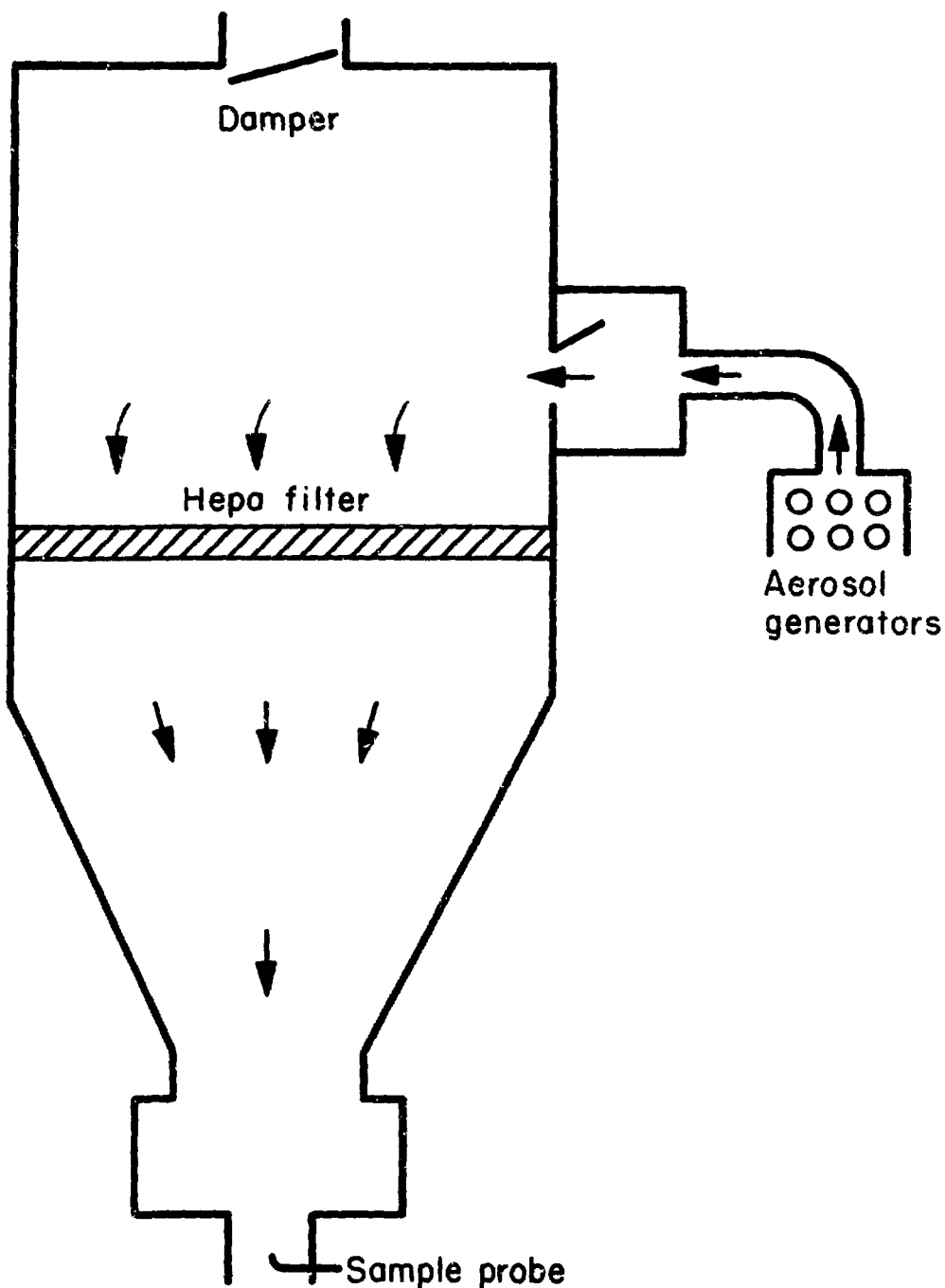
"Figure 5", DP West room air exhaust system.
