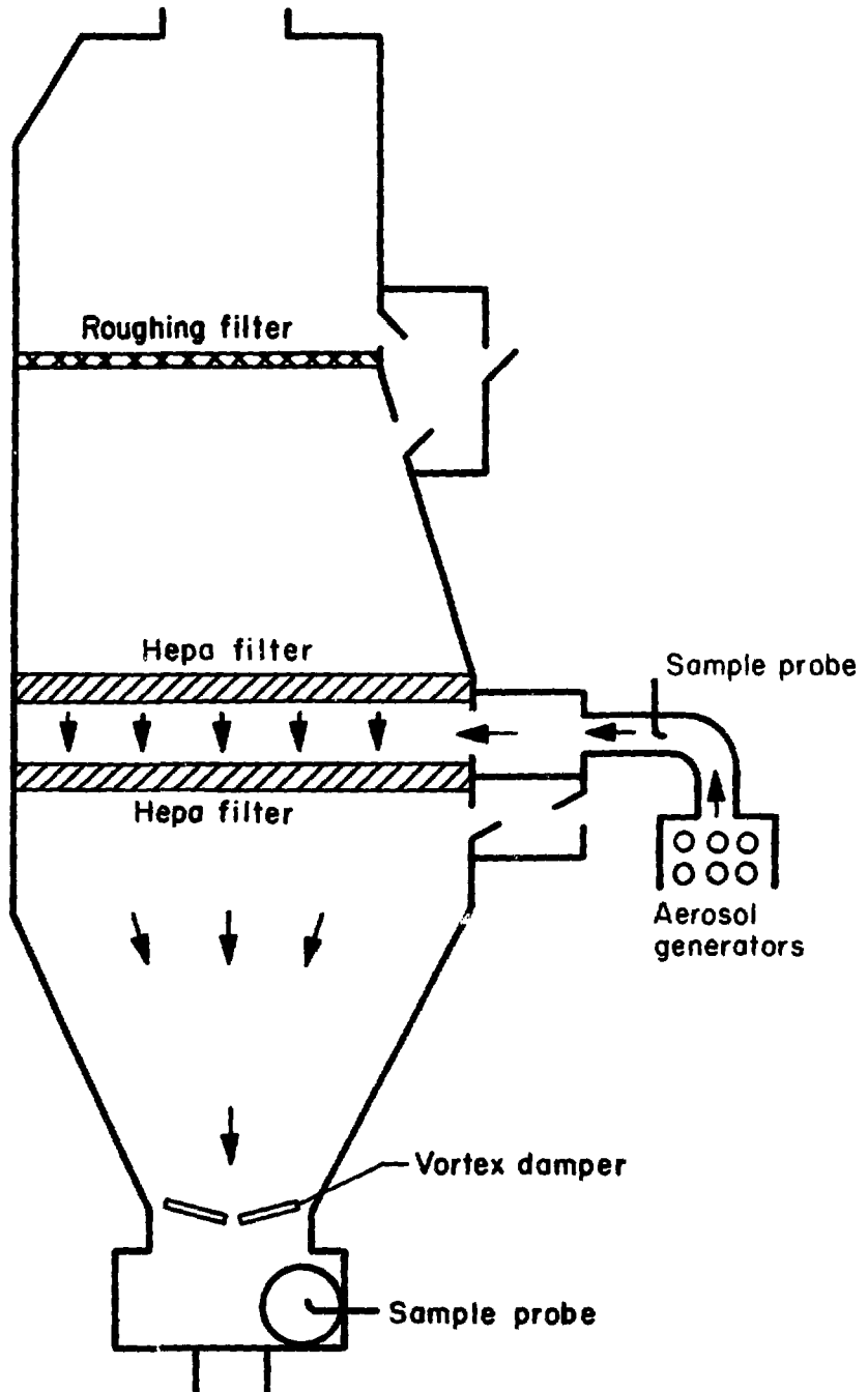
"Figure 10", DOP Testing of the second stage of filter.
