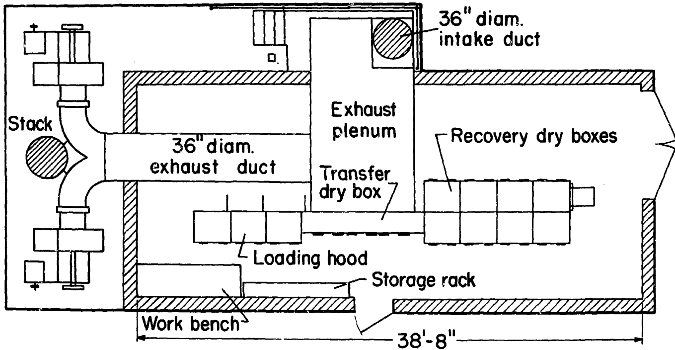
Filter house layout
