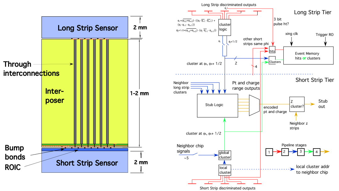
Figure 2. a) Conceptual drawing of a 3D-based stack. Analog signals flow from the top long strip sensor through the interposer to the readout IC (ROIC) bonded to the bottom sensor. b) Schematic of on-chip cluster and stub formation. Event memory is associated with the long strips.
