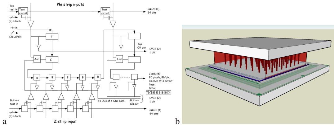
Figure 3. a) Schematic drawing of the VICTR chip. The 5 Z strips on the bottom tier are anded with the long phi strip on the top tier. b) Conceptual drawing of the VICTR-based 3D module stack. The interposer is transparent showing the 8 \times 8 array of vias from the top sensor to the VICTR (which is outlined in blue). The active areas of the sensors are approximately 5 \times 5 mm.
