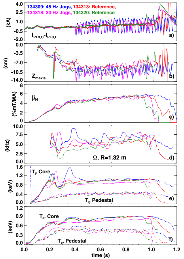
Figure 4. Compatibility of jogging with high-performance operation in NSTX. Shown are (a) the difference in radial-field coil currents I_{PF3,U} - I_{PF3,L} , (b) the axis location z_{maxis} , (c) the normalized beta \beta_N , (d) the toroidal rotation frequency \Omega at a radius ( R = 1.32 m) near the q = 2 surface, (e) the core and pedestal ion temperature and (f) the core and pedestal electron temperature.
