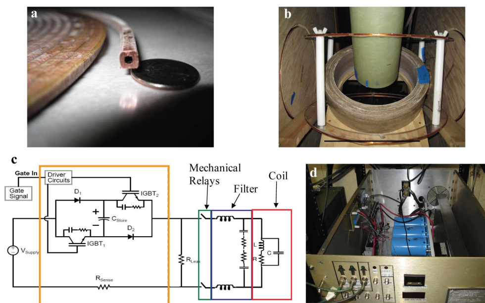
Figure 3.2: Images and schematics of water cooled coil and associated switching electronics. a. Image of square-hollow copper tube cross section. Quarter included for scale. b. Image of prepolarizing coil in the MRI system. The outer diameter of the coil is 0.413 m. c. Schematic prepolarizing circuit with switching electronics (orange box), mechanical relays (green) filter (blue) and coil (red) indicated. d. Picture of assembled switcher box. Capacitors are blue cylinders, connected to low-inductance bus (green/white bar). IGBTs and diodes are black objects visible between low-inductance bus and aluminum heat sink.
