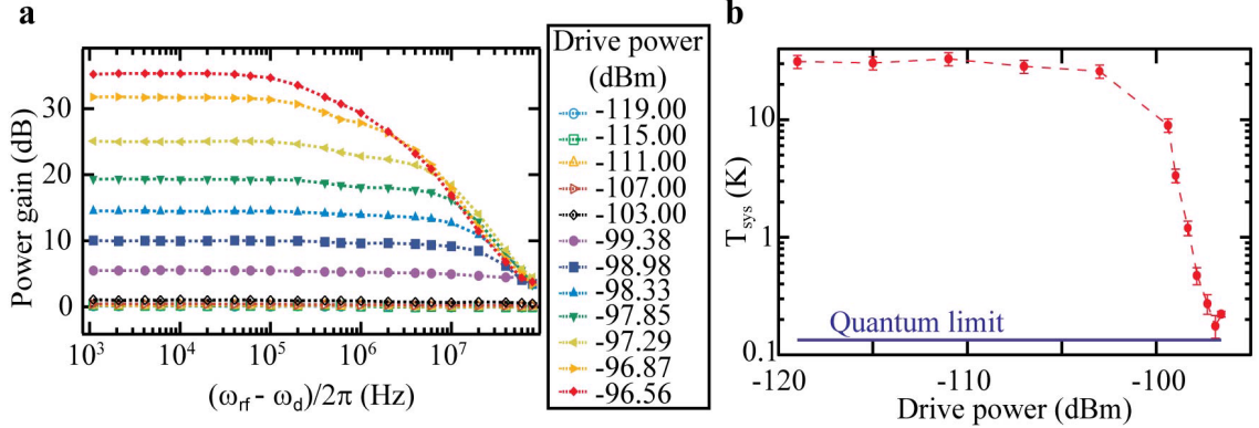
Figure 5.7: Device parametric gain and system noise temperature. a. The parametric gain of rf signals applied in combination with an rf drive tone versus the offset frequency (\omega_{rf} - \omega_d)/2\pi . Each curve is identified by the applied microwave power of the drive tone at the plane of the resonator. For low drive powers ( < -103 dBm) the resonator response is linear, and consequently the parametric gain is 0 dB. At higher drive powers, the drive power was chosen so that maximum gain was achieved at a given drive frequency, as the drive frequency was decreased from 5.778 GHz at parametric gain of 0 dB to 5.556 GHz at 35 dB gain. b. System noise temperature (K) vs. drive power (dBm). The error bars are due to uncertainty in system noise temperature in the absence of parametric gain. The standard quantum limit ( T_{sys} = 0.14 K at \omega/2\pi = 5.56 GHz) is shown in blue. At 32 dB gain the device is nearly quantum limited.
