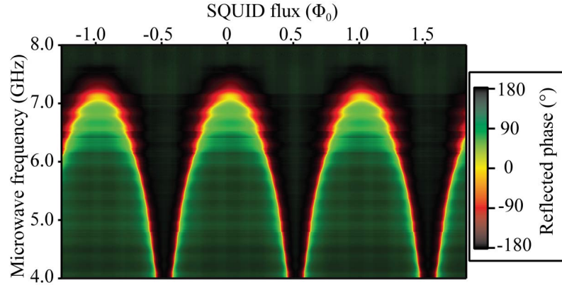
Figure 5.5: Resonator response to static flux. The phase of the reflected microwave drive is plotted versus applied SQUID flux and drive frequency. The periodicity of the SQUID inductance versus flux is evident in the pattern of reflected phase.
