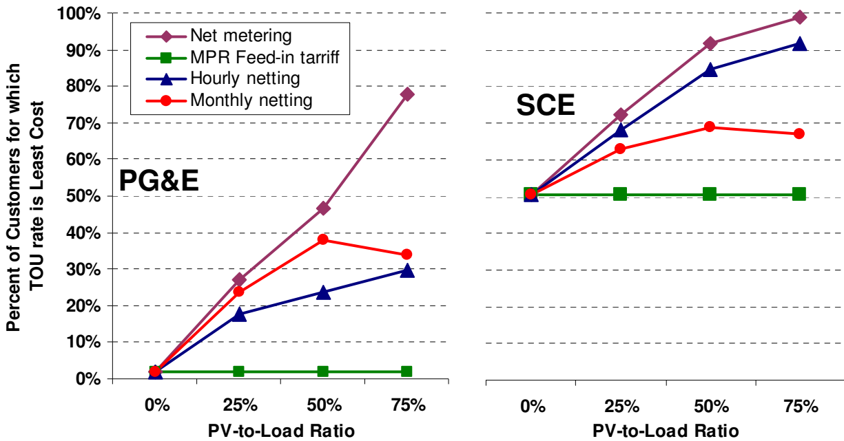
Figure 19. Least-Cost Rate Choice under Alternative PV Compensation Mechanisms
