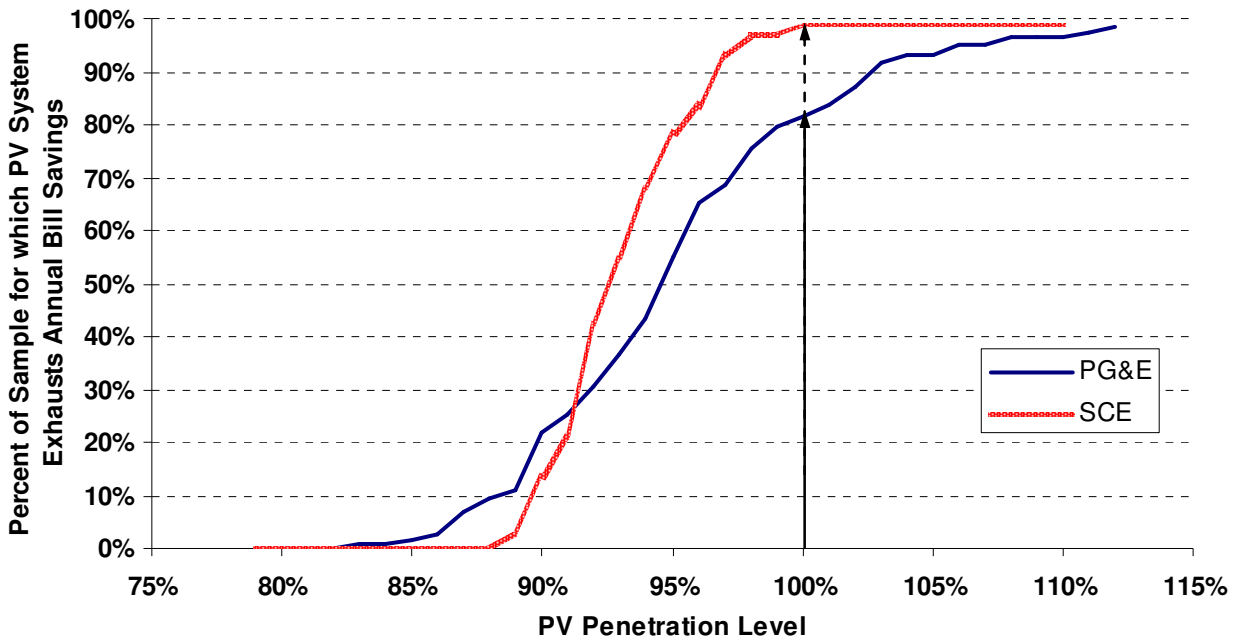
Figure 17. PV System Size that Exhausts Annual Bill Savings
