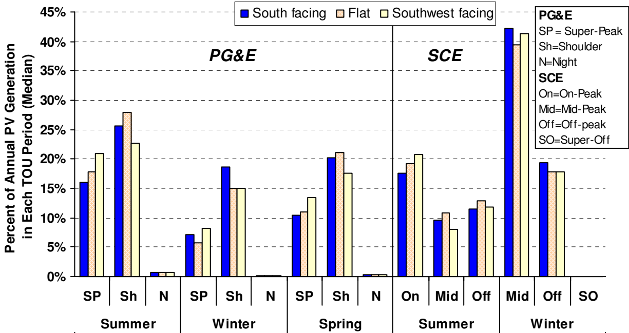
Figure 6. Distribution of PV Electricity Generation by MPR-TOD Period
