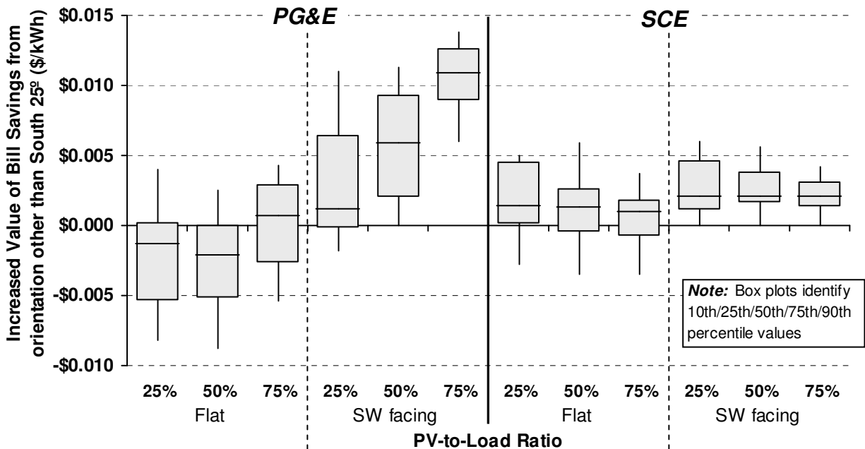
Figure 15. Difference in Bill Savings between Alternate and Base-Case PV Orientations
