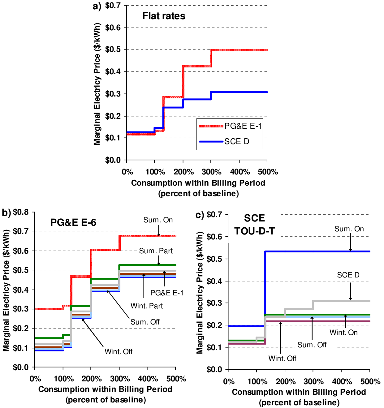
Figure 1. Prices under Current PG&E and SCE Residential Retail Rates
