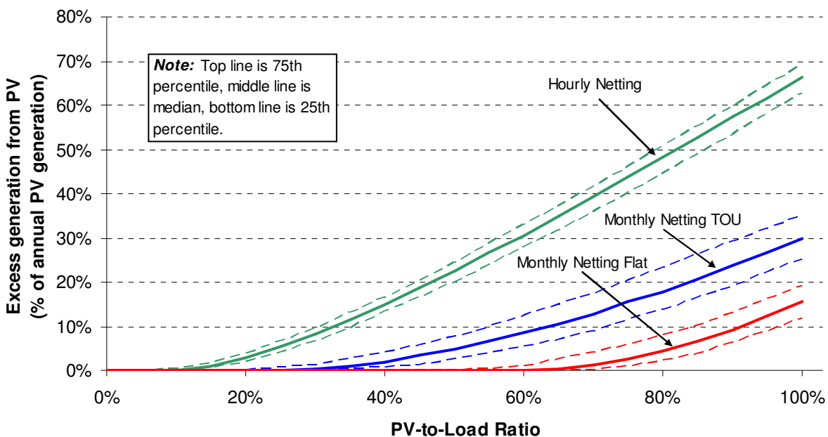
Figure 18. Net Excess PV Generation under Hourly and Monthly Netting Options
