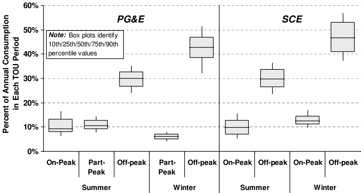
Figure 4. Customer Load Distribution by TOU Period
