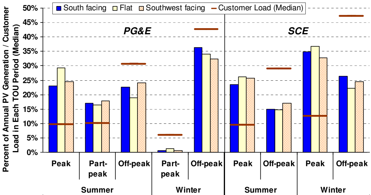
Figure 5. Distribution of PV Electricity Generation by Retail TOU Period
