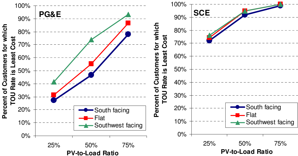
Figure 9. Least-Cost Rate Choice under Alternate PV Orientations
