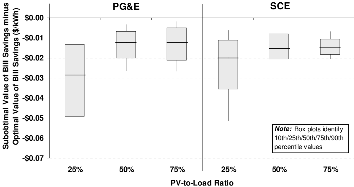
Figure 14. Distribution in the Effect of Sub-Optimal Rate Selection on the Value of Bill Savings
