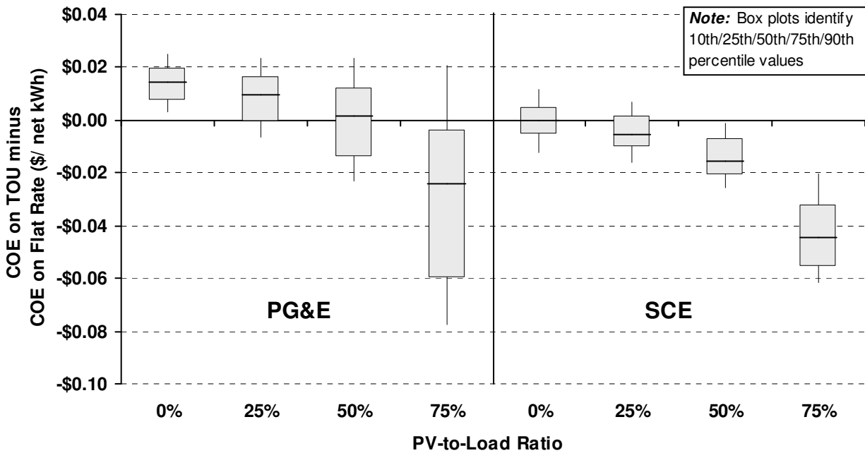
Figure 7. Difference between COE on TOU and Flat Rate
