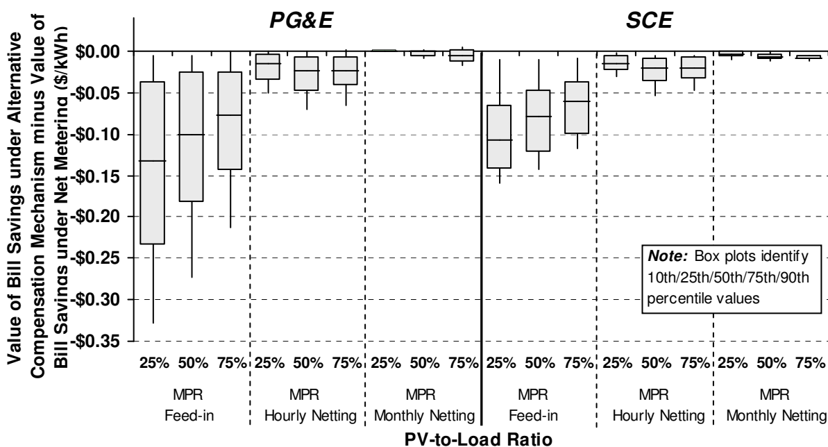
Figure 20. Difference in Bill Savings between Alternative Compensation Mechanisms and Net Metering
