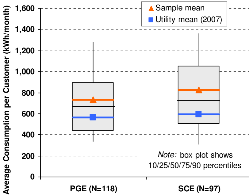
Figure 2. Distribution in Average Monthly Consumption across Customers in Data Sample 23
