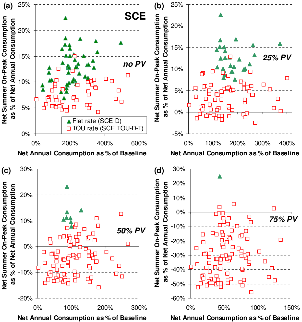
Figure 11. Customer Characteristics Associated with Least-Cost Rate Choice (SCE)
