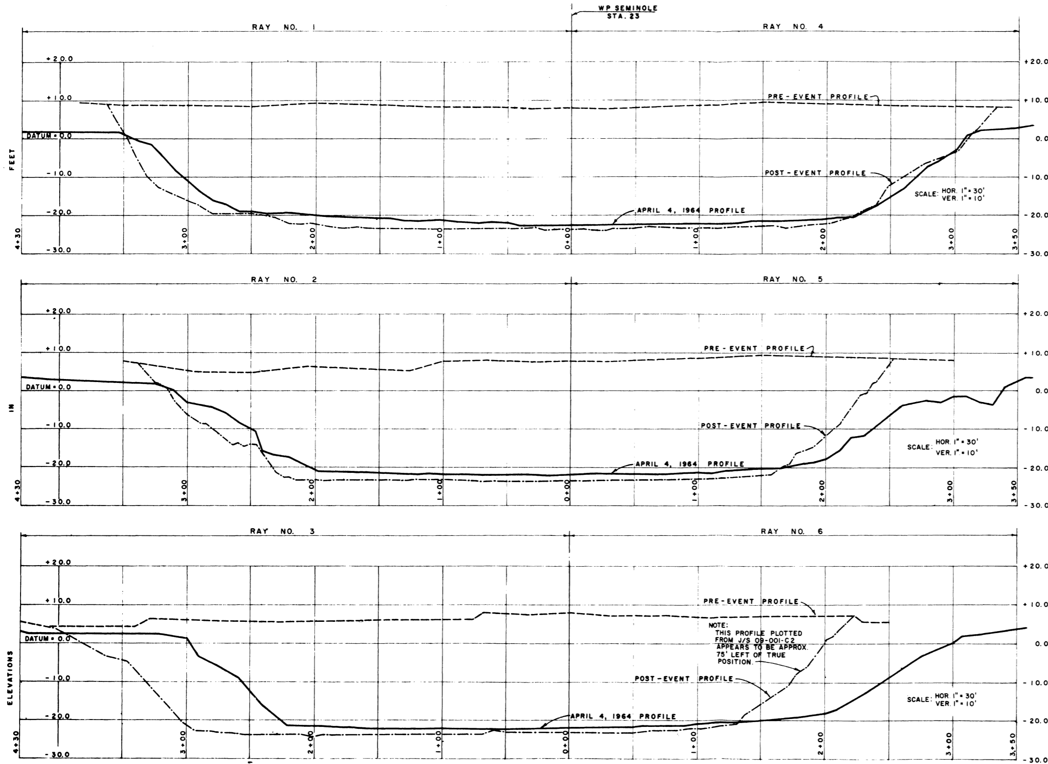
Fig. 26. Preshot, postshot, and 1964 survey profiles of Seminole crater.
