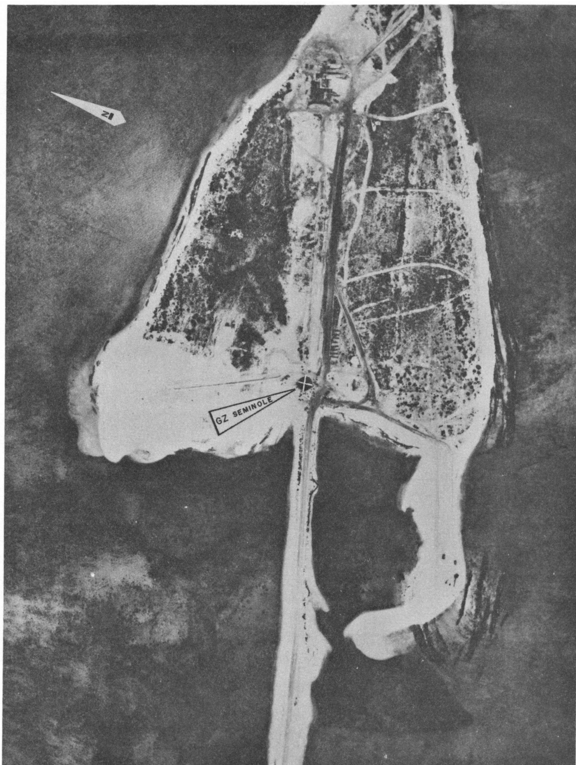
Fig. 24. Preshot Seminole area. 2
