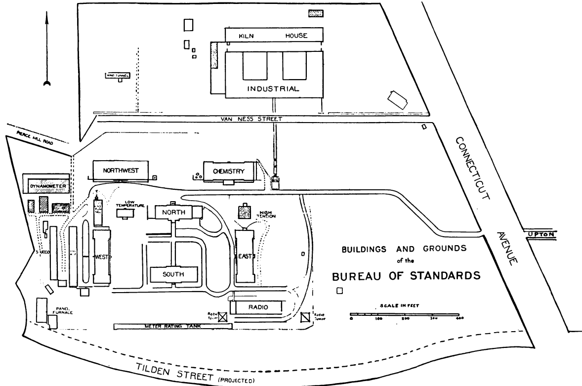
FIG. 86.—Plan of site showing location of buildings of the Bureau of Standards. (See key view on p. 112)
