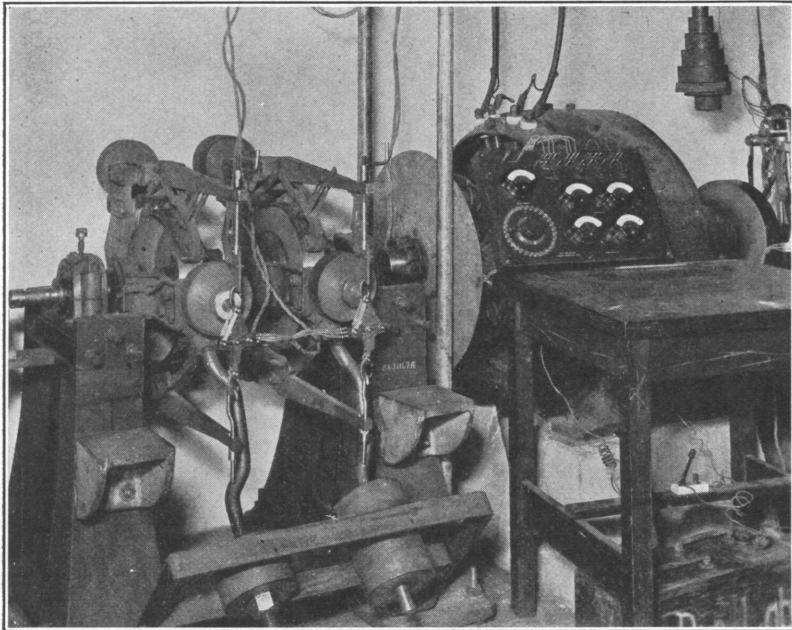
FIG. 4.— Brake-lining test equipment
