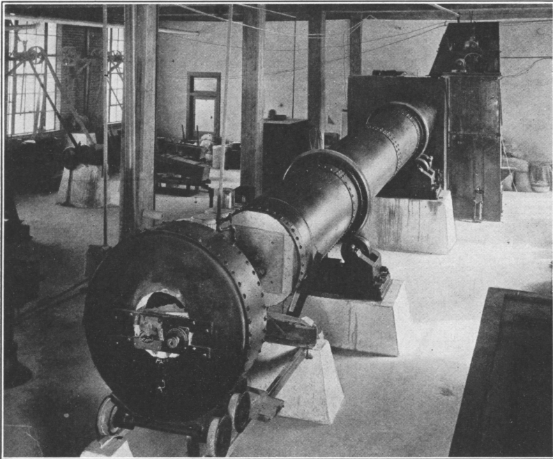
FIG. 78.— Experimental rotary cement kiln
