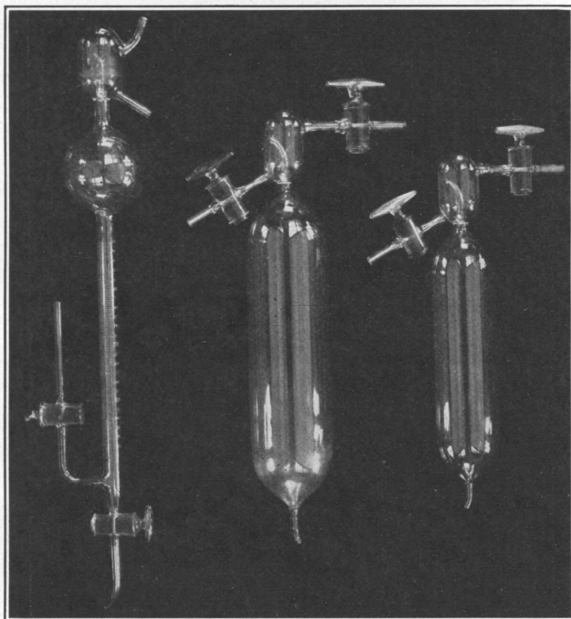
FIG. 38.— Standards of capacity
