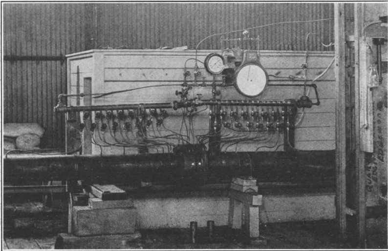
FIG. 76.— Equipment for orifice meter research
