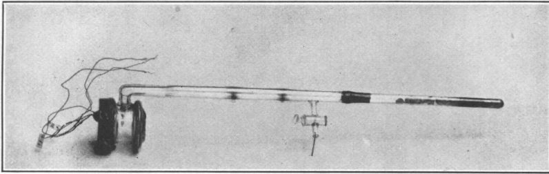
FIG. 36.— Device to record the heat of the stars and other radiation
