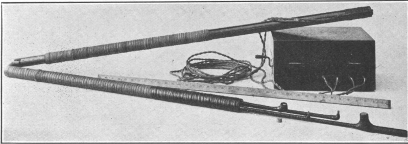
FIG. 25.— Earth current meter at the bureau
