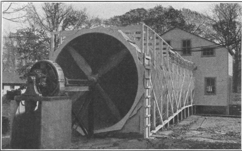
FIG. 5.— Outdoor wind tunnel
