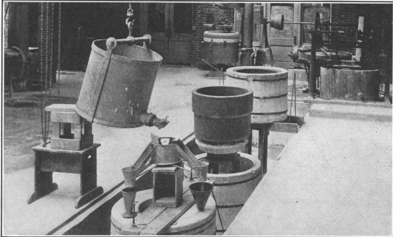
FIG. 9.— Casting clay pots
