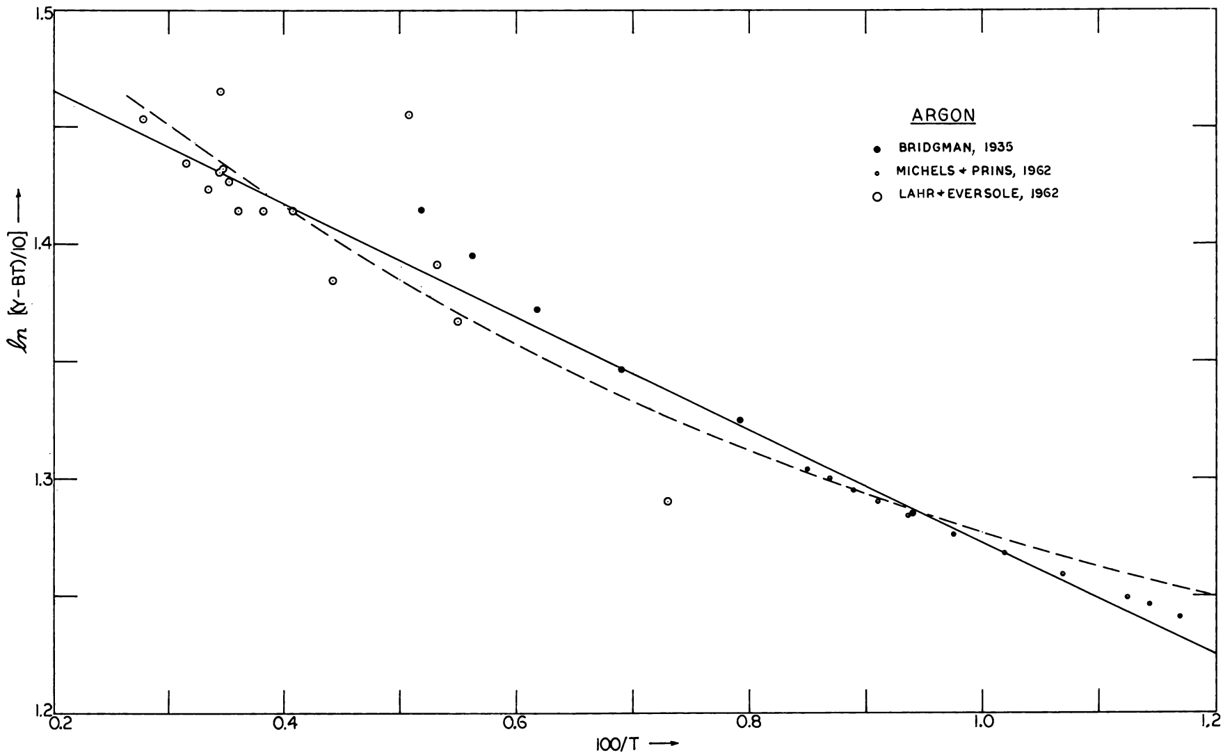
Figure 4. Logarithmic plot of equation (2) for argon using the value B = 0.06264 \text{ atm deg}^{-2} .
