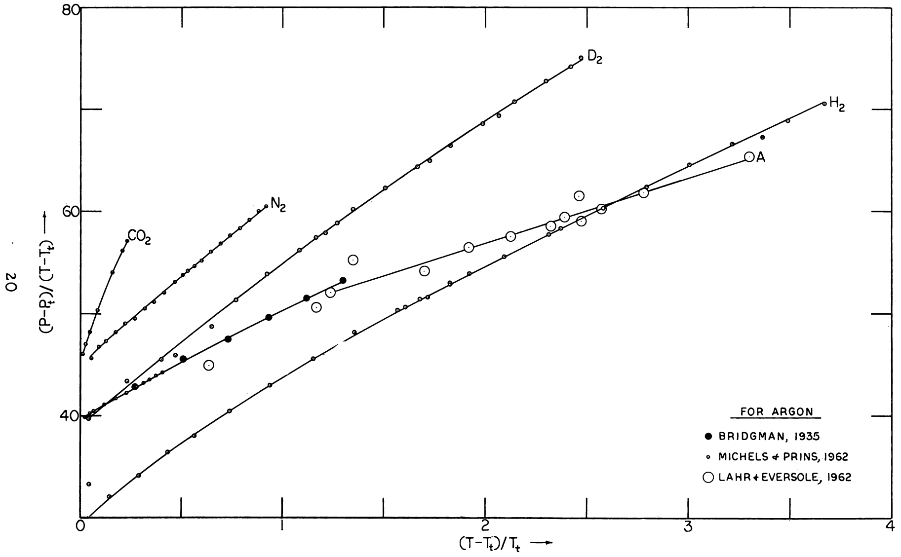
Figure 1. The function (P-P_t)/(T-T_t) vs. (T-T_t)/T_t .
