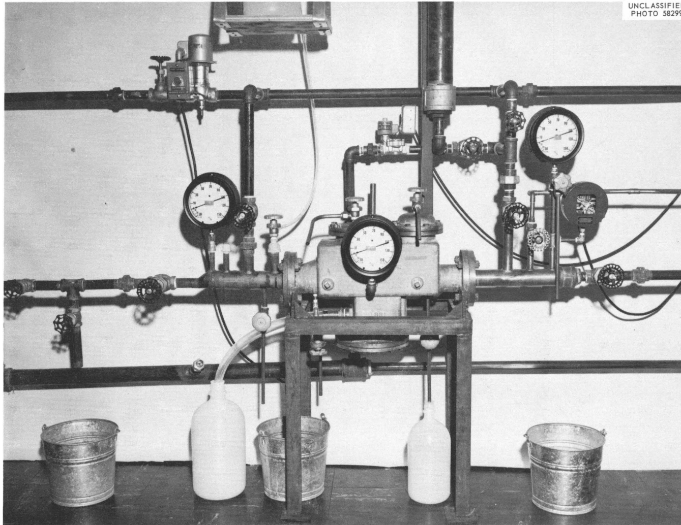
Backflow Preventer Test Installation, Closeup
