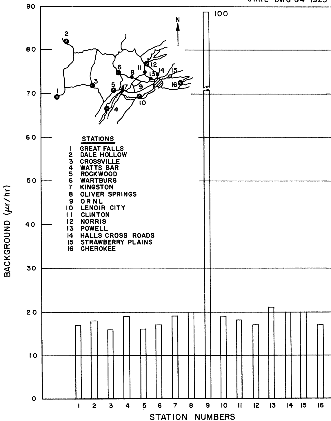
Fig. 10. Radiation Measurements Taken During 1963, 3 ft. Above the Ground Surface Out to Distances of 75 Miles from ORNL.
