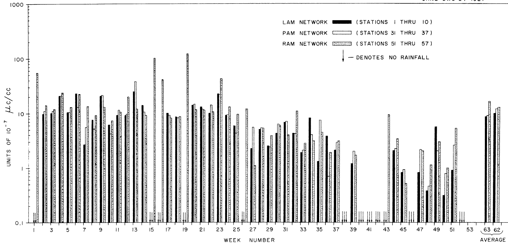
Fig. 8. Concentration of Radioactive Materials in Rainwater, 1963.
