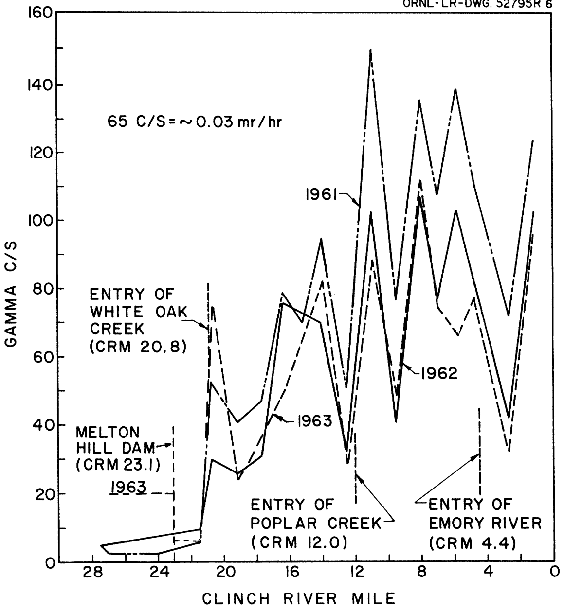
Fig. 12. Gamma Count at Surface of Clinch River Silt.
