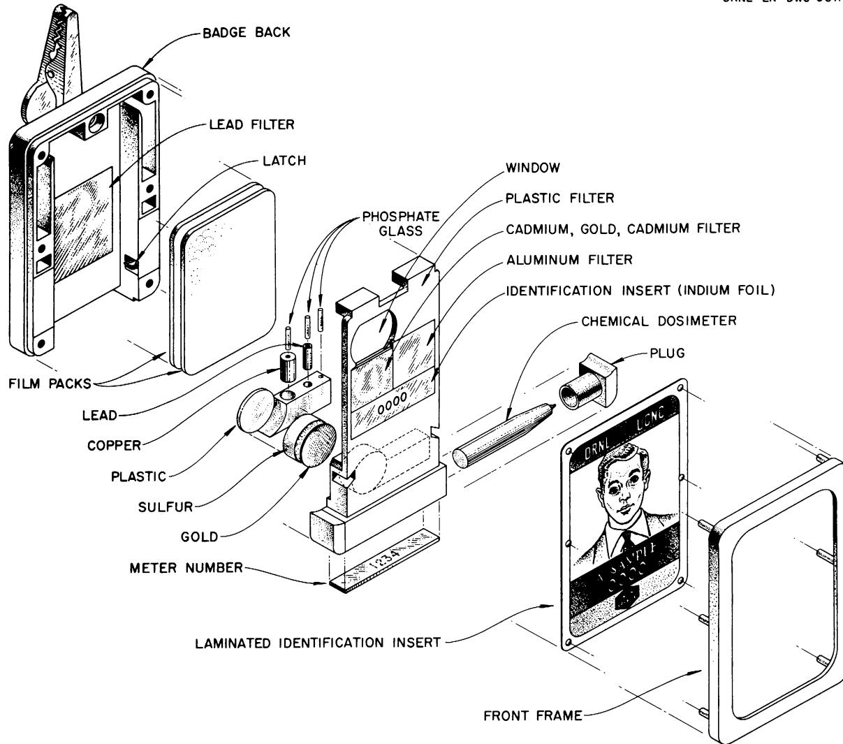
Fig. 15. ORNL Badge-Meter, Model II.
