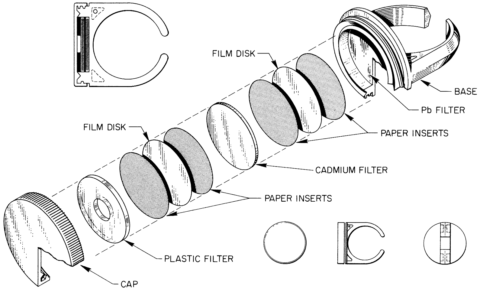
Fig. 18. Details of the ORNL Hand Exposure Meter.
