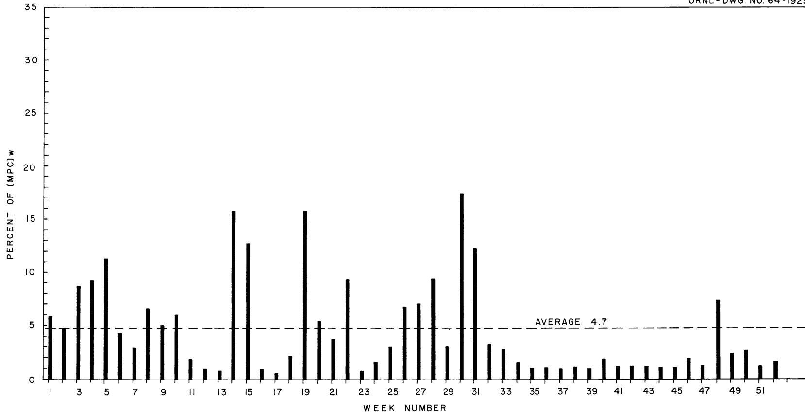
Fig. 9. Estimated Per Cent (MPC)w of Radioactivity in Clinch River Water Below the Mouth of White Oak Creek, 1963.
