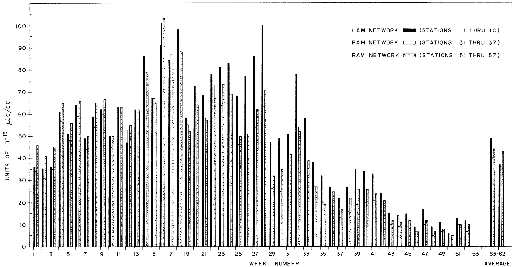
Fig. 6. Concentration of Radioactive Materials in Air as Determined from Filter Paper Data, 1963.
