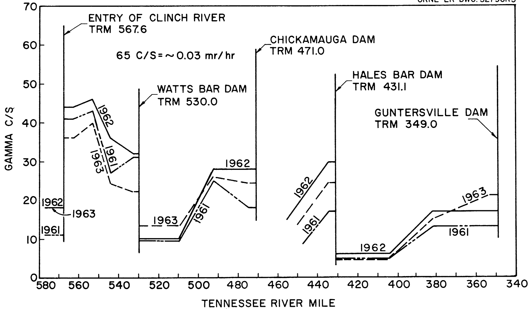
Fig. 13. Gamma Count at Surface of Tennessee River Silt.
