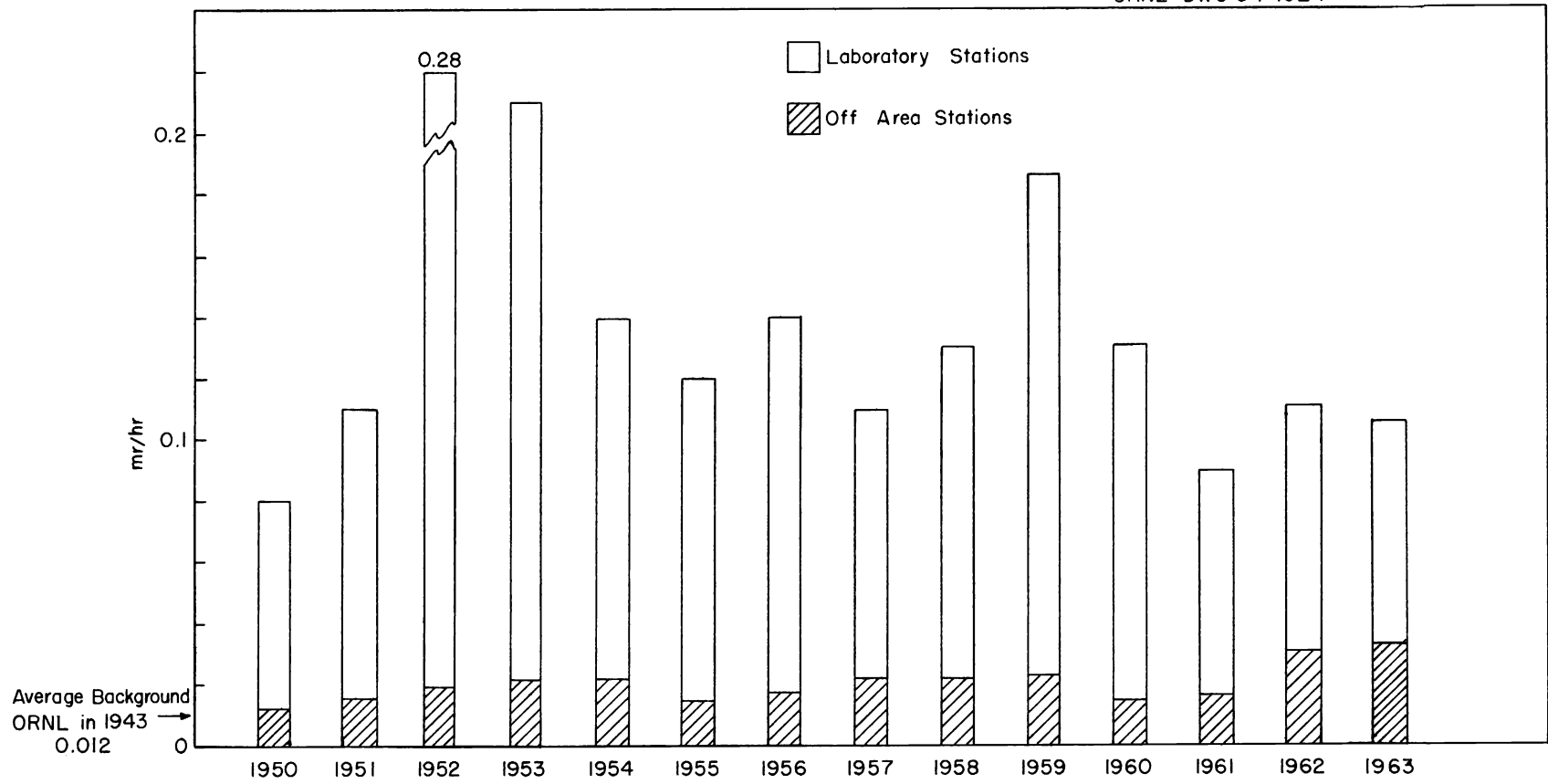
Fig. 11. Radiation Measurements Taken 3 ft. Above the Ground Surfaces at ORNL Compared with Like Measurements Taken Elsewhere within the AEC Controlled Area for the Years 1950-1963.
