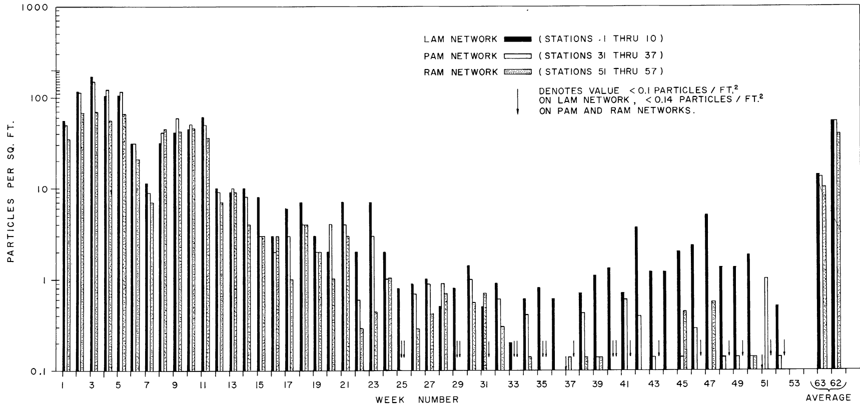
Fig. 7. Radioparticulate Fall-Out Measurements as Determined by Autoradiographic Techniques Using Gummed Paper Collectors, 1963.
