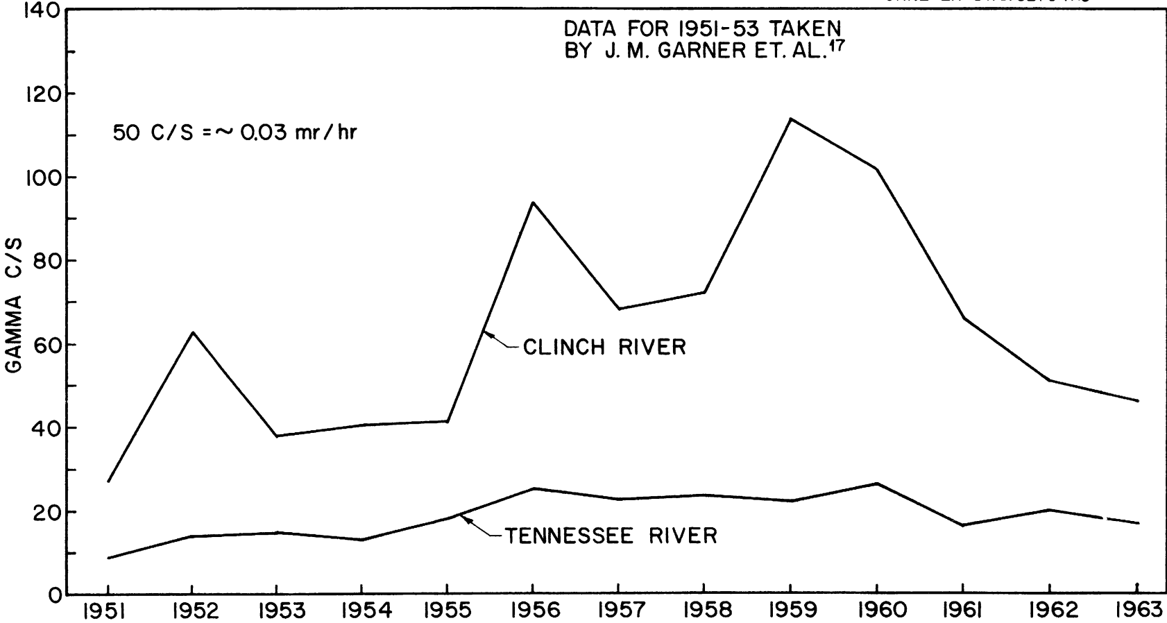
Fig. 14. Average Gamma Count at Surface of Silt Clinch and Tennessee Rivers, 1951-63.
